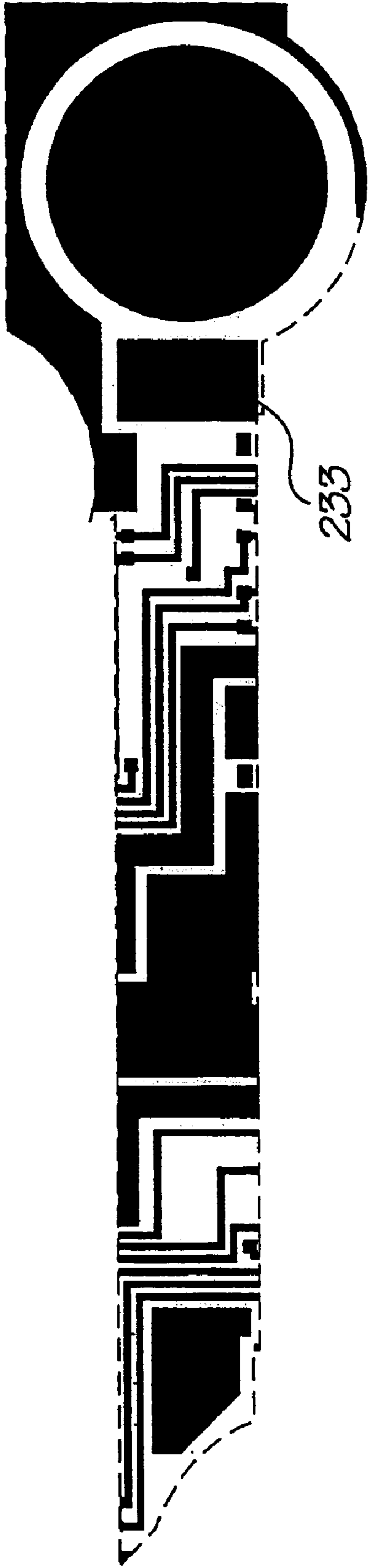
Metal 2 mask
