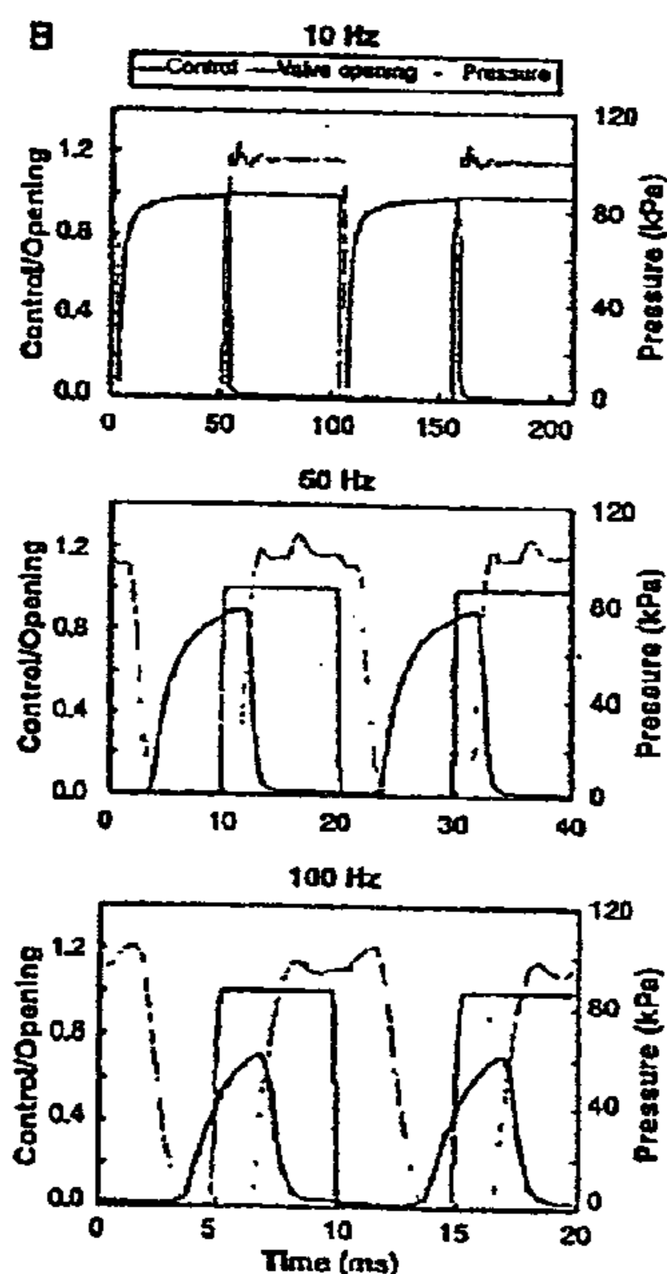
Fig. 3. (A) Valve opening versus applied pressure. "50 \times 100" indicates a microvalve with a 50- \mu\text{m} -wide control channel and a 100- \mu\text{m} -wide fluid channel. 100 \times 50 closing and opening data (not shown) are nearly identical to 50 \times 100 data. (B) Time response of a 100 \mu\text{m} by 100 \mu\text{m} by 10 \mu\text{m} RTV microvalve with 10-cm-long air tubing connected from the chip to a pneumatic valve. Two periods of digital control signal, actual air pressure at the end of the tubing, and valve opening are shown here. The pressure applied on the control line is 100 kPa, which is substantially higher than the \sim 40 kPa required to close the valve. Thus, when closing, the valve is pushed closed with a pressure 60 kPa greater than required. When opening, however, the valve is driven back to its rest position only by its own spring force ( \leq 40 kPa). Thus, \tau_{\text{close}} is expected to be smaller than \tau_{\text{open}} . There is also a lag between the control signal and control pressure response, due to the limitations of the miniature valve used to control the pressure. Calling such lags t and the 1/e time constants \tau , the values are t_{\text{open}} = 3.63 ms, \tau_{\text{open}} = 1.88 ms, t_{\text{close}} = 2.15 ms, and \tau_{\text{close}} = 0.51 ms. If 3\tau each are allowed for opening and closing, the valve runs comfortably at 75 Hz when filled with aqueous solution (36). Valve opening was measured by fluorescence. The flow channel was filled with a solution of fluorescein isothiocyanate in buffer (pH \geq 8 ), and the fluorescence of a square area occupying the center third of the channel was monitored on an epi-fluorescence microscope with a photomultiplier tube with a 10-kHz bandwidth. The pressure was monitored with a Wheatstone-bridge pressure sensor (SCC15GD2; Sensym, Milpitas, California) pressurized simultaneously with the control line through nearly identical pneumatic connections.
