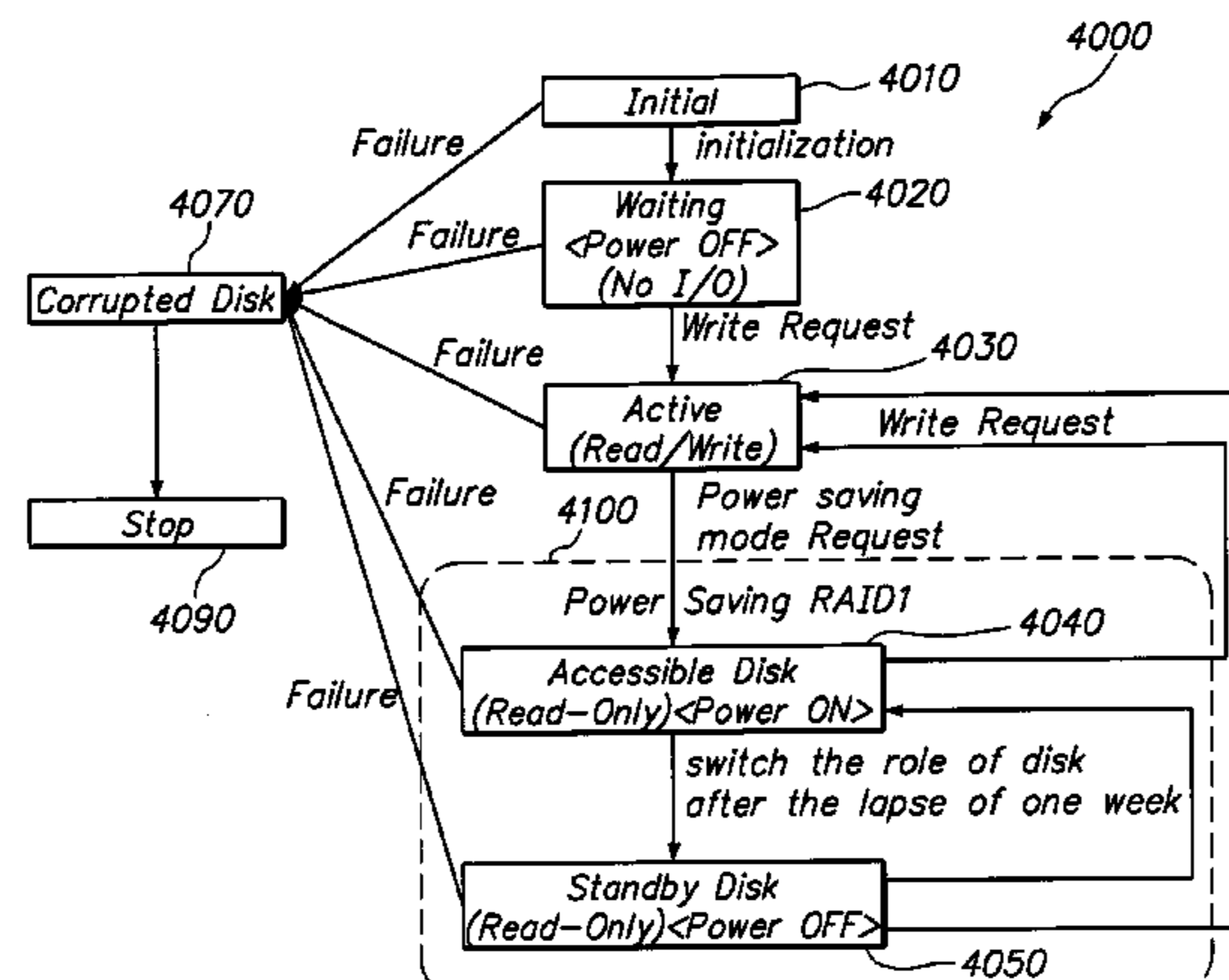
State Transition Diagram (default)
