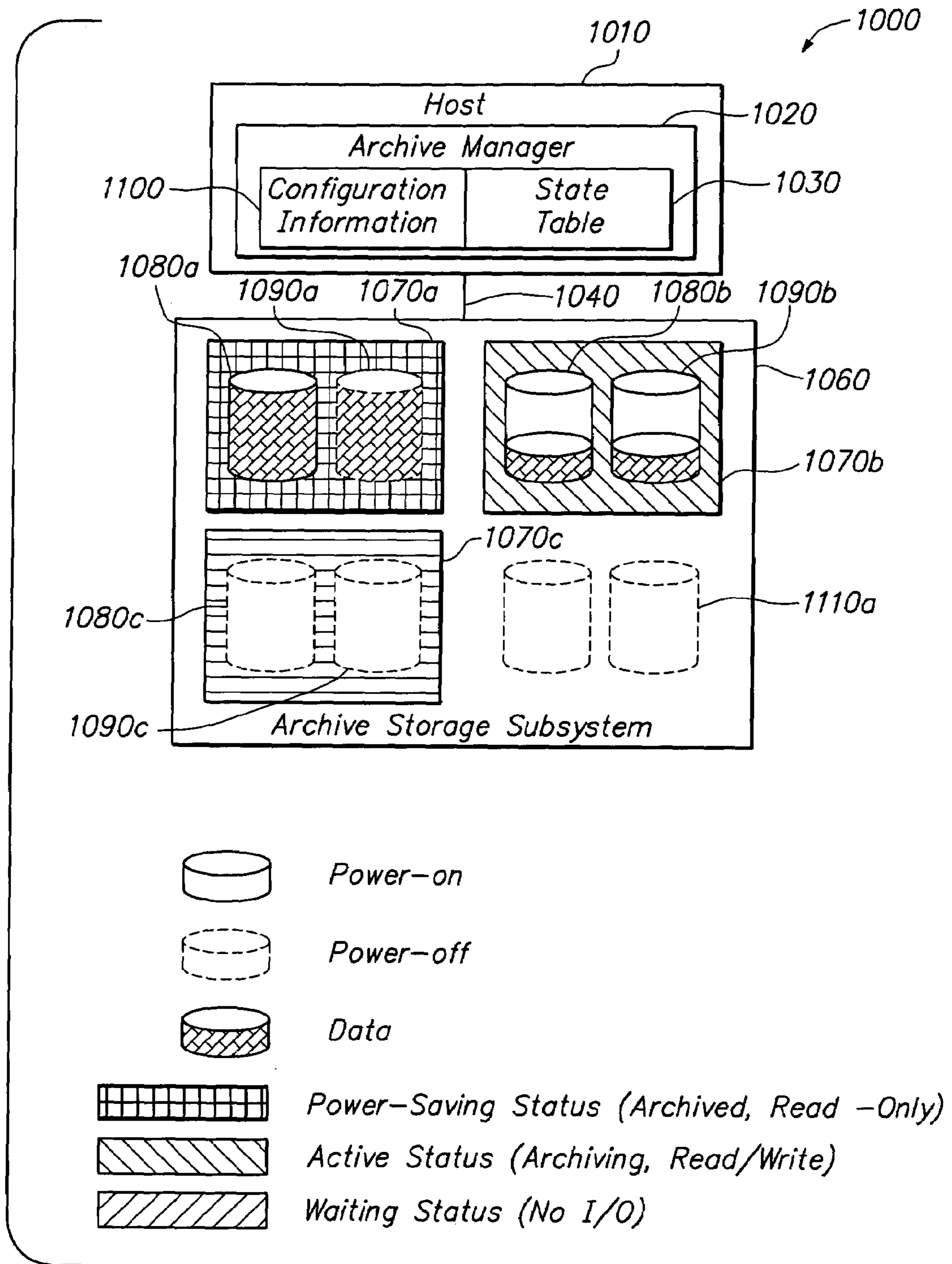
FIG. 3 Status of RAID1
