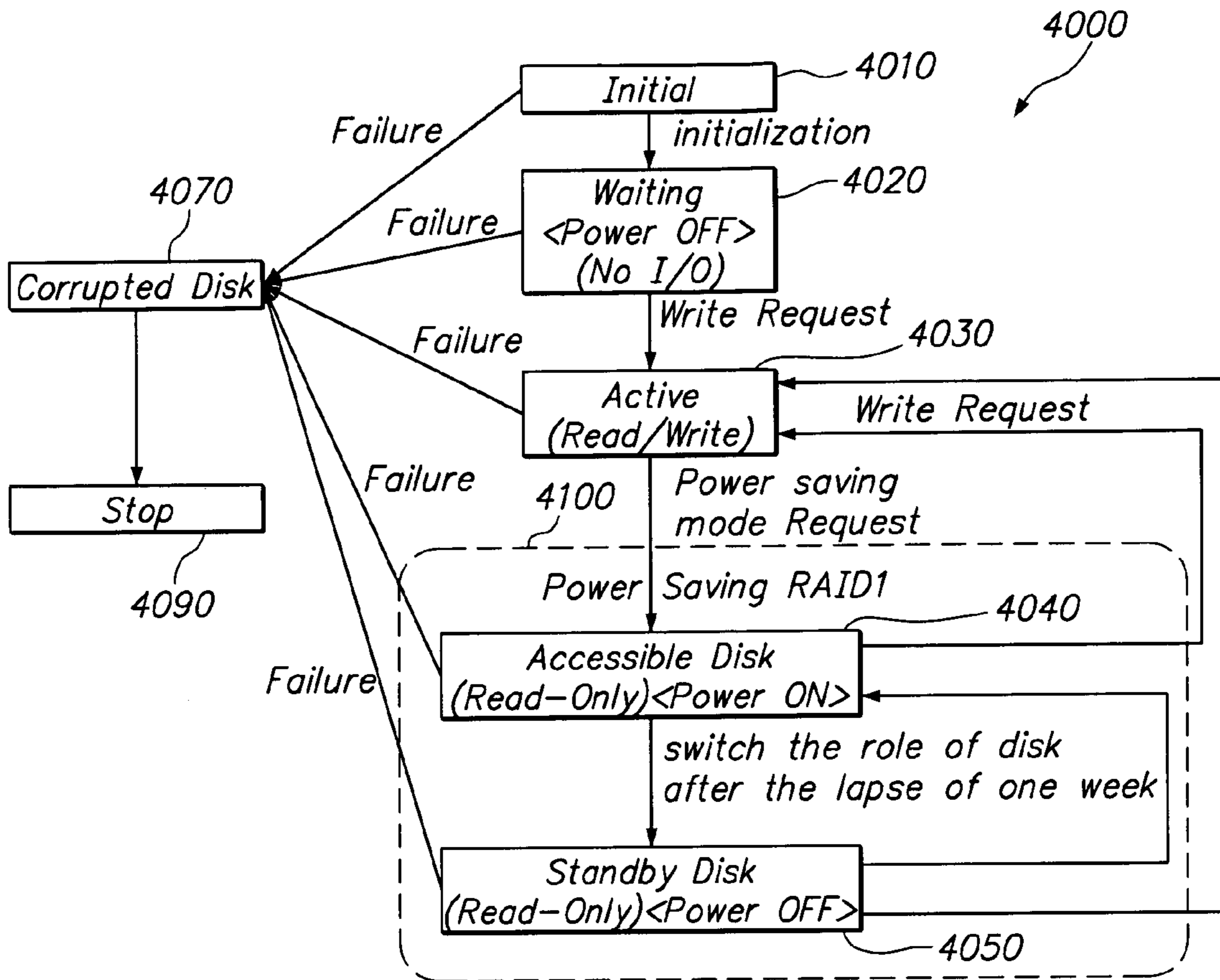
FIG. 6 State Transition Diagram (default)
