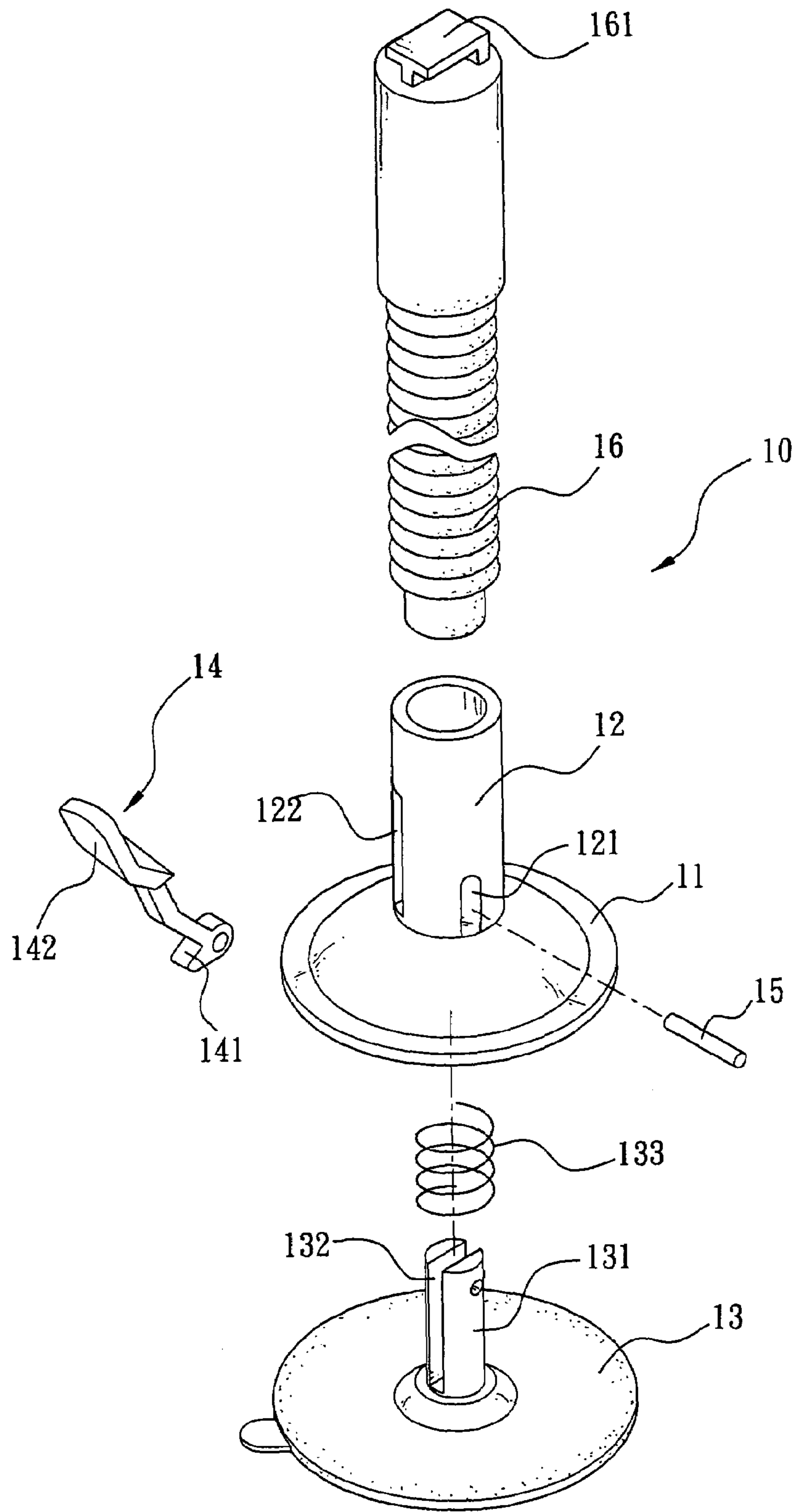
FIG. 1 (Prior Art)
