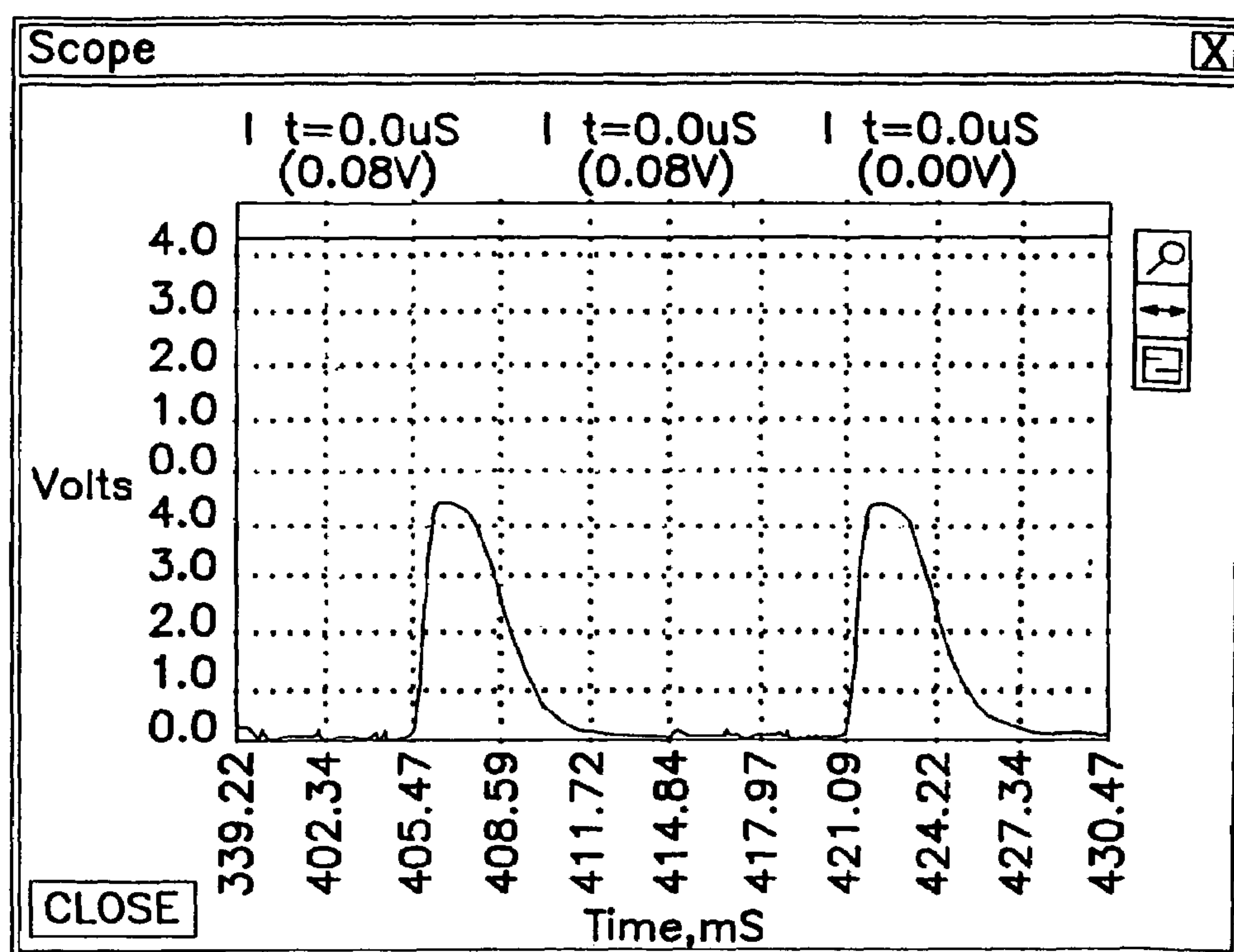
CRT photoresponse
