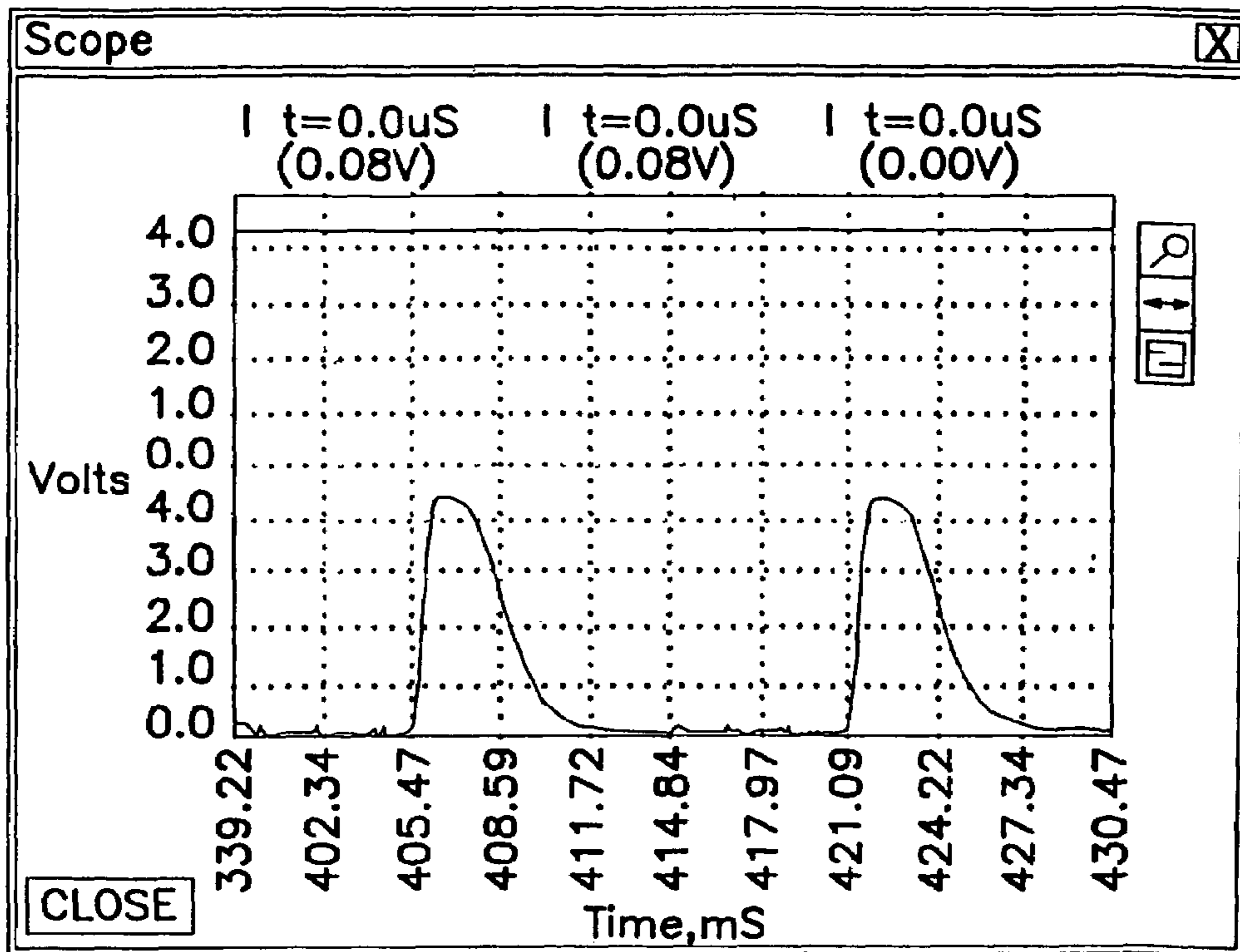
CRT photoresponse
