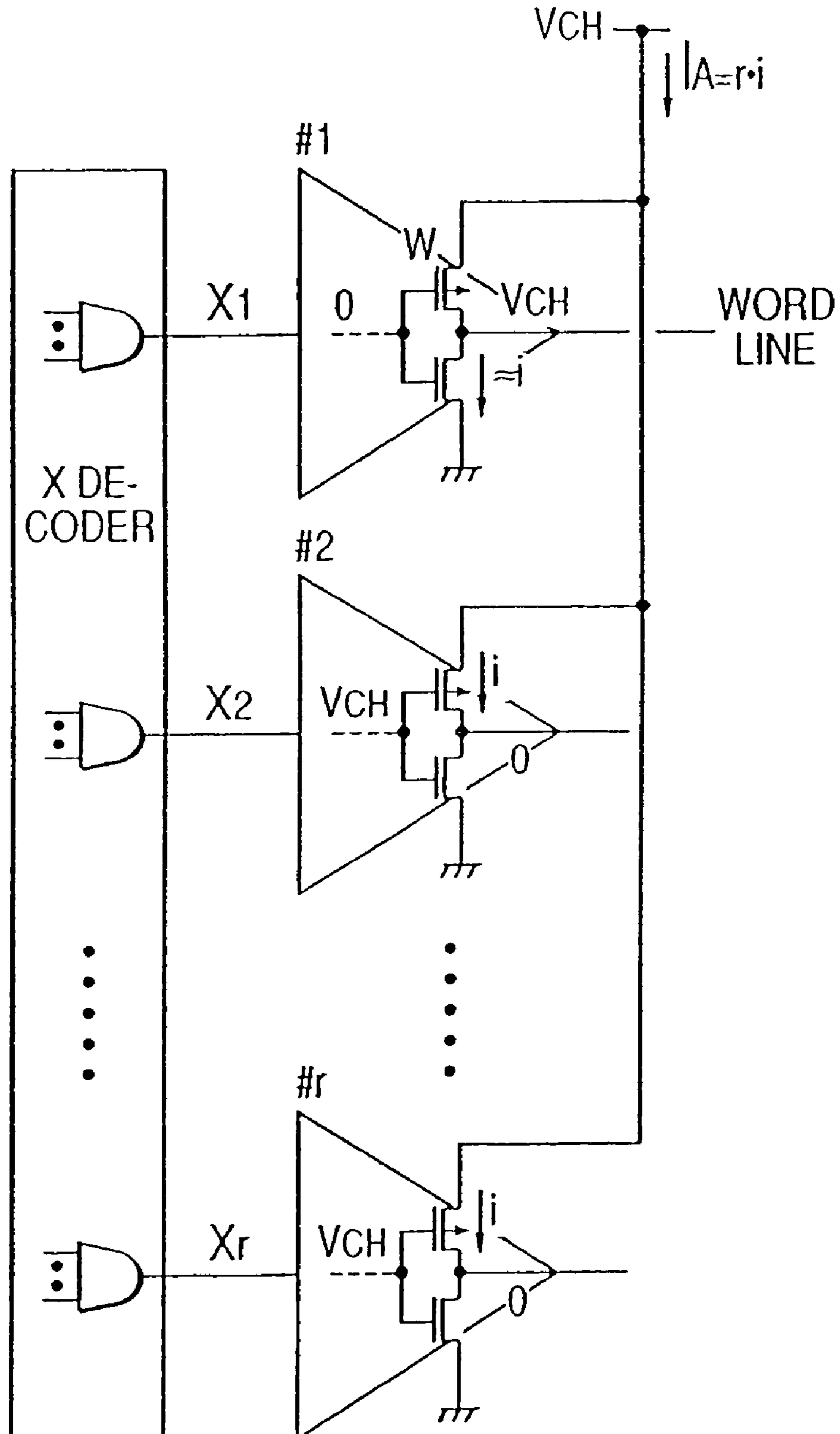
FIG. 24 PRIOR ART
