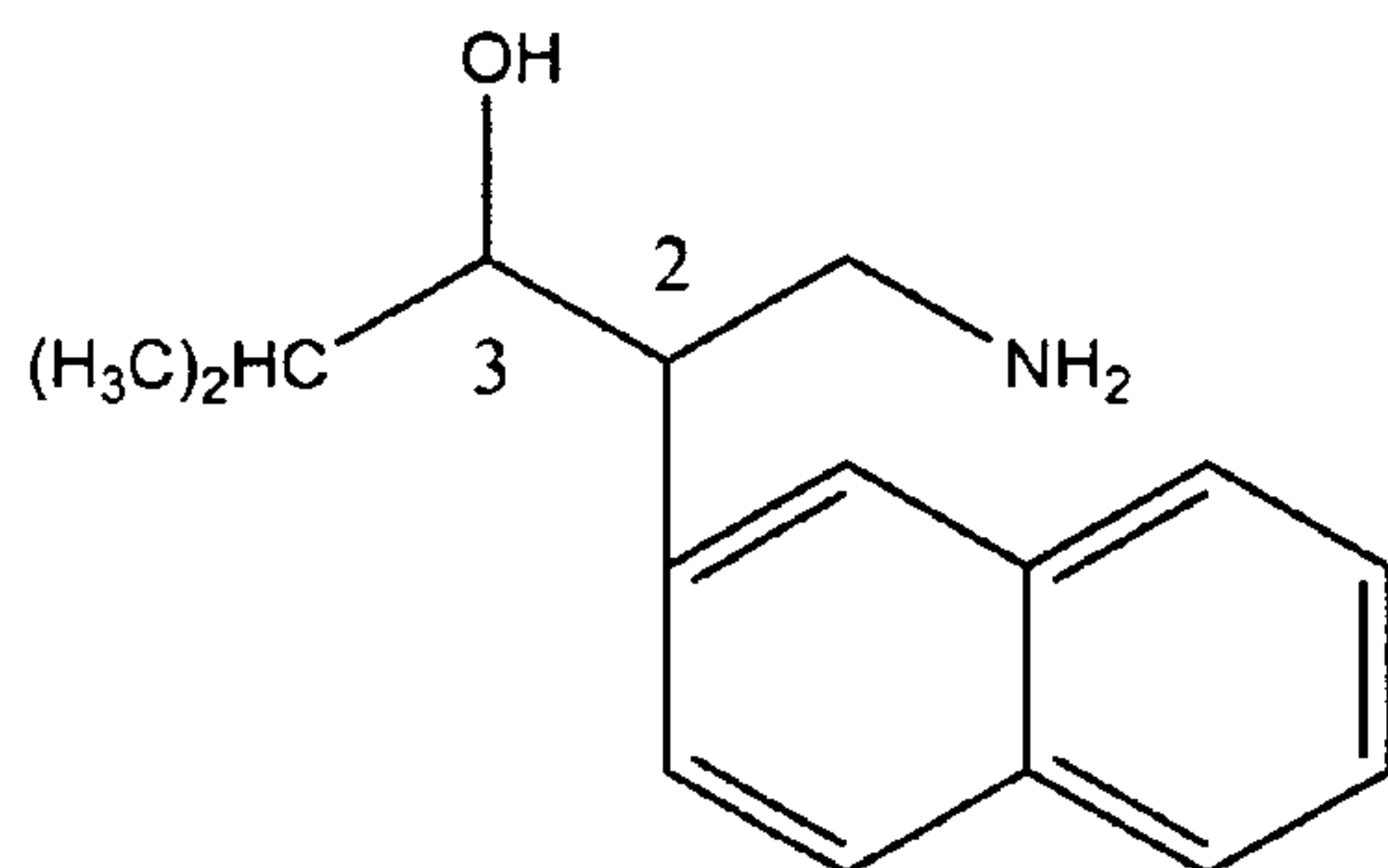
3-hydroxy-4-methyl-2-(2'-naphthyl)pentylamine
