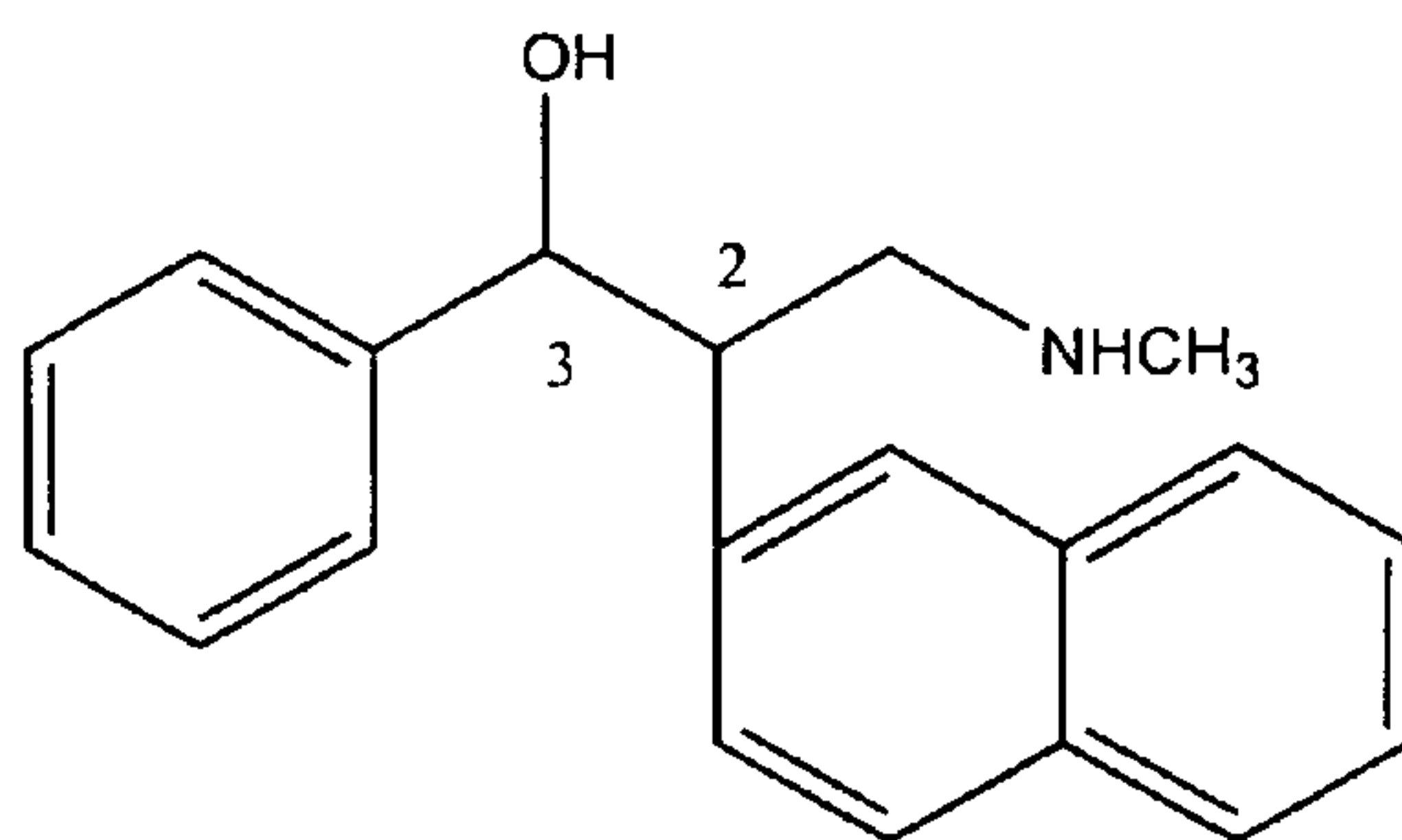
N -methyl-3-hydroxy-2-(2'-naphthyl)-3-phenylpropylamine
