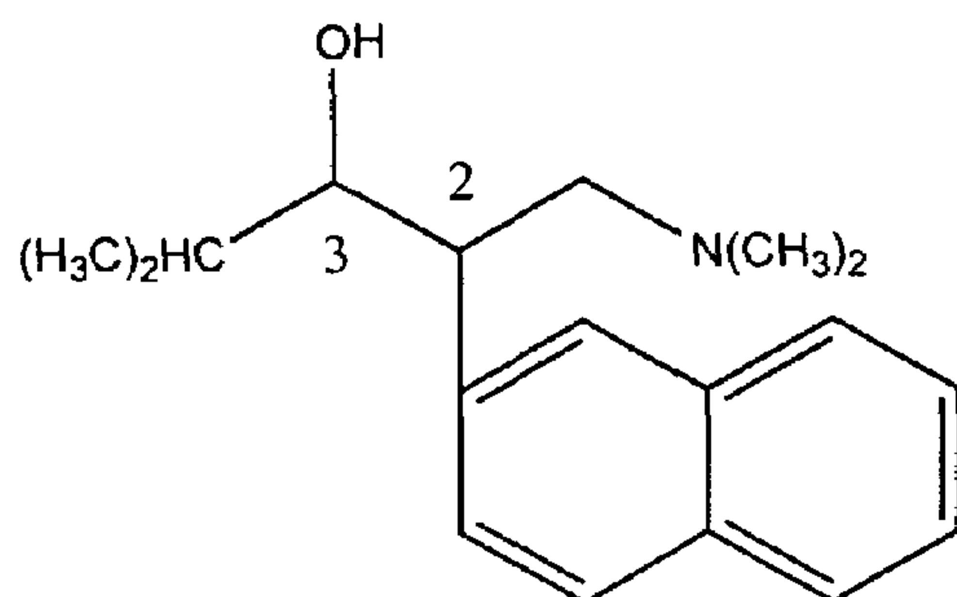
N,N -dimethyl-3-hydroxy-4-methyl-2-(2'-naphthyl)pentylamine
