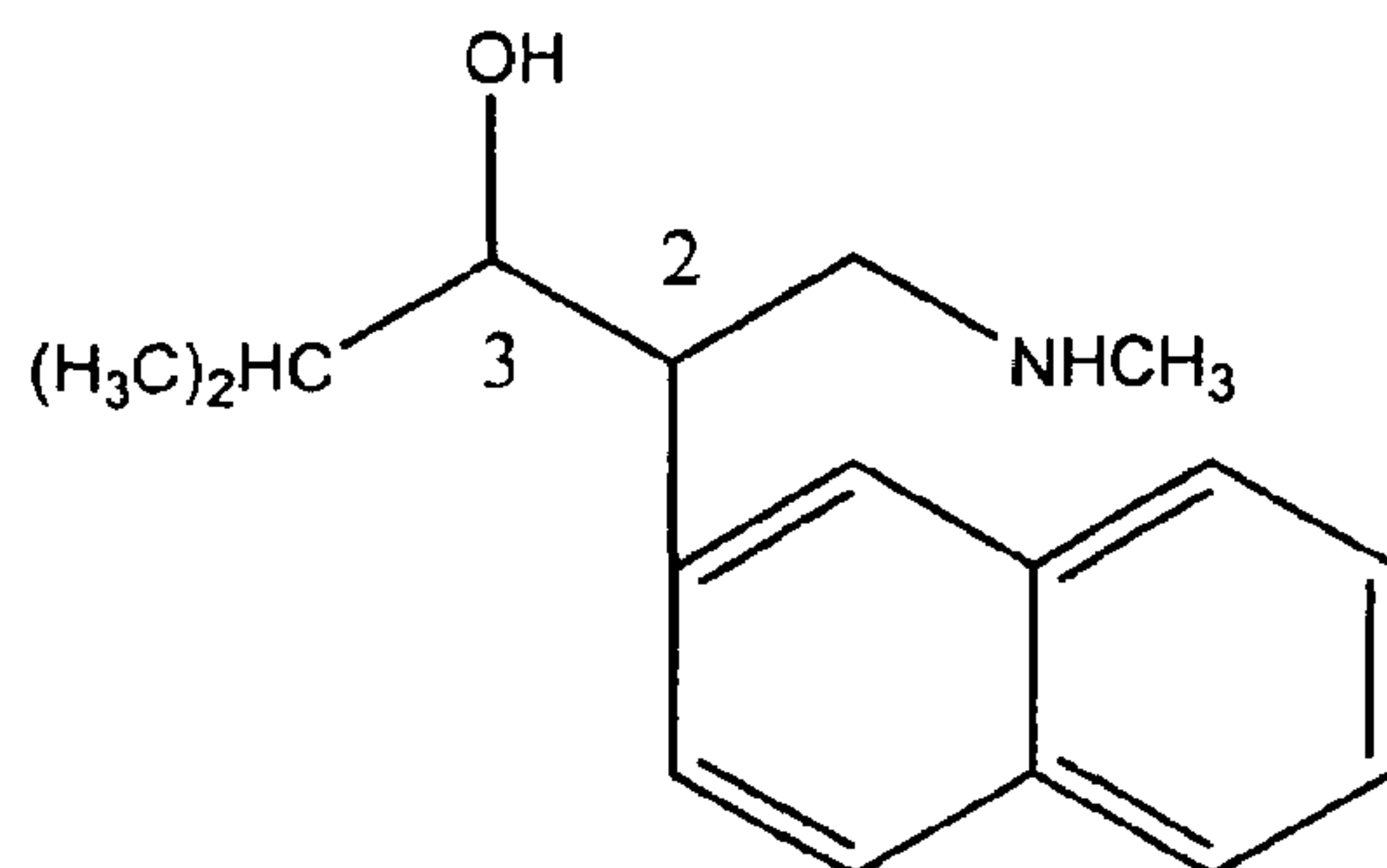
N -methyl-3-hydroxy-4-methyl-2-(2'-naphthyl)pentylamine
