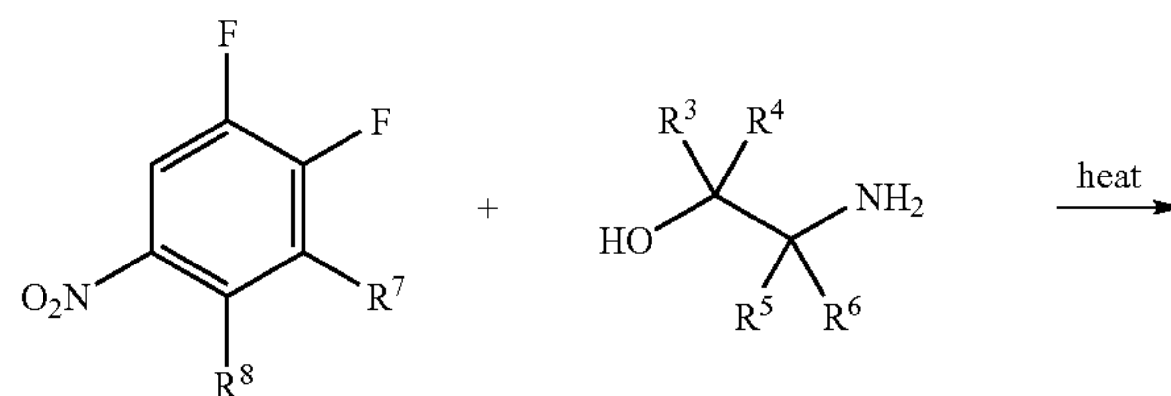
Scheme V
