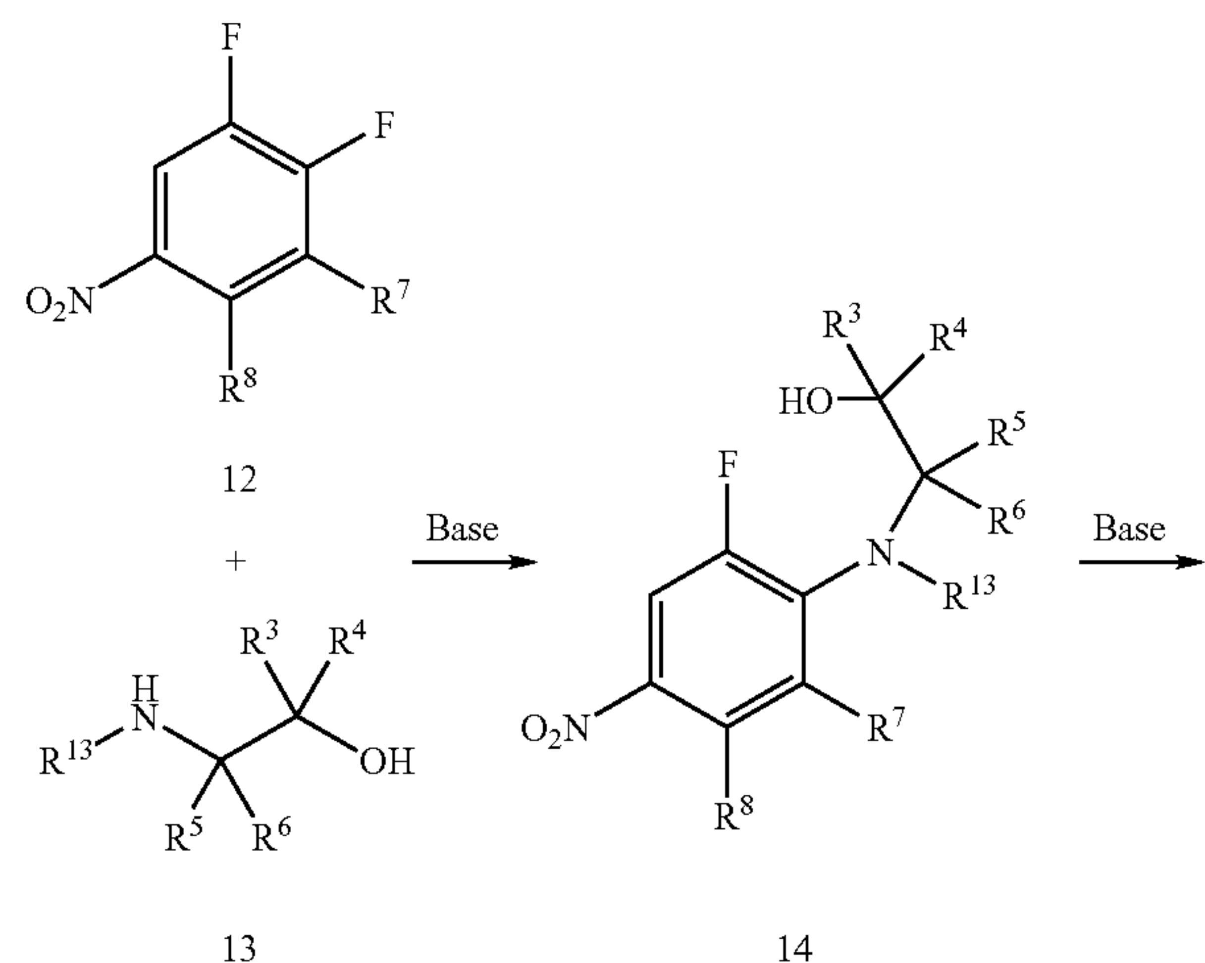
Scheme III
