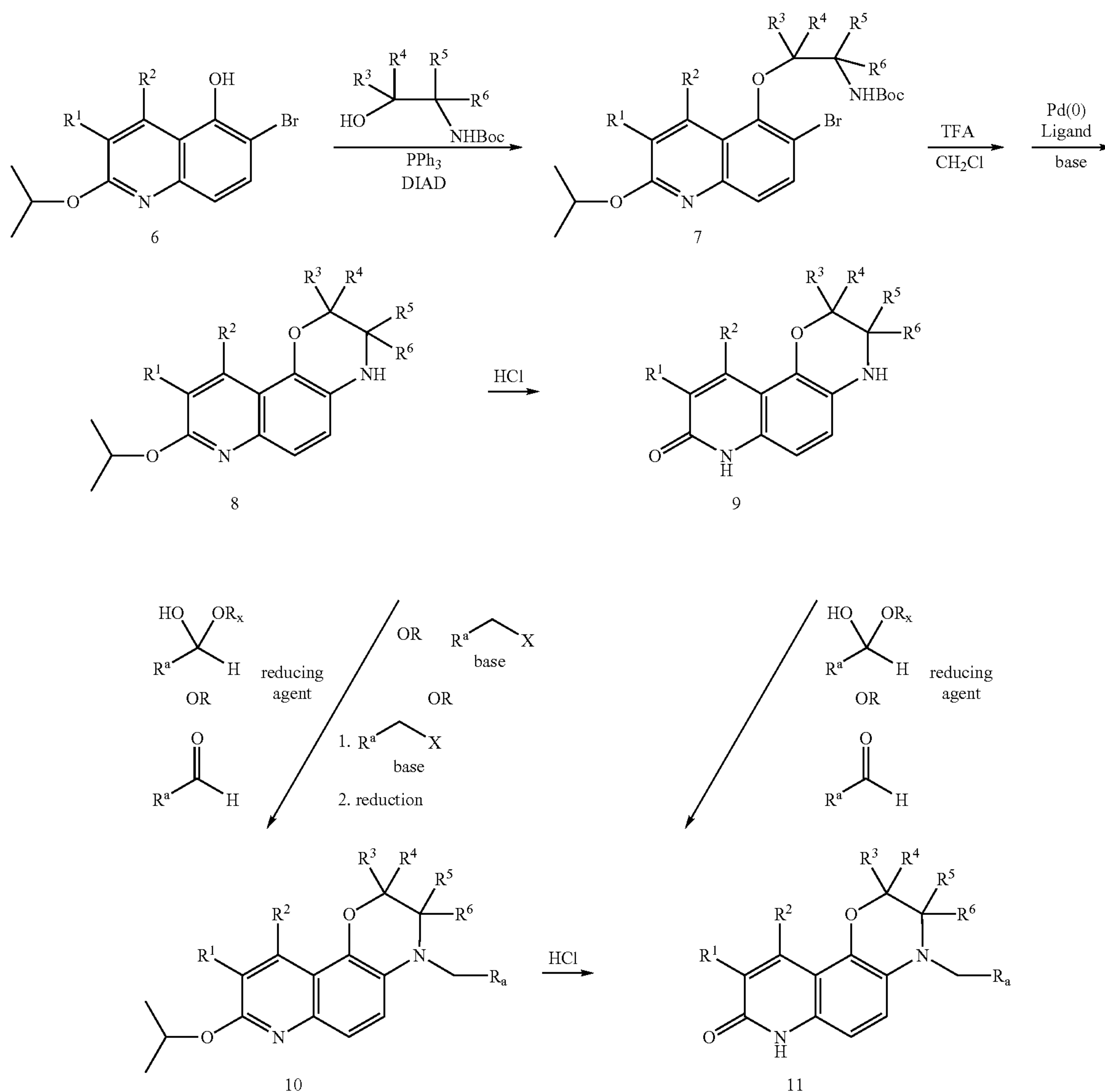
Scheme II
