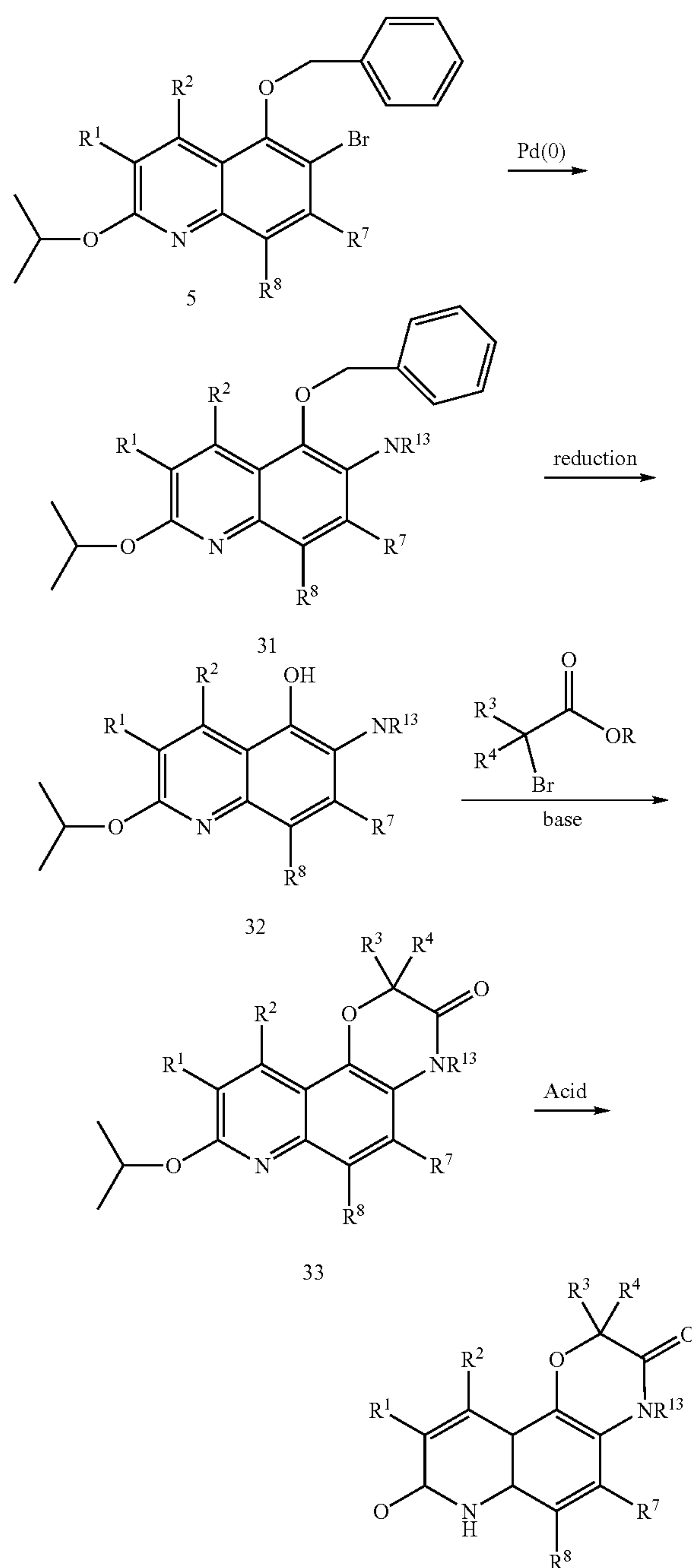
Scheme VII
