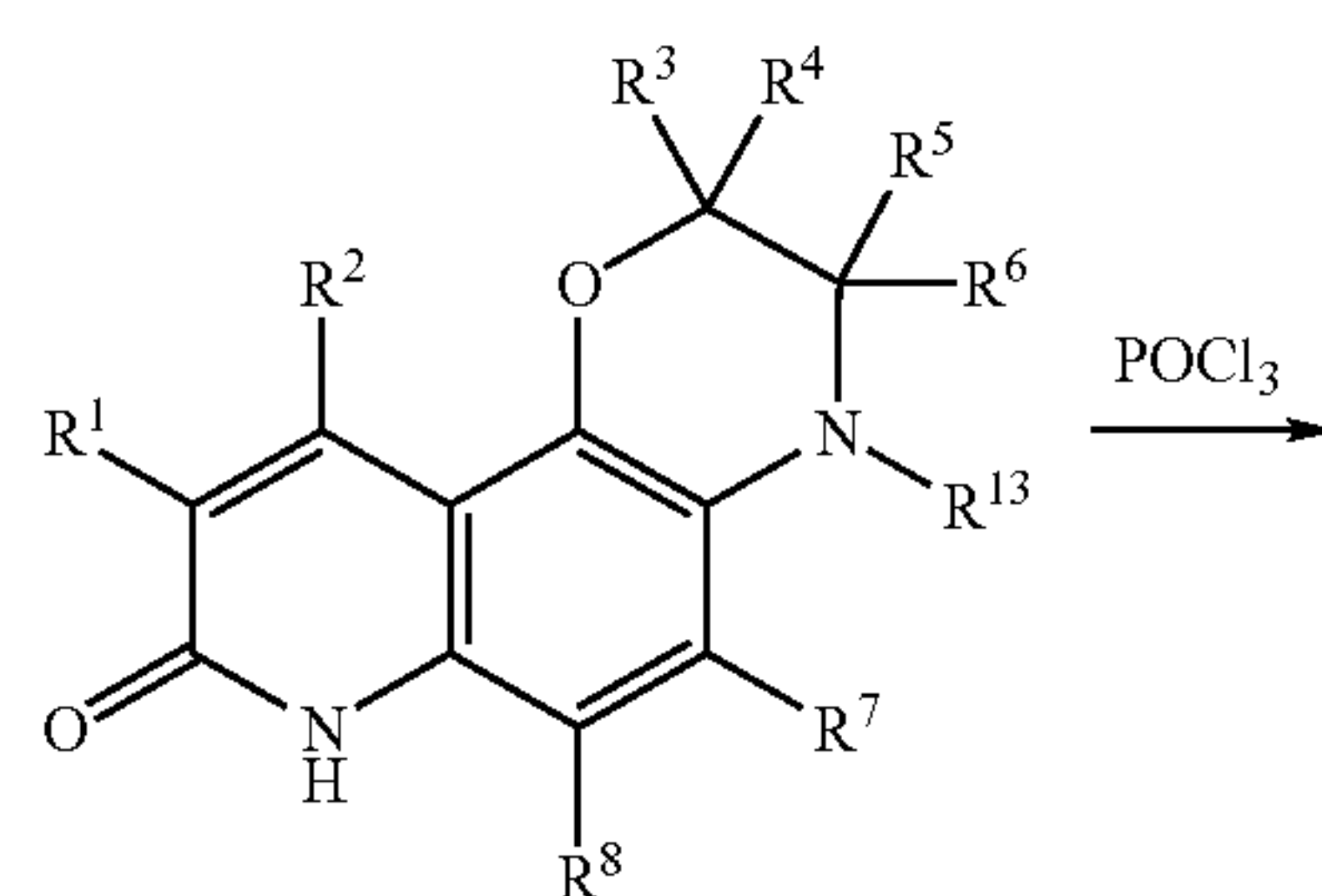
Scheme IV
