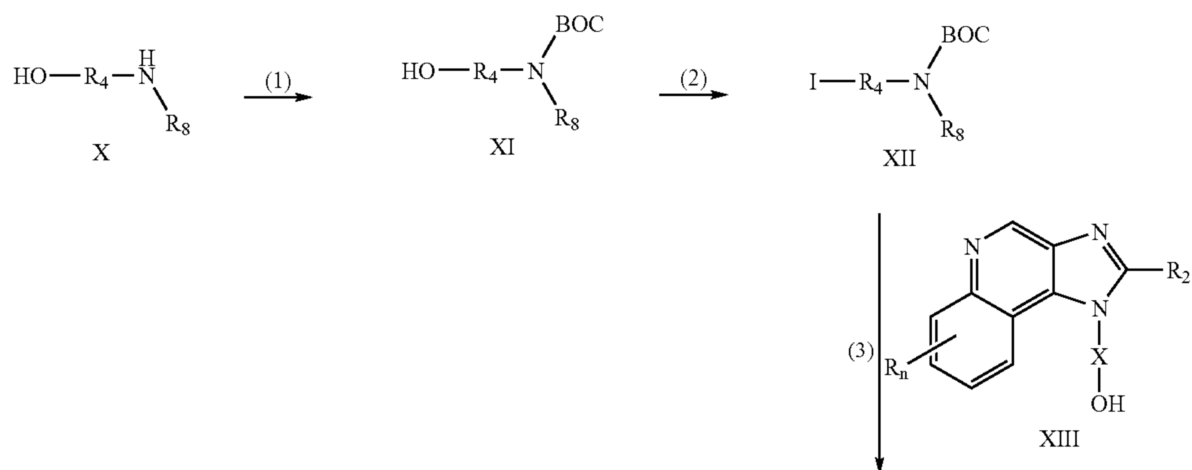
Reaction Scheme I
