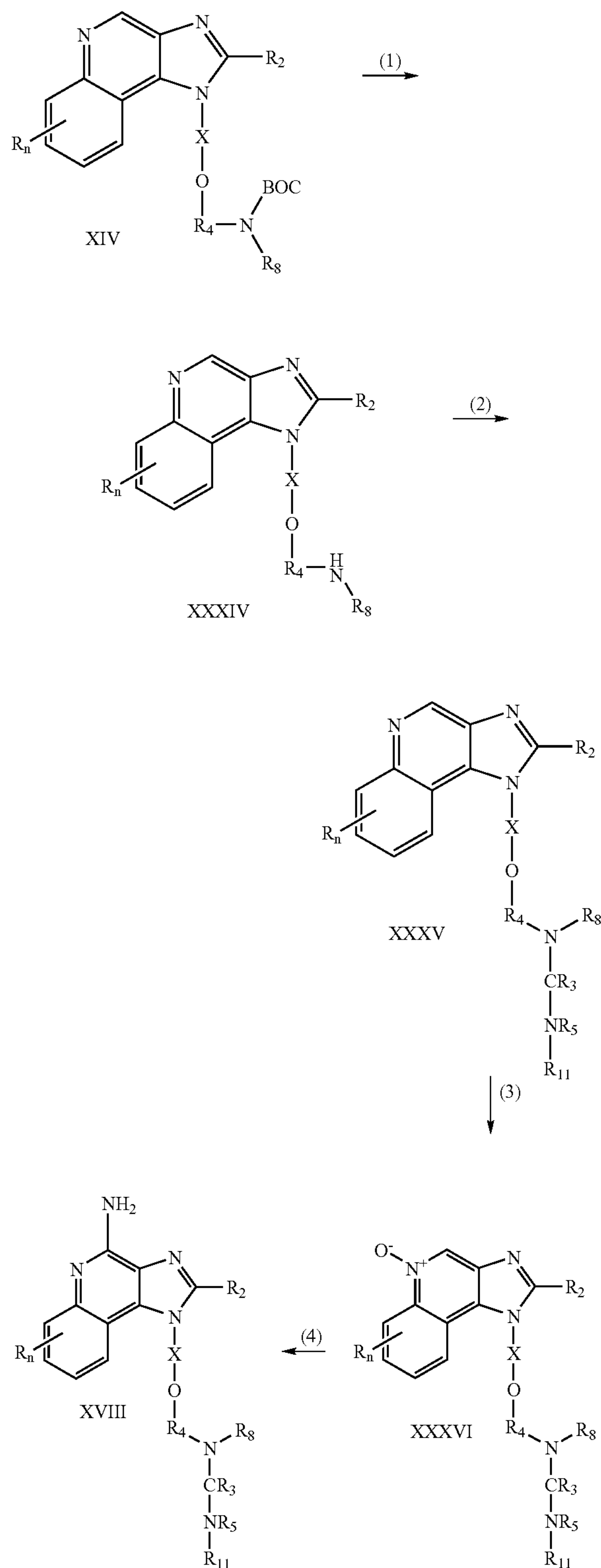
Reaction Scheme V
