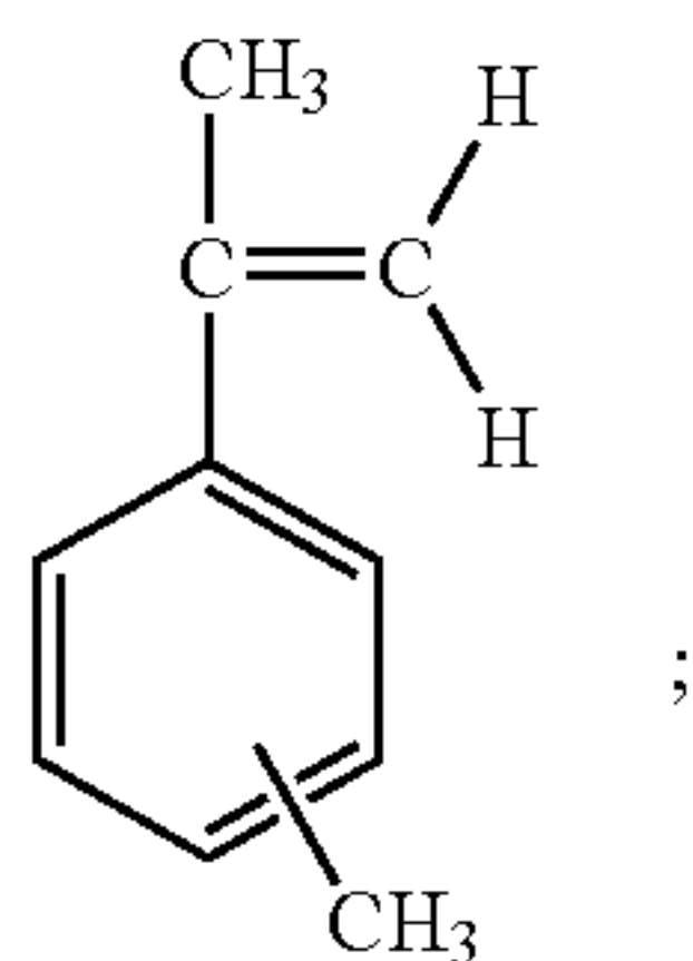
Isopropenyltoluene
