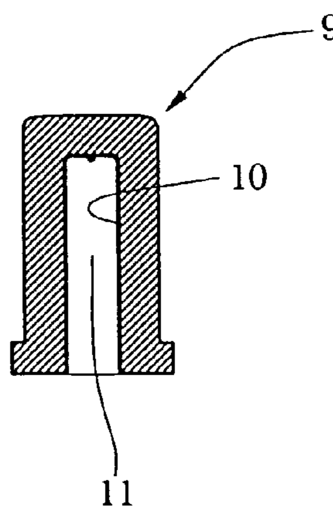
Fig.2C (PRIOR ART)
