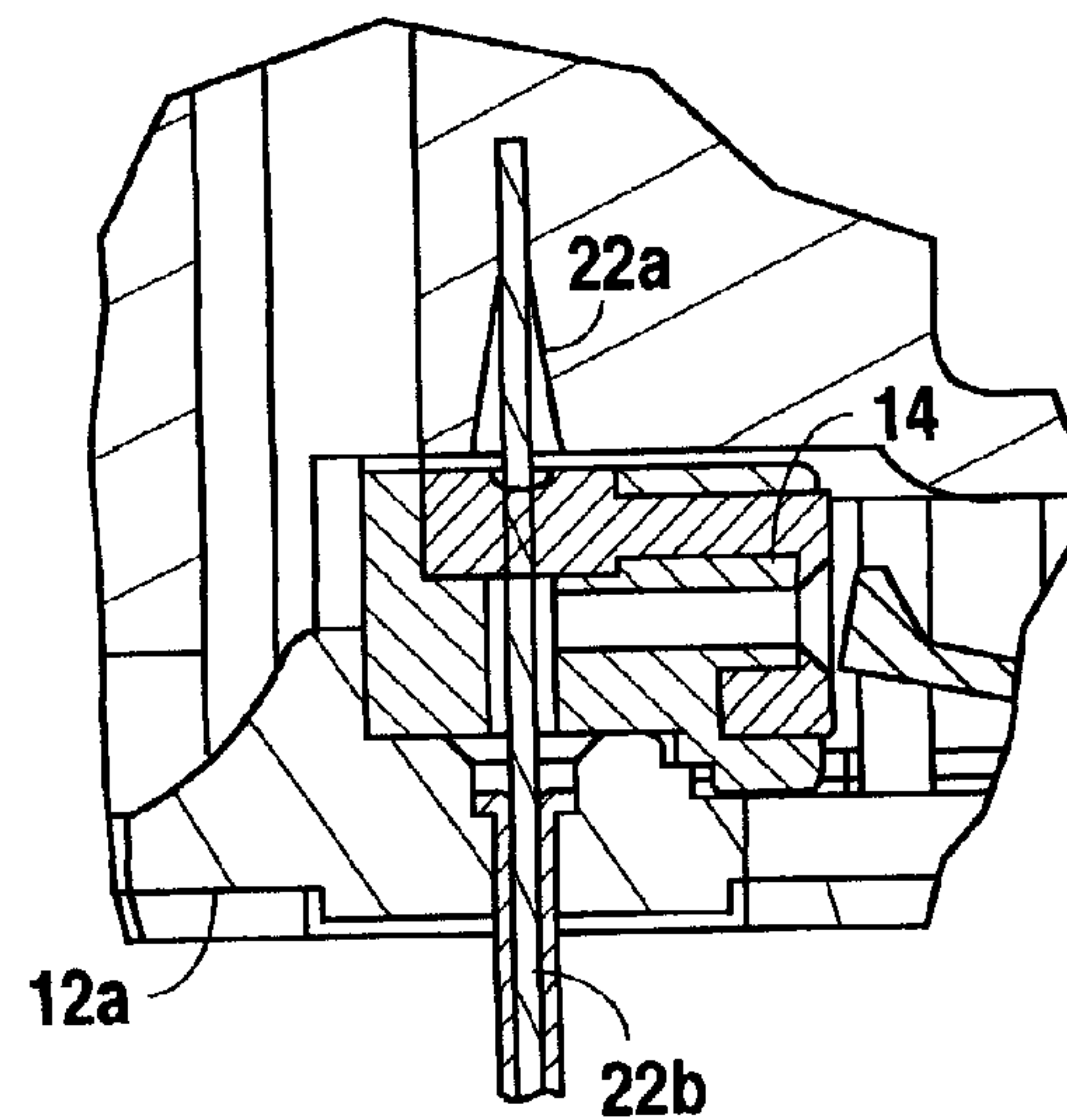
Fig. 3C ( DETAIL B )
