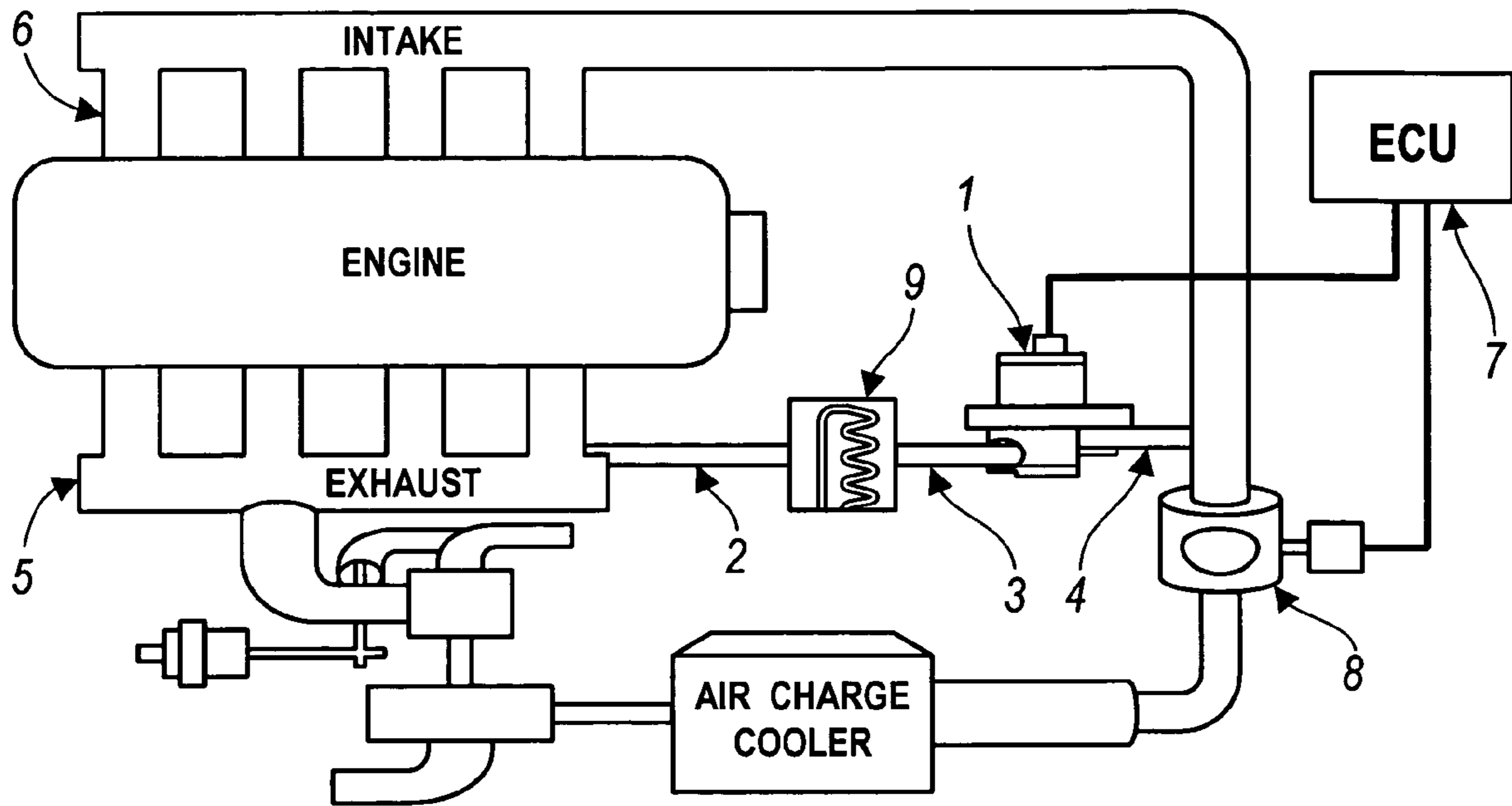
FIG. 1 (prior art)
