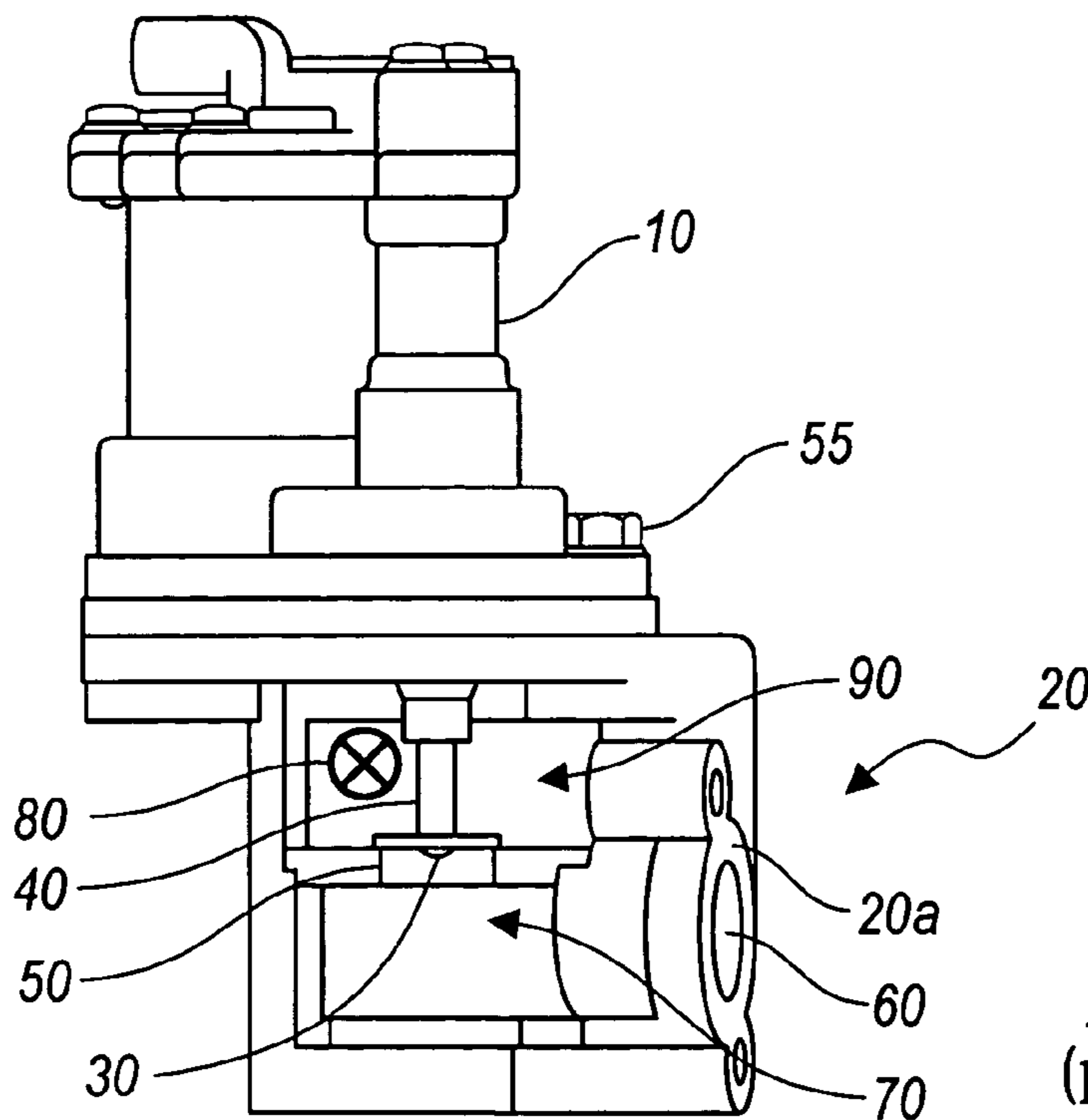
FIG. 1 (prior art)
