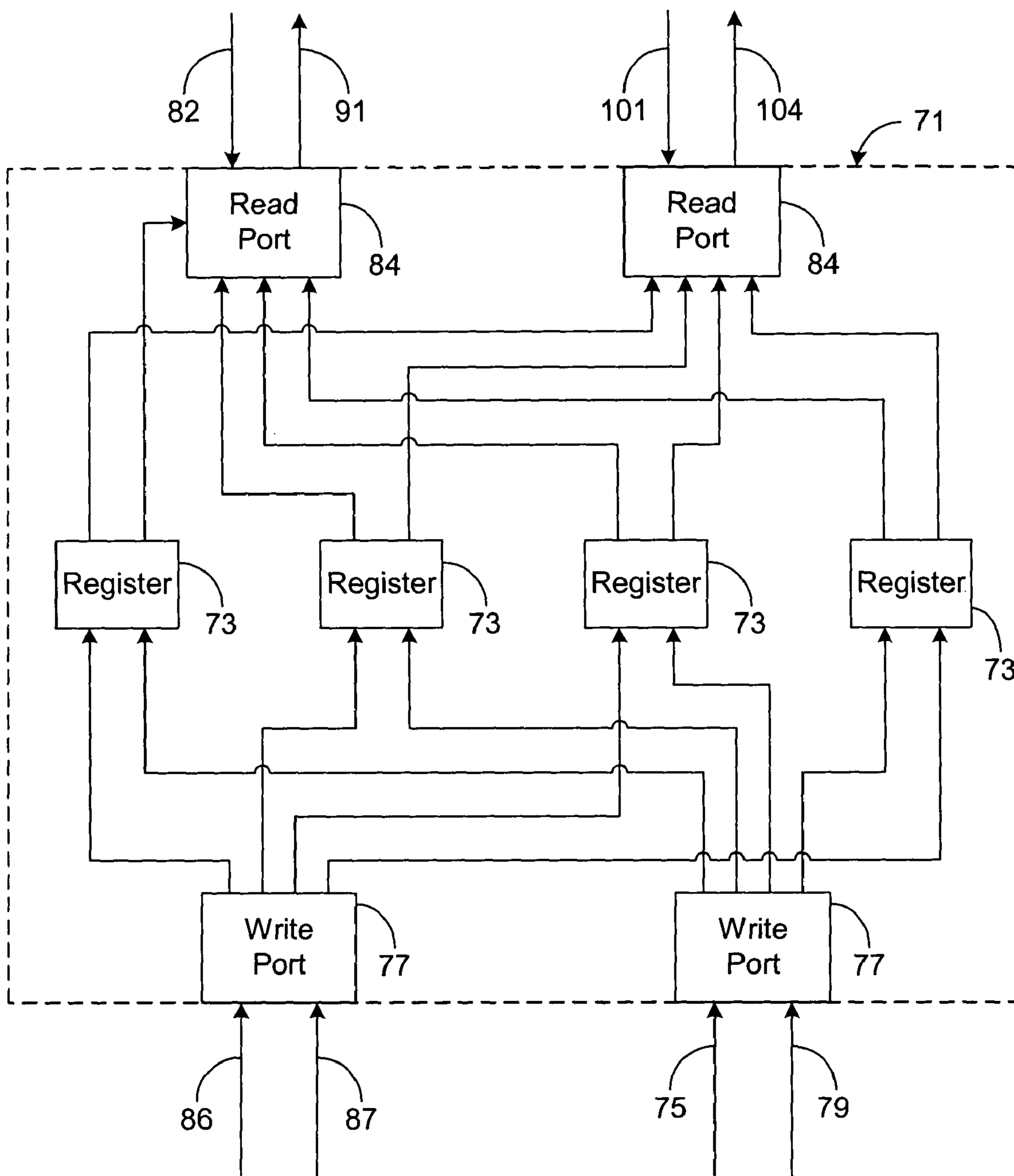
FIG. 3 (Prior Art)
