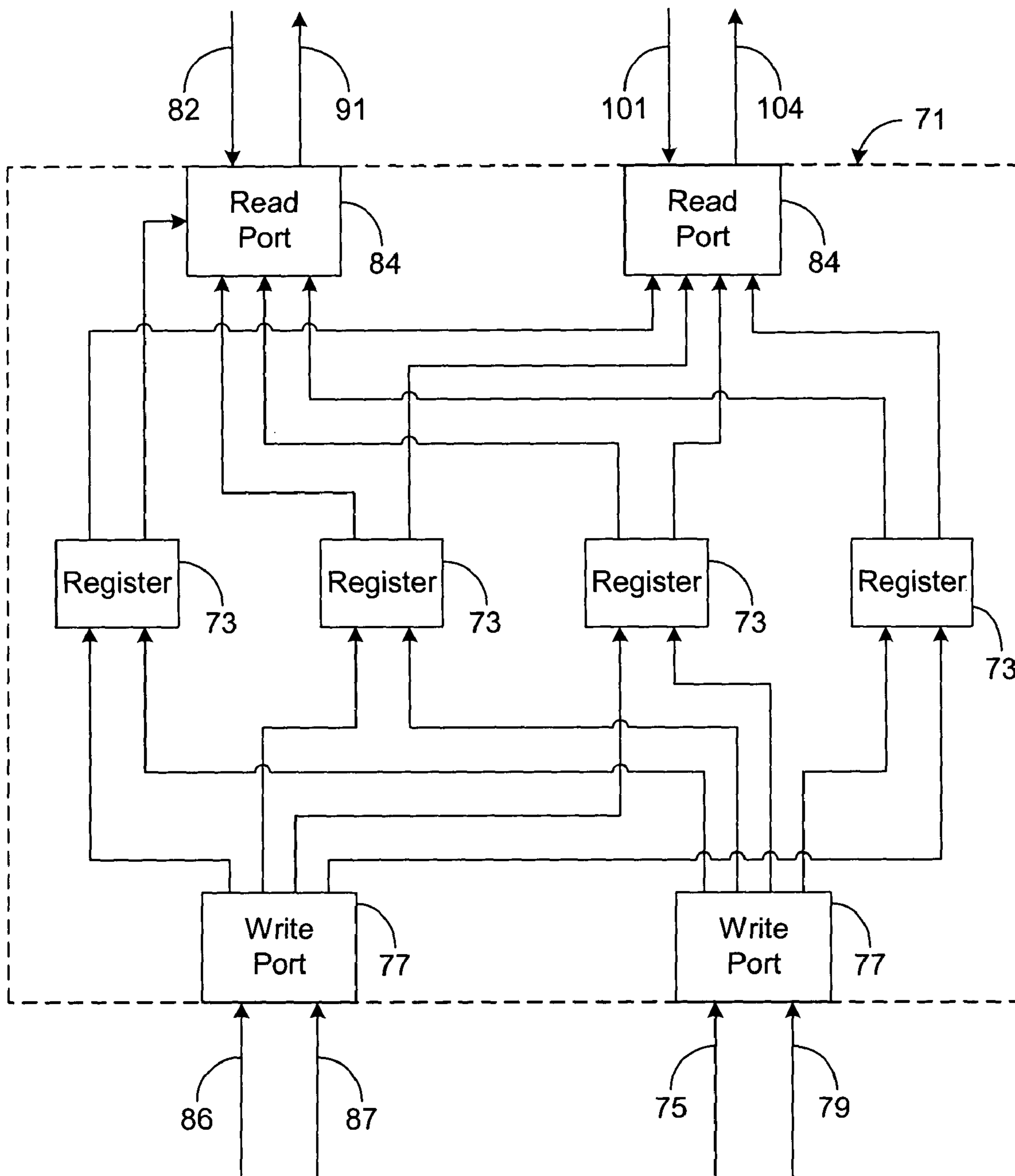
FIG. 3 (Prior Art)
