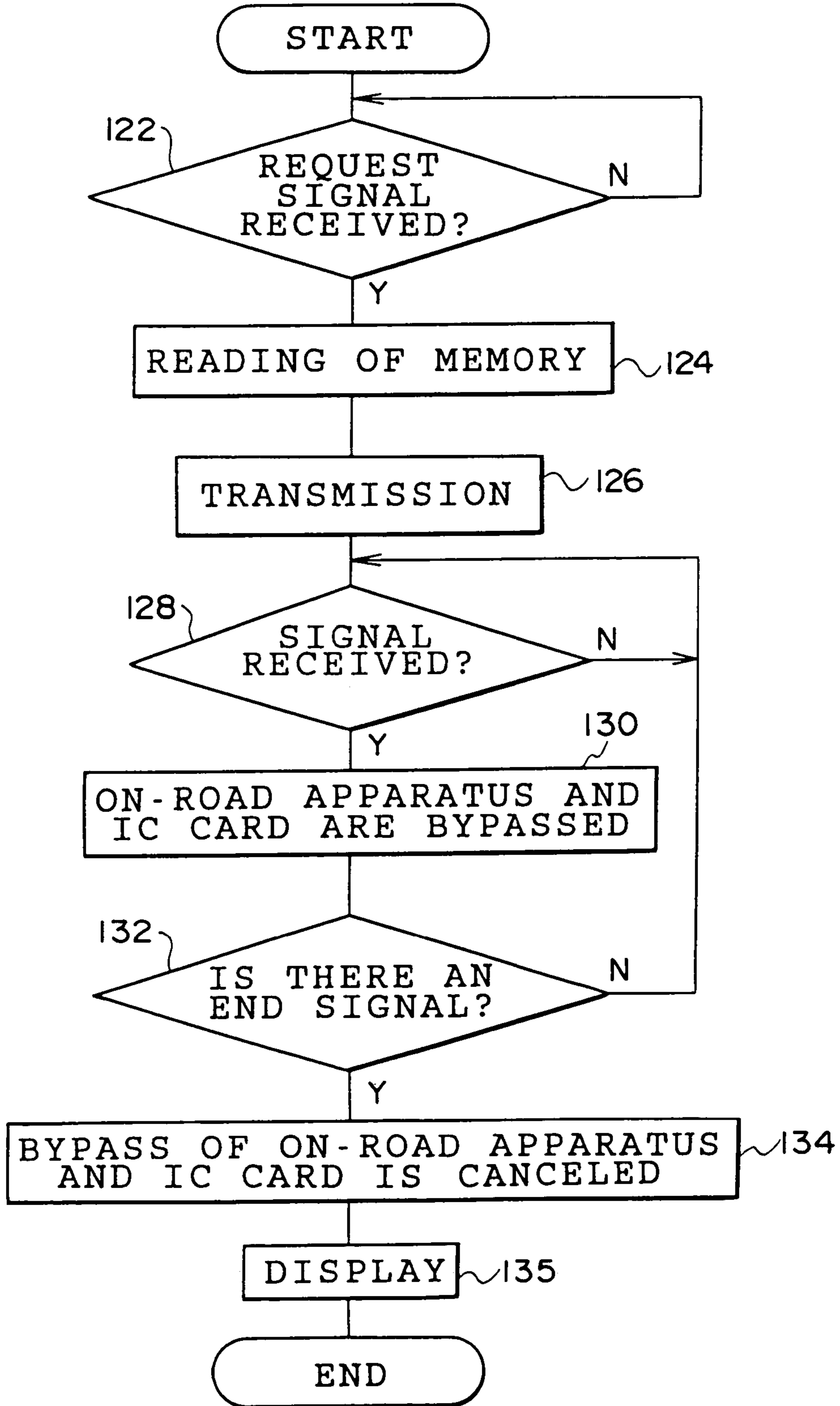
FIG. 8 EXIT GATE PROCESS OF VEHICLE- MOUNTED APPARATUS
