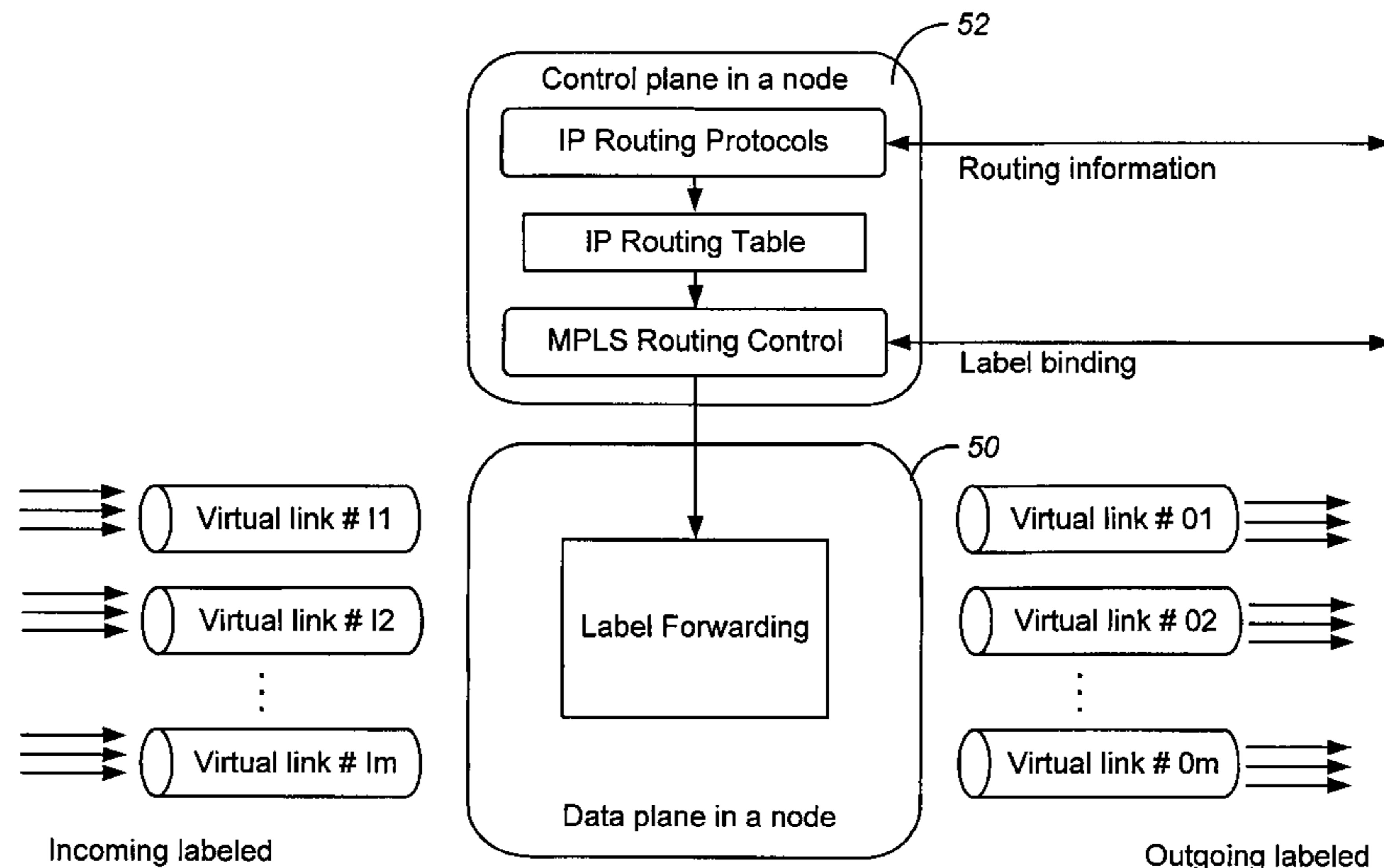
LSR Architecture
