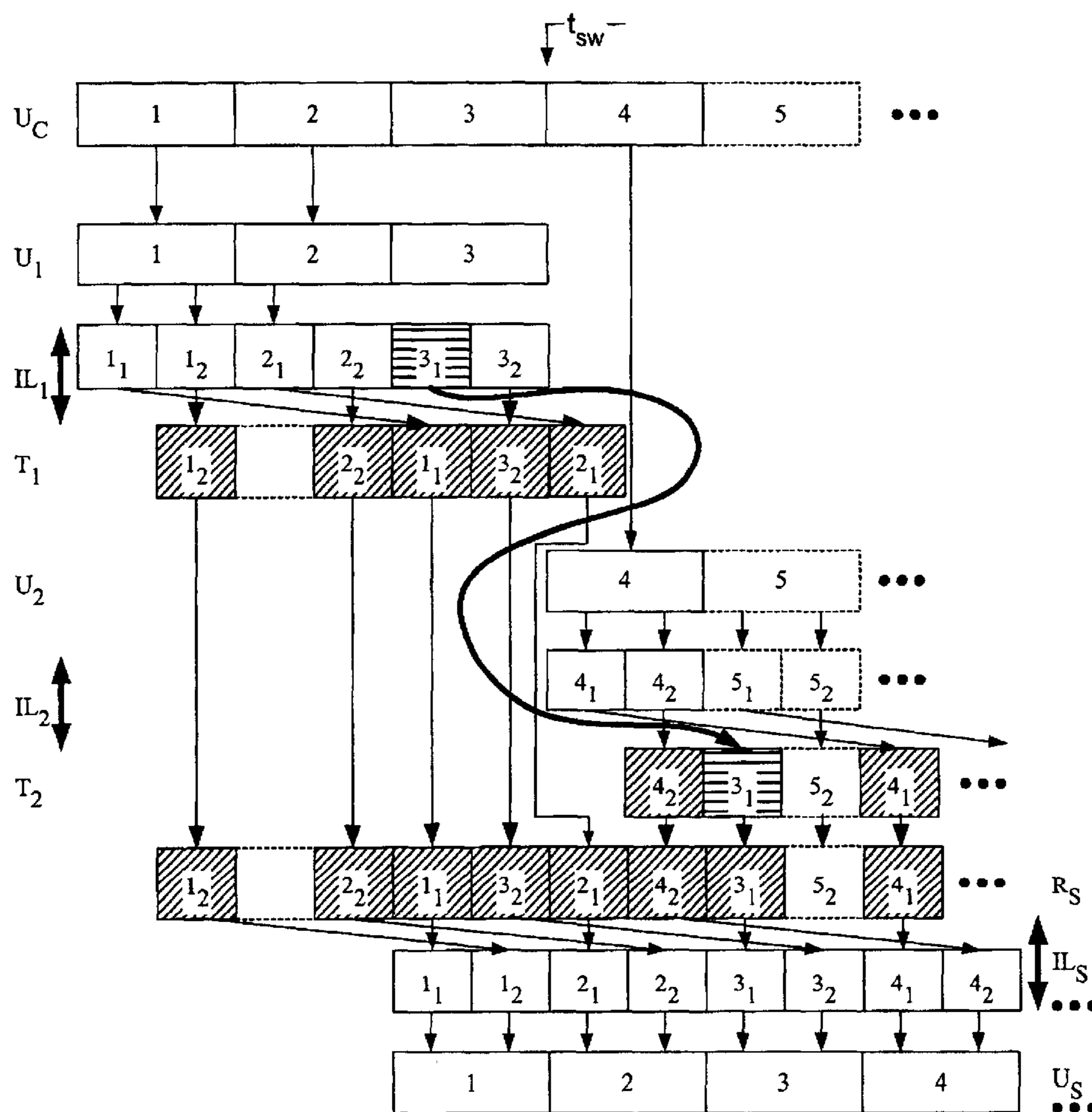
FIG. 5 DOWNLINK (switch)
