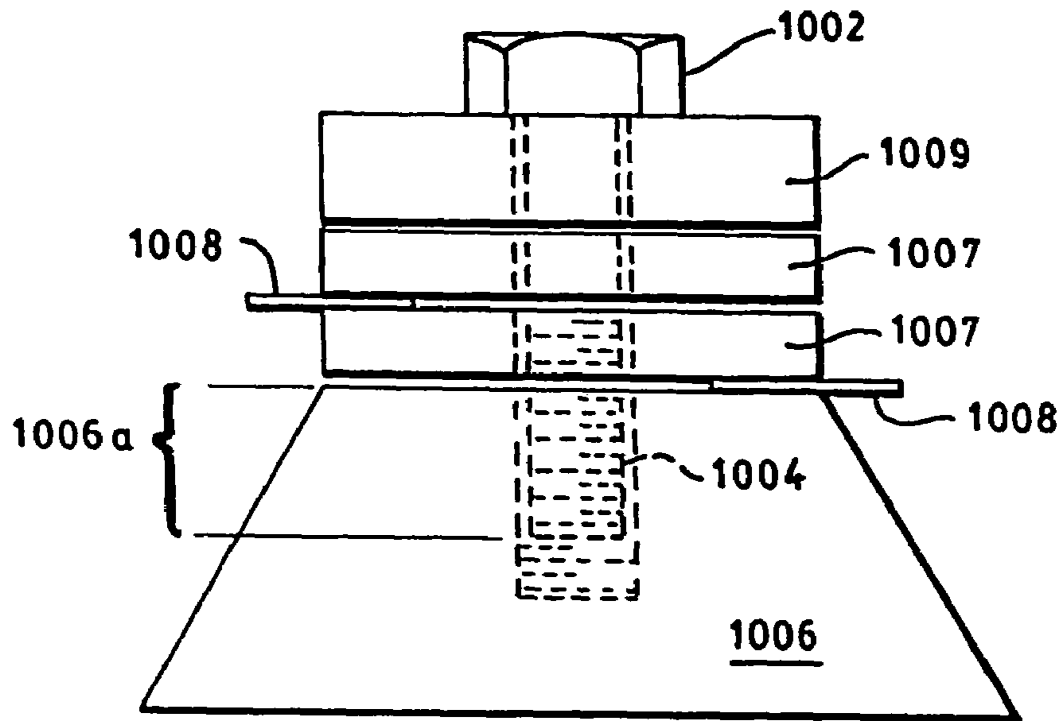
FIG. 51 (PRIOR ART)
