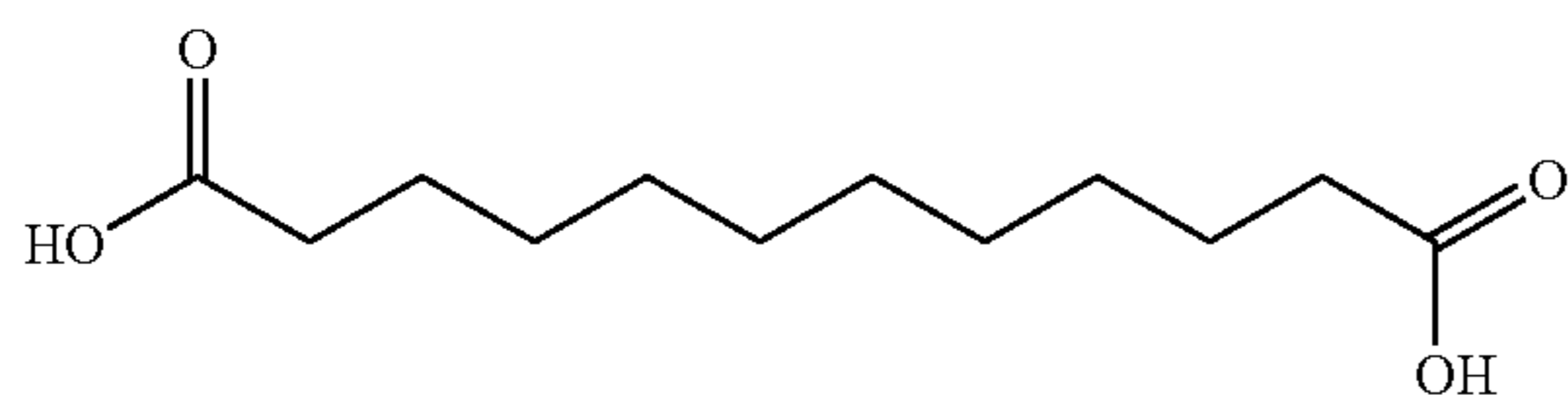
Diacids
