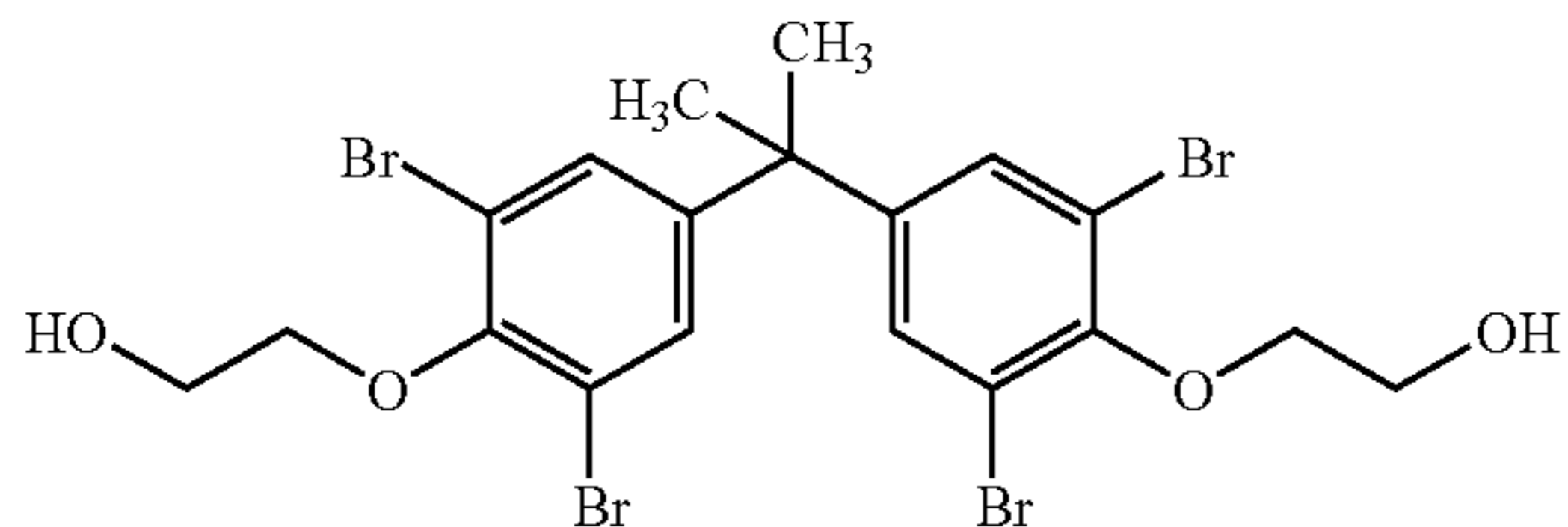
Diols
