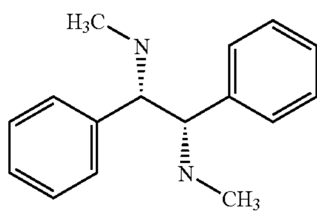
Chiral
