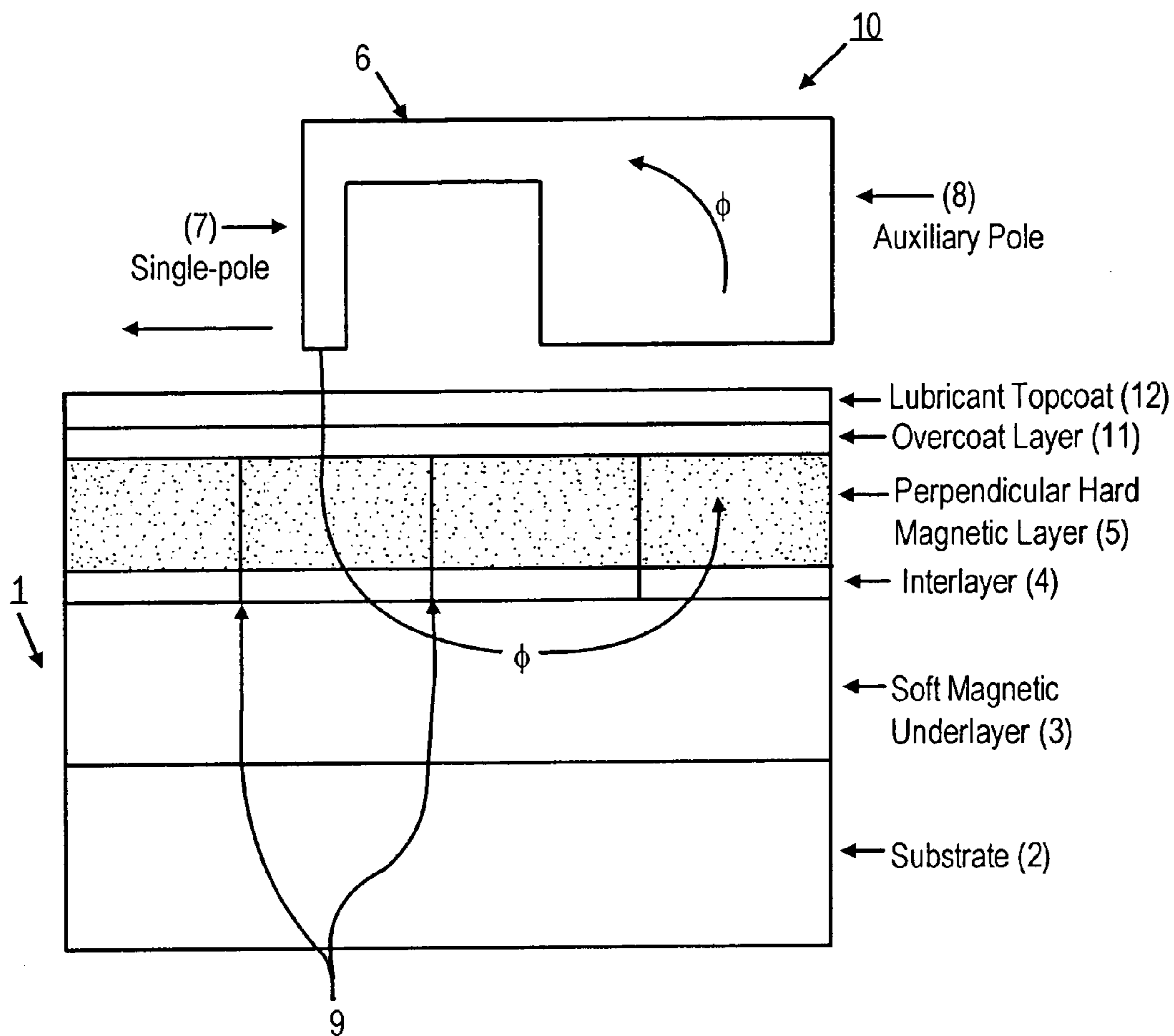
FIG. 1 (PRIOR ART)
