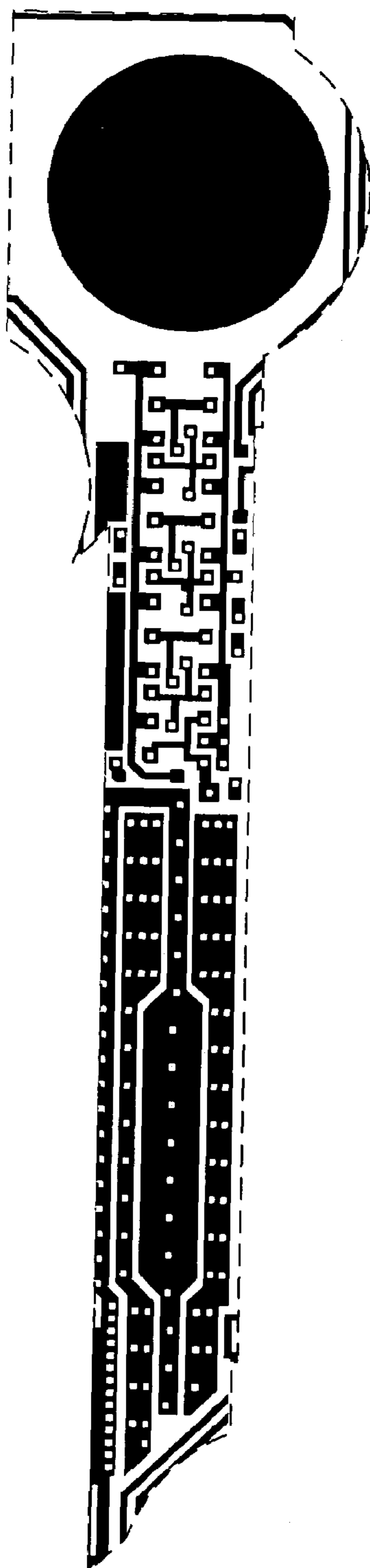
Metal 1 mask
