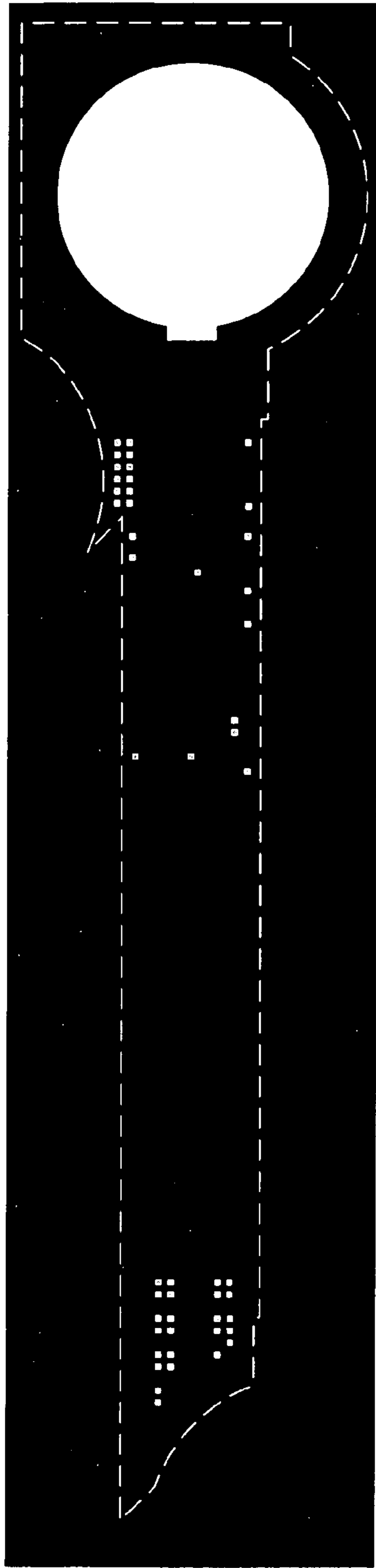
Via 1 mask
