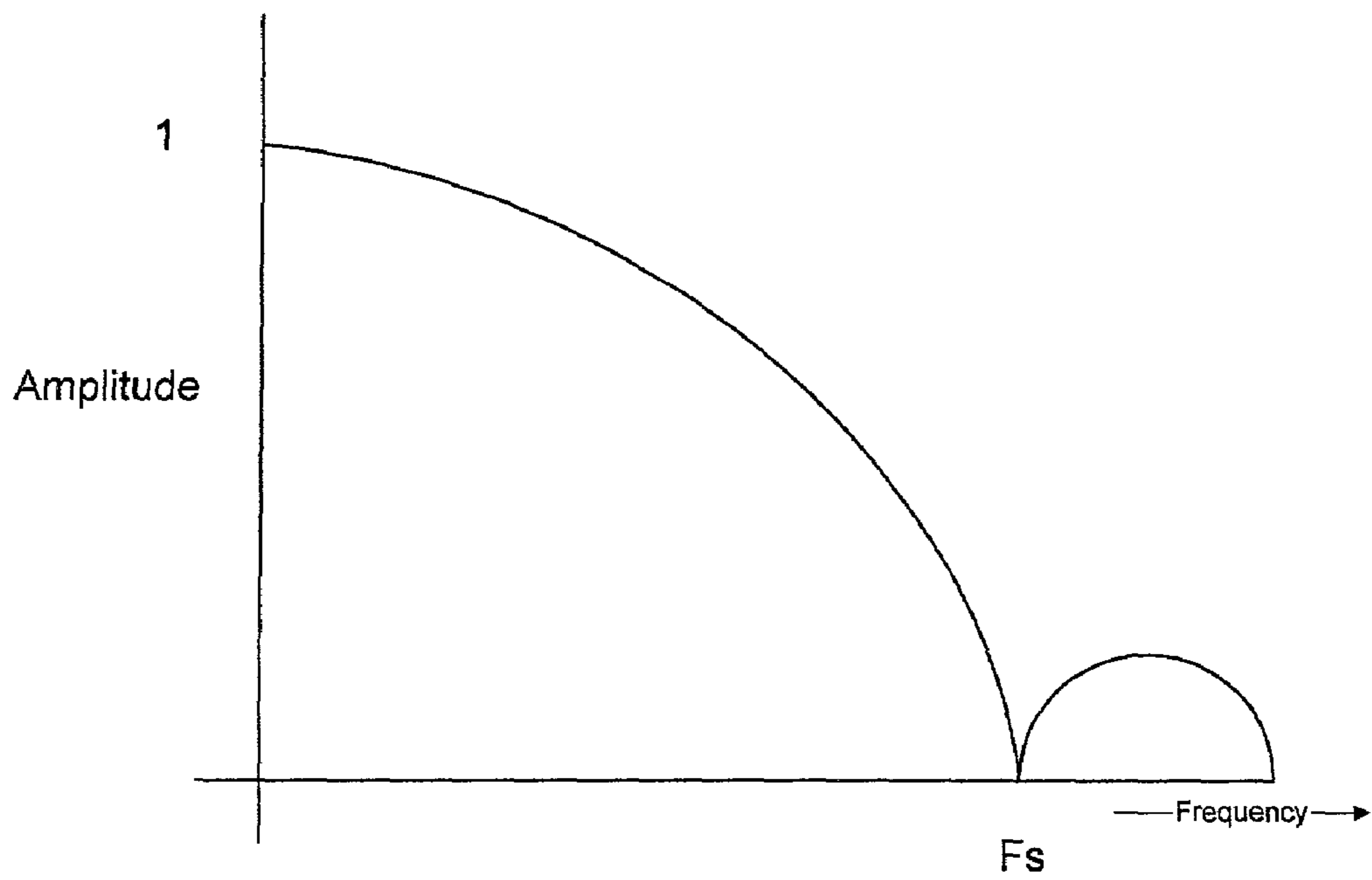
SDV NRZI Spectrum
