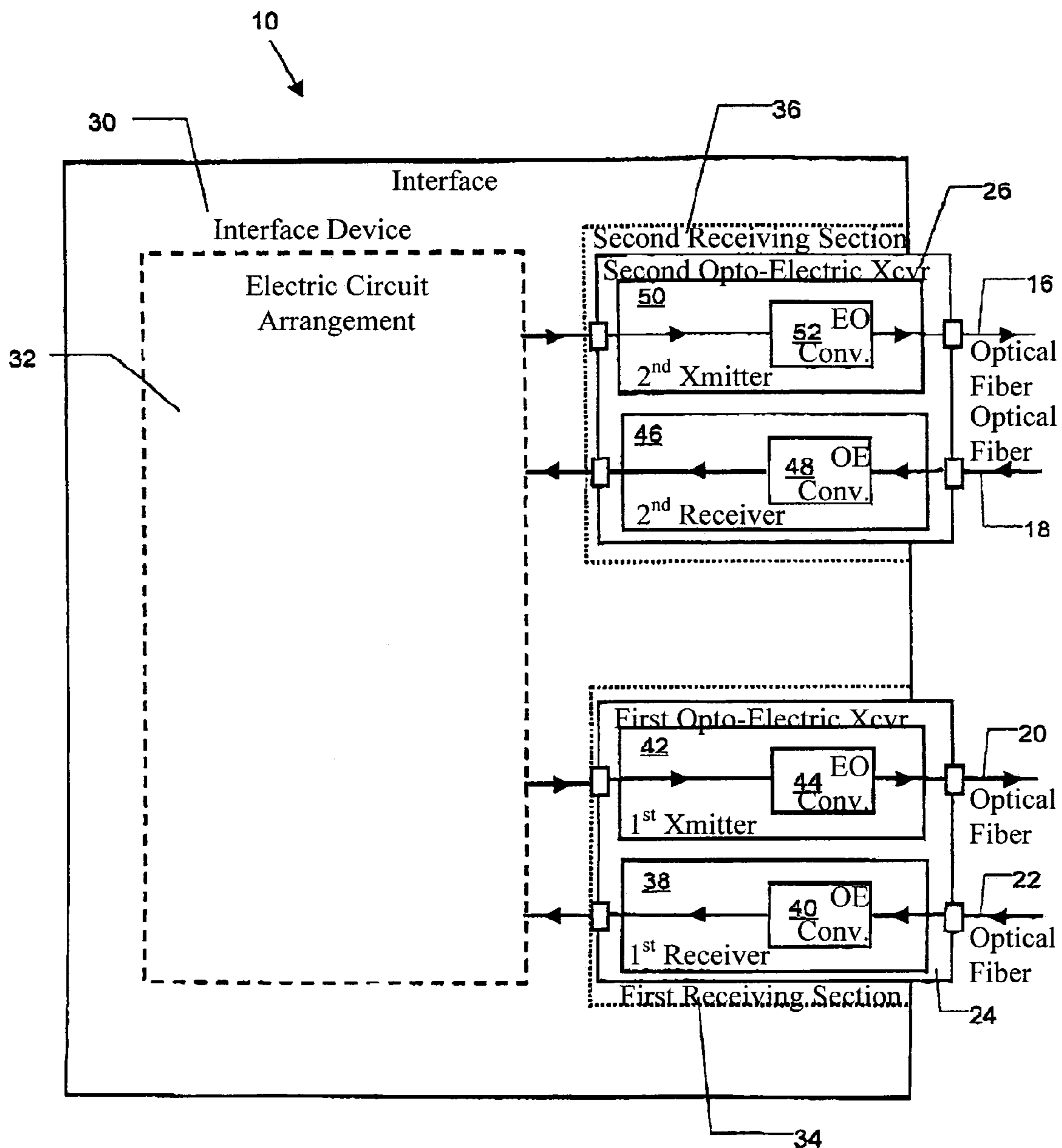
FIG 2 PRIOR ART
