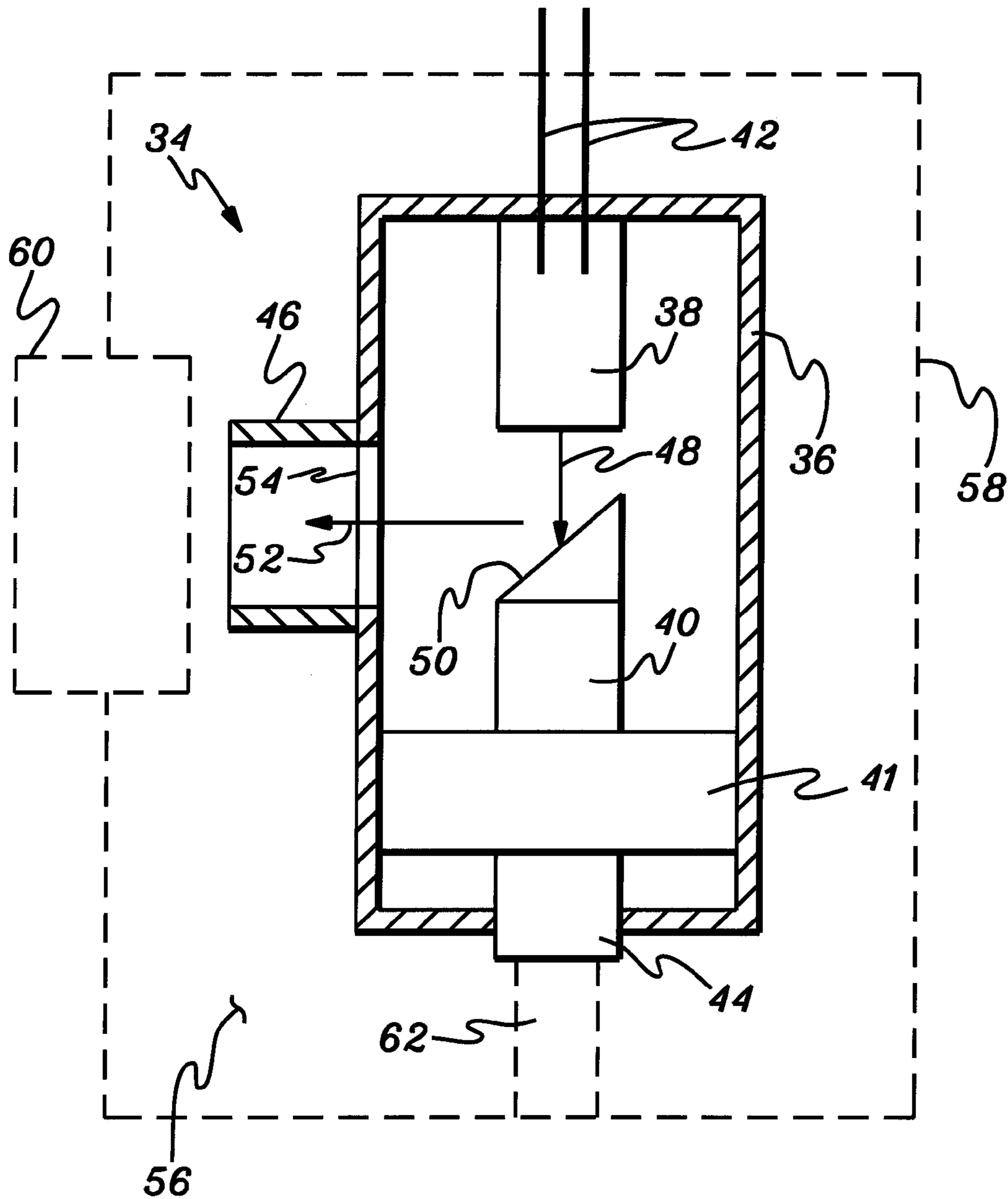
fig. 2 (PRIOR ART)
