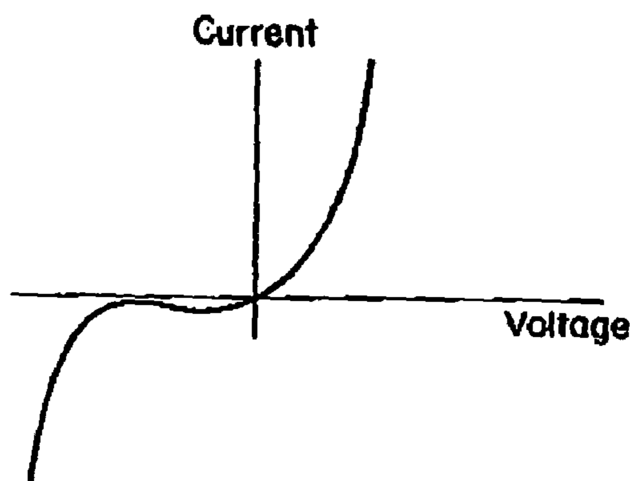
BACK TUNNEL DIODE
