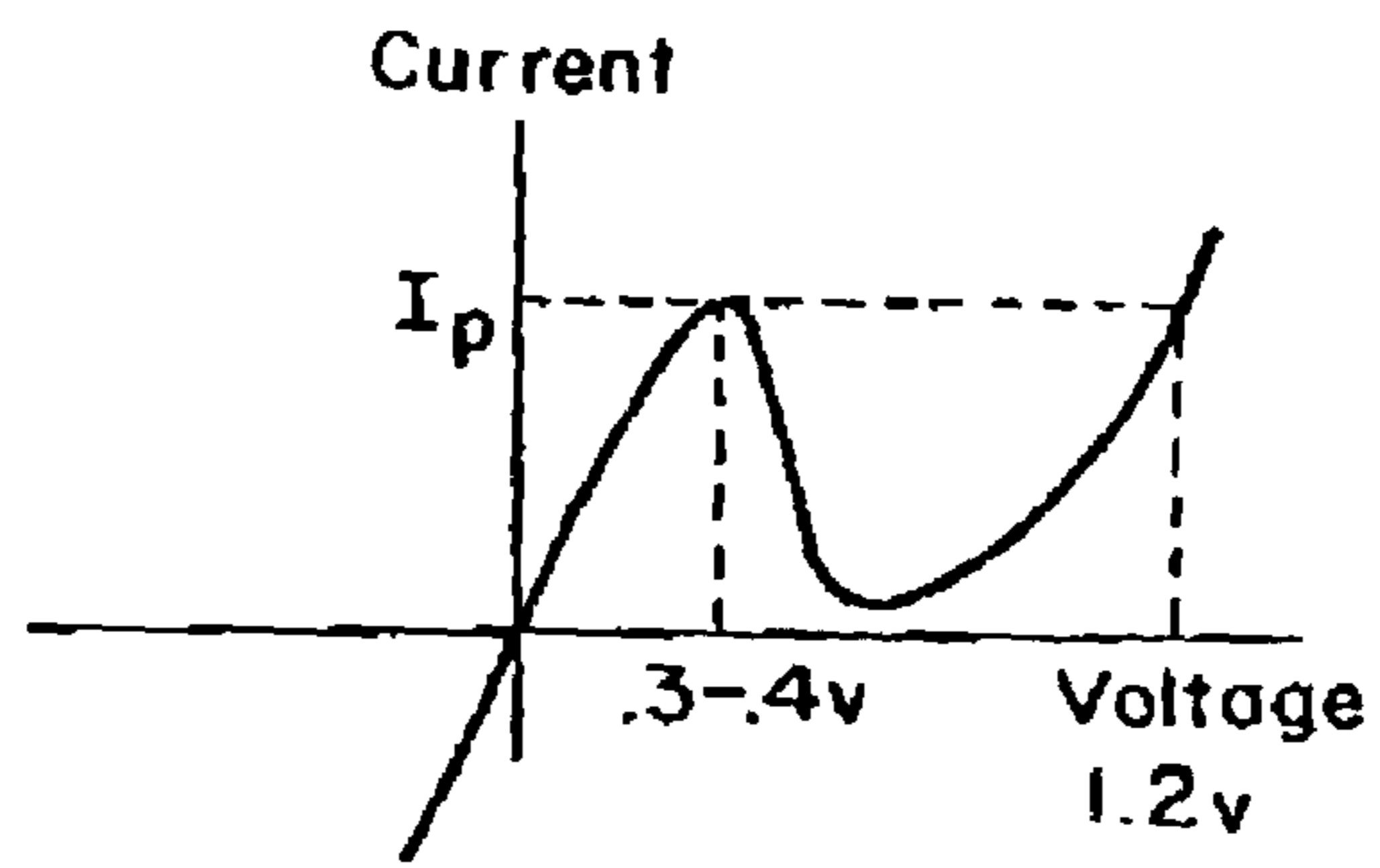
TUNNEL DIODE
