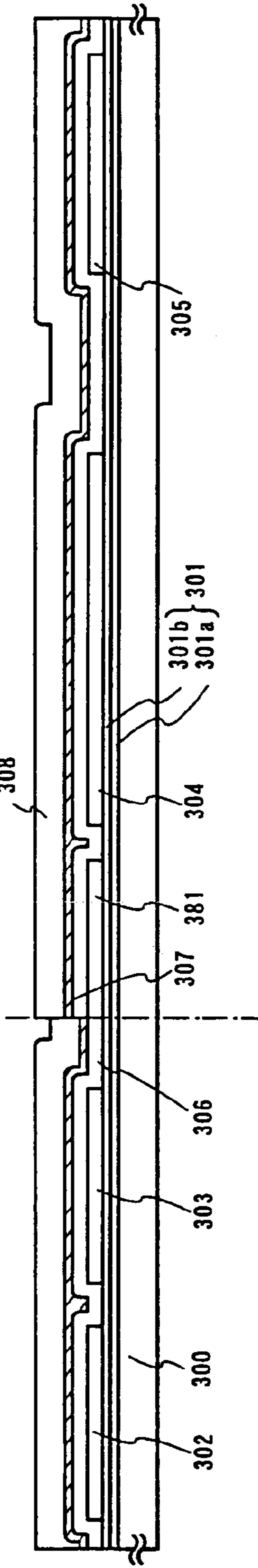
Fig. 21A semiconductor layer formation/insulating film formation of first and second conductive films
