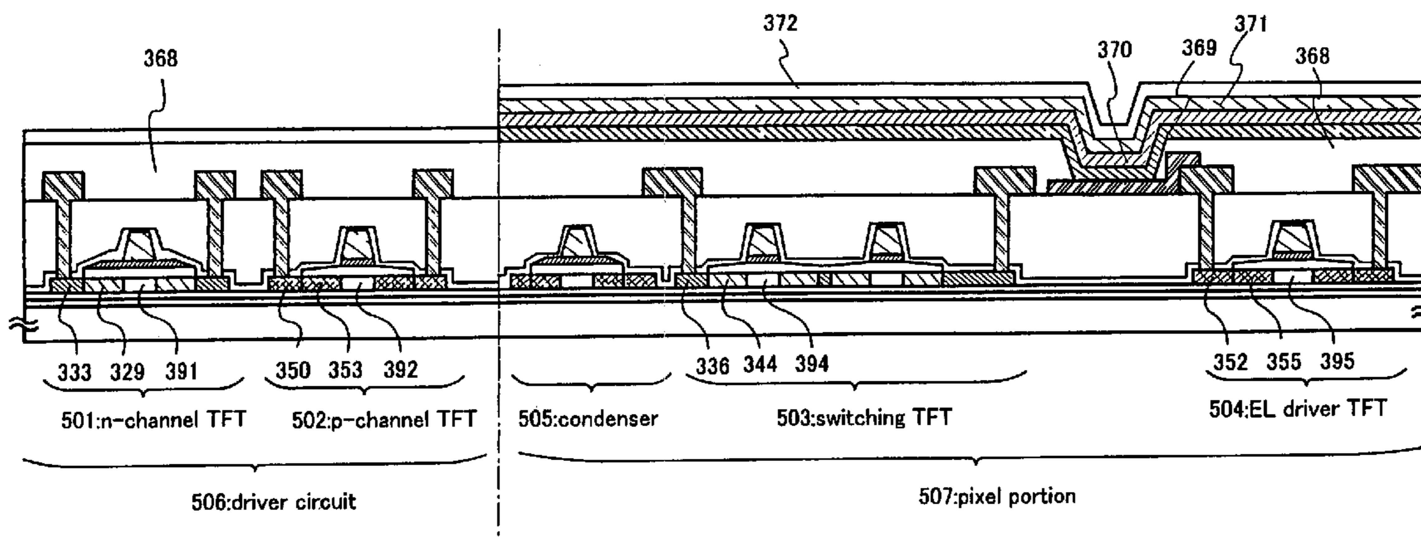
formation of third interlayer insulating film, EL layer, pixel electrode, passivation film
