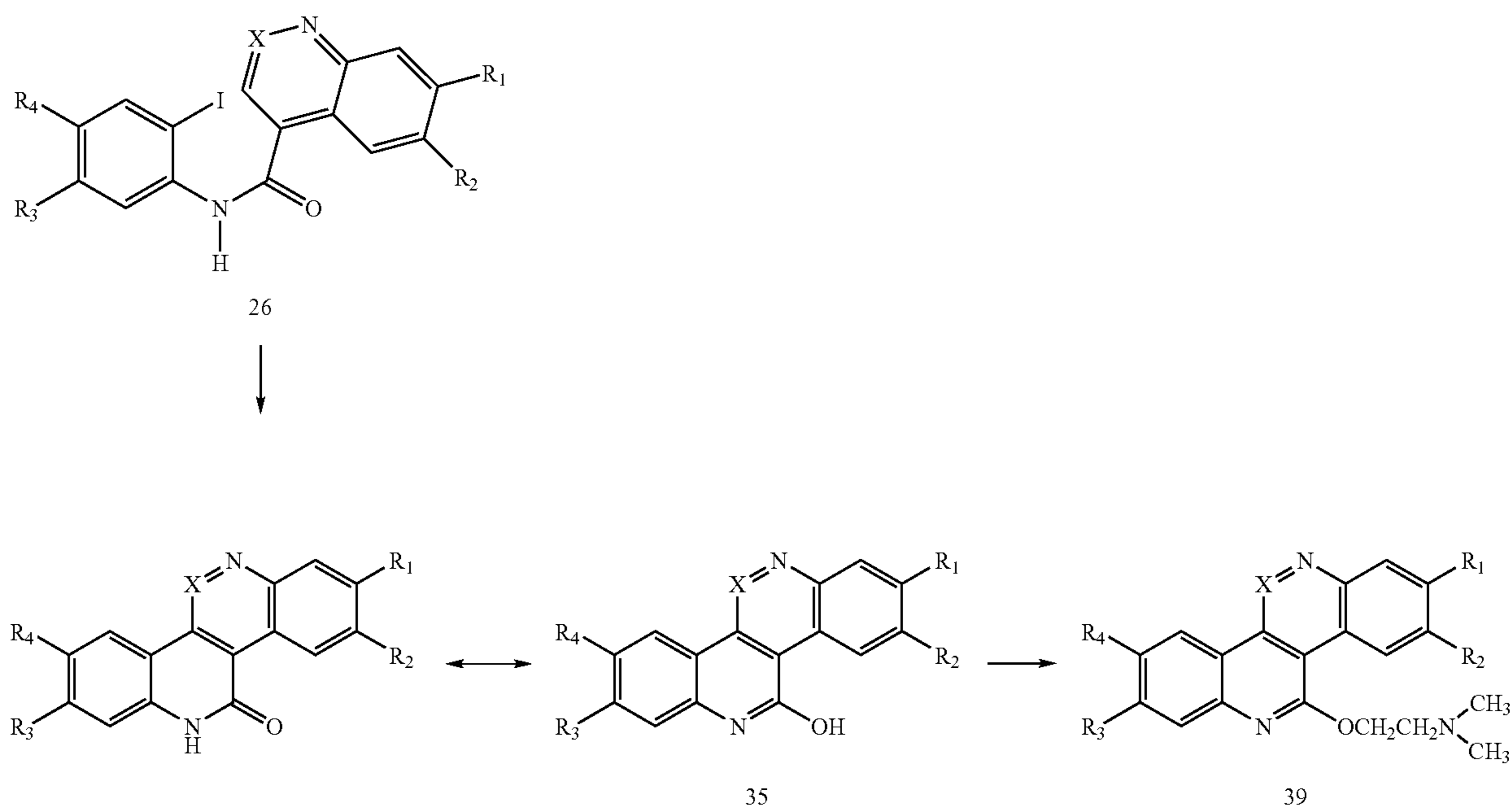
Scheme 4.
