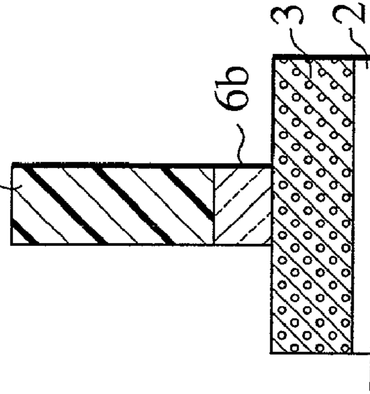
WIRING PATTERN SECTION 5b
