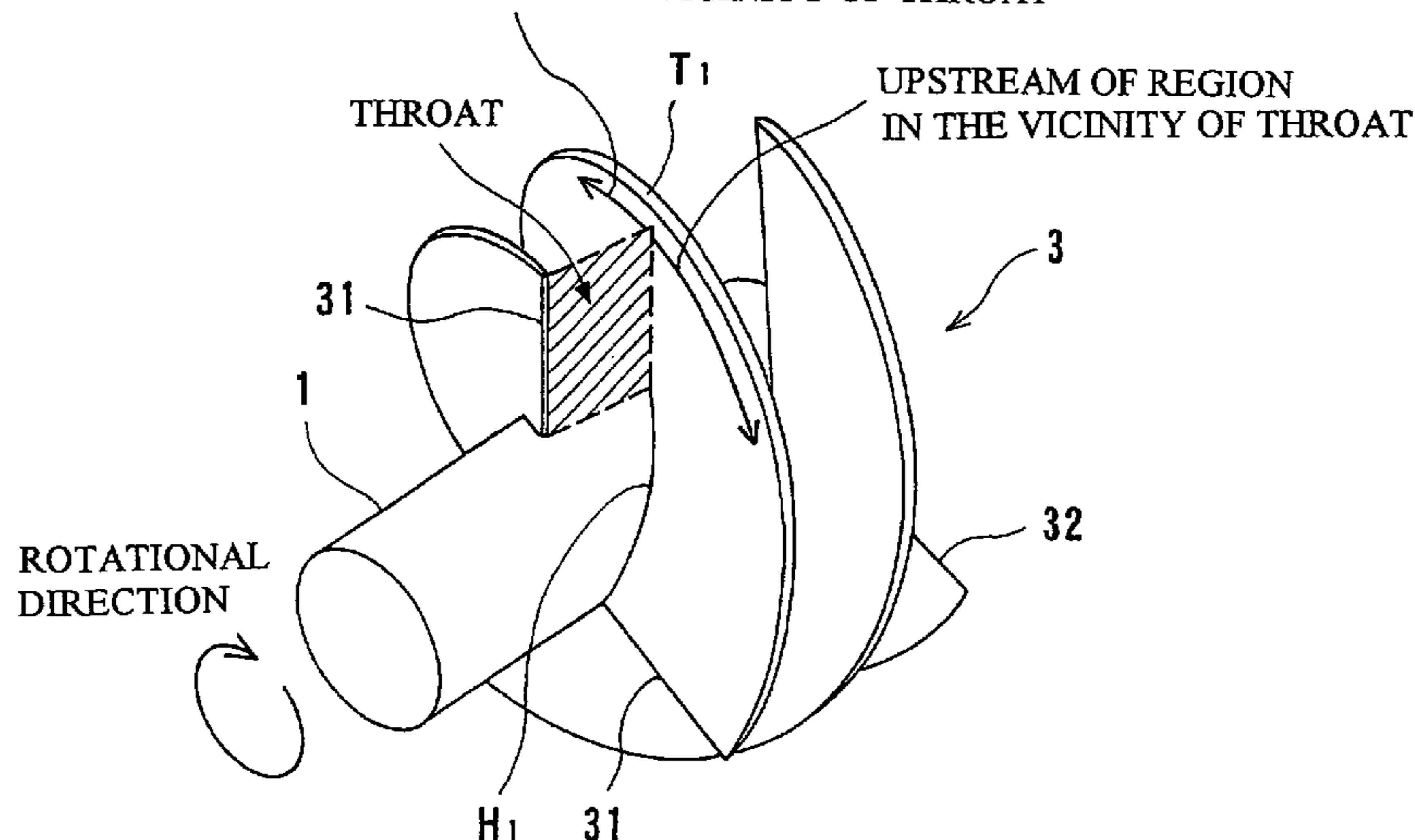
DOWNSTREAM OF REGION IN THE VICINITY OF THROAT
