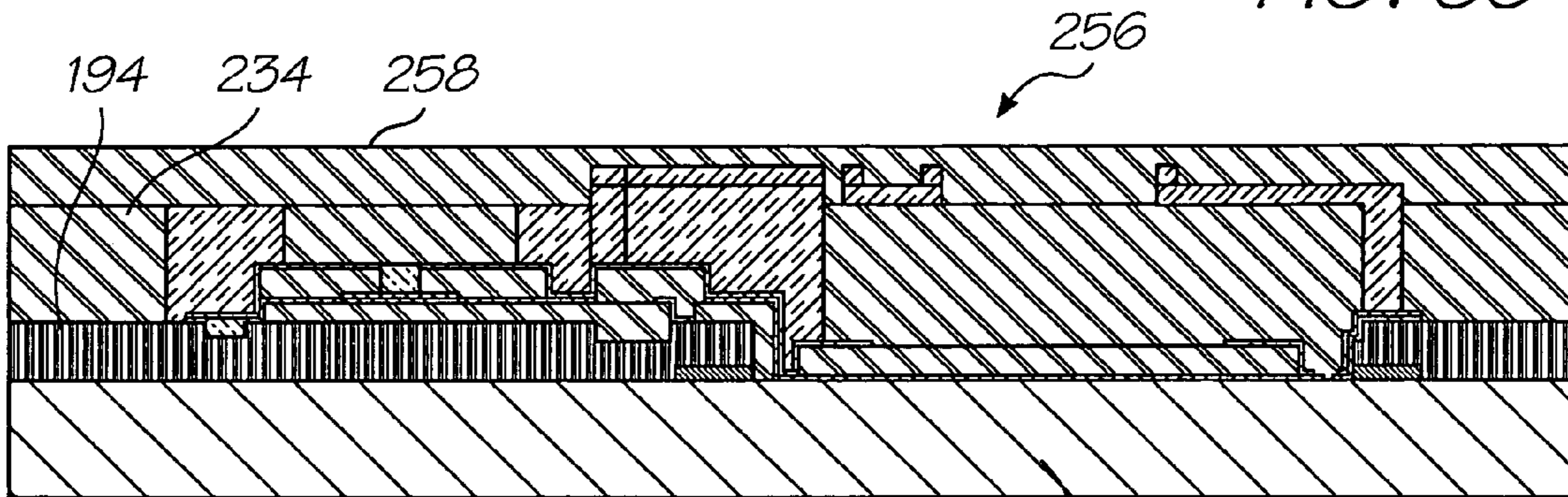
3 micron sacrificial protective polyimide
