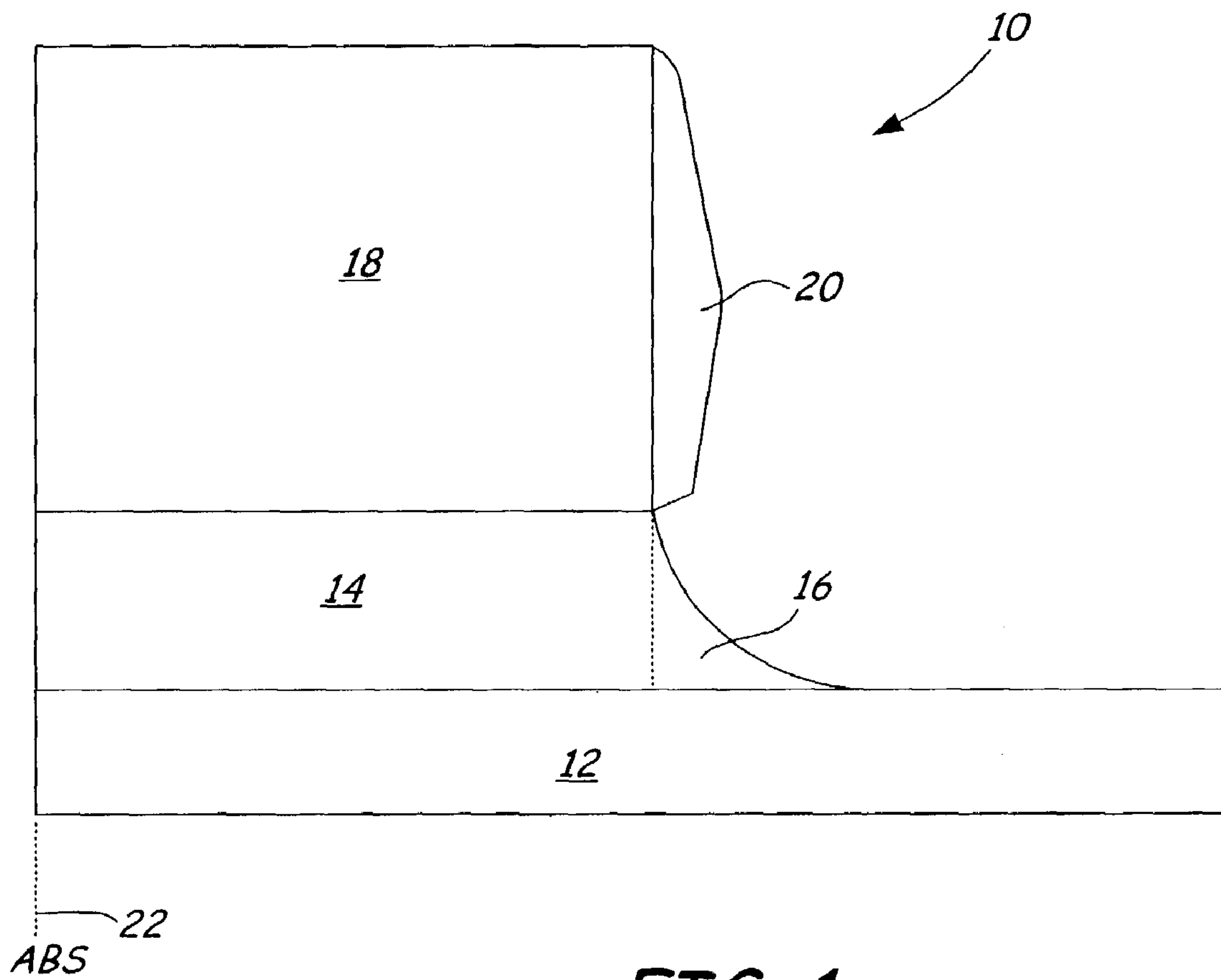
FIG. 1 PRIOR ART
