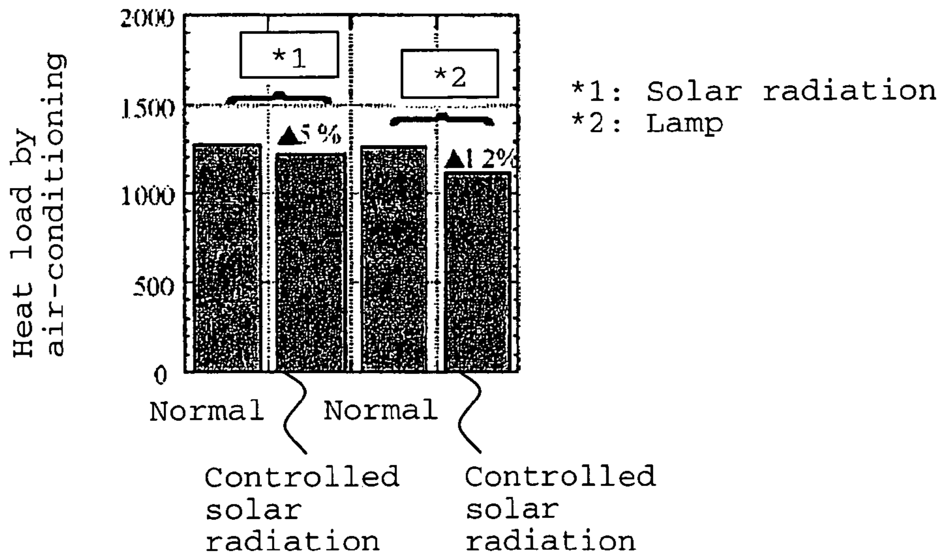
Heat load by air-conditioning of an air conditioner
