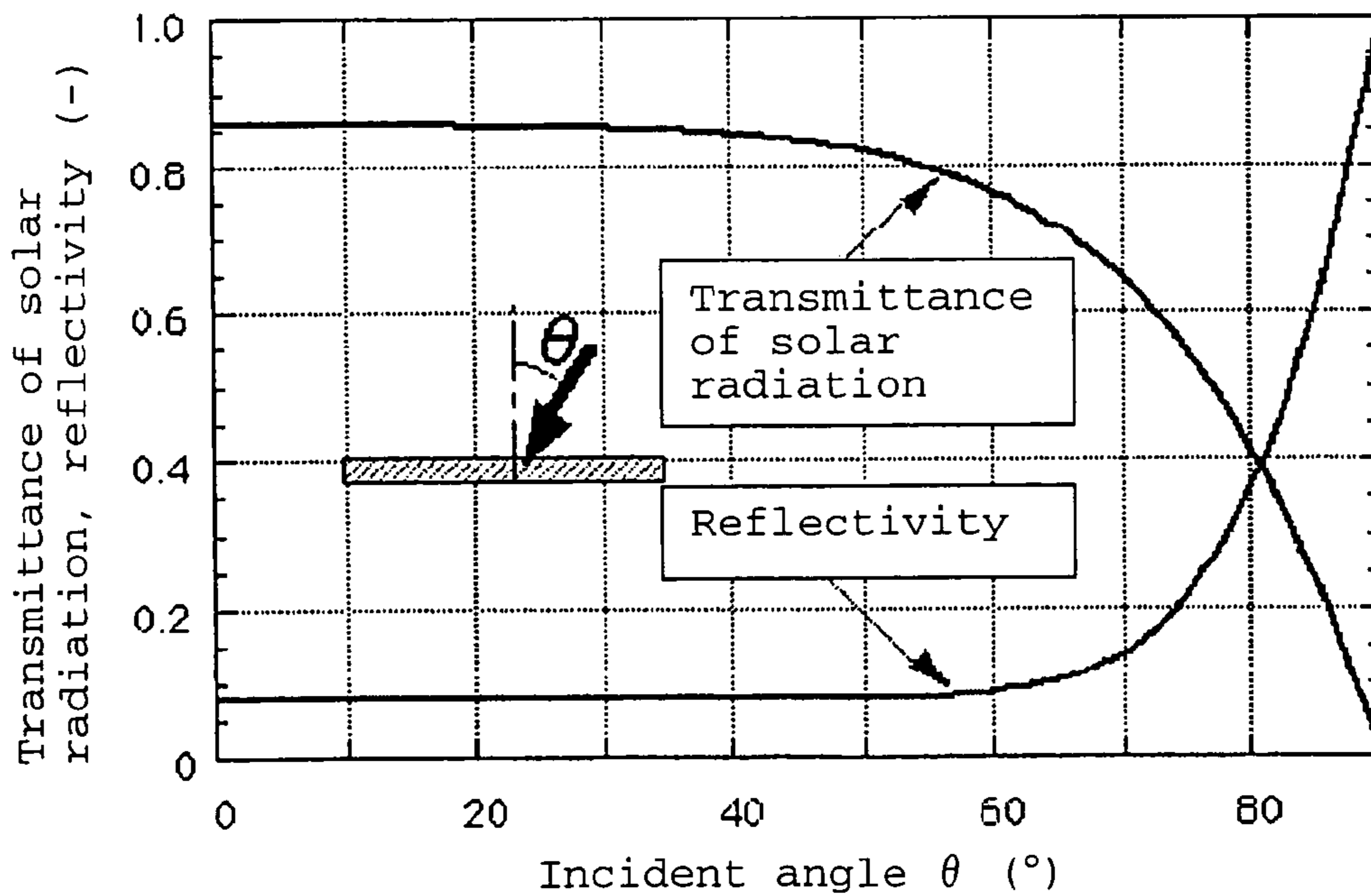
Transparent glass sheet having a thickness of 3 mm with a solar reflection film
