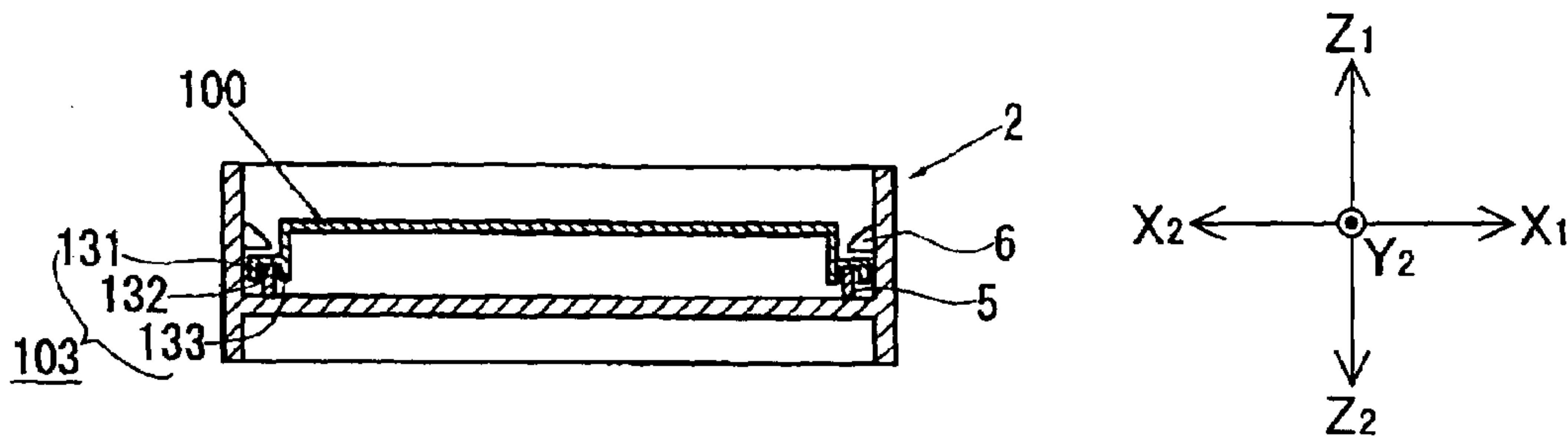
FIG.4 PRIOR ART
