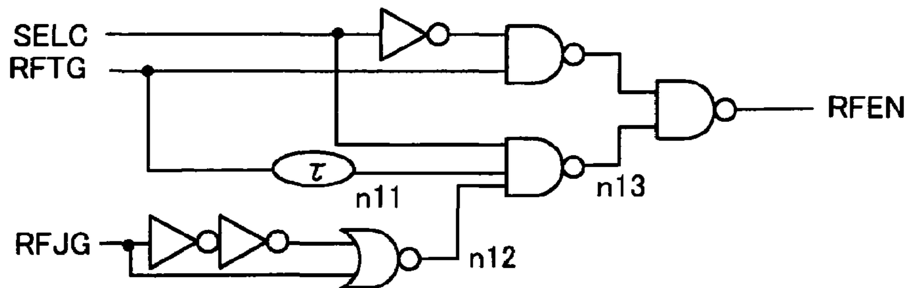
SECOND JUDGMENT SECTION EMPLOYED IN THIRD EMBODIMENT
