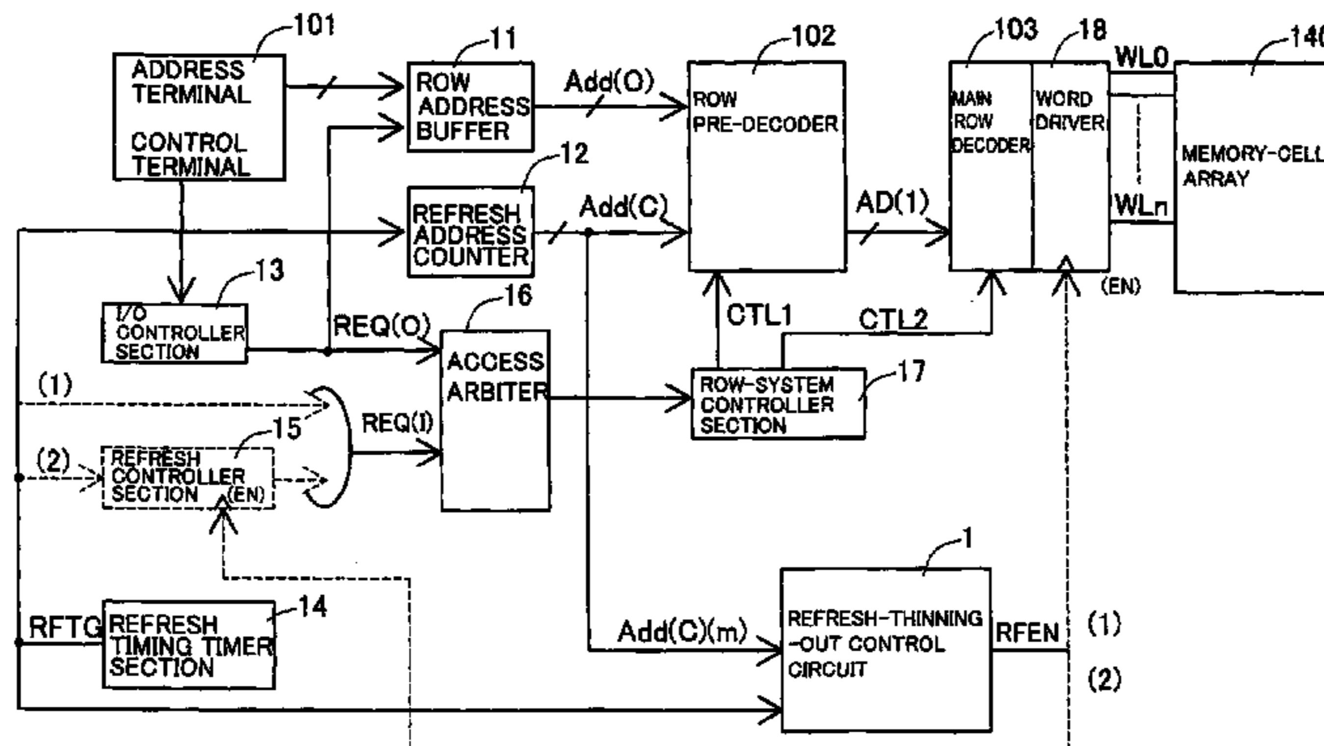
CIRCUIT BLOCK DIAGRAM OF FIRST EMBODIMENT
