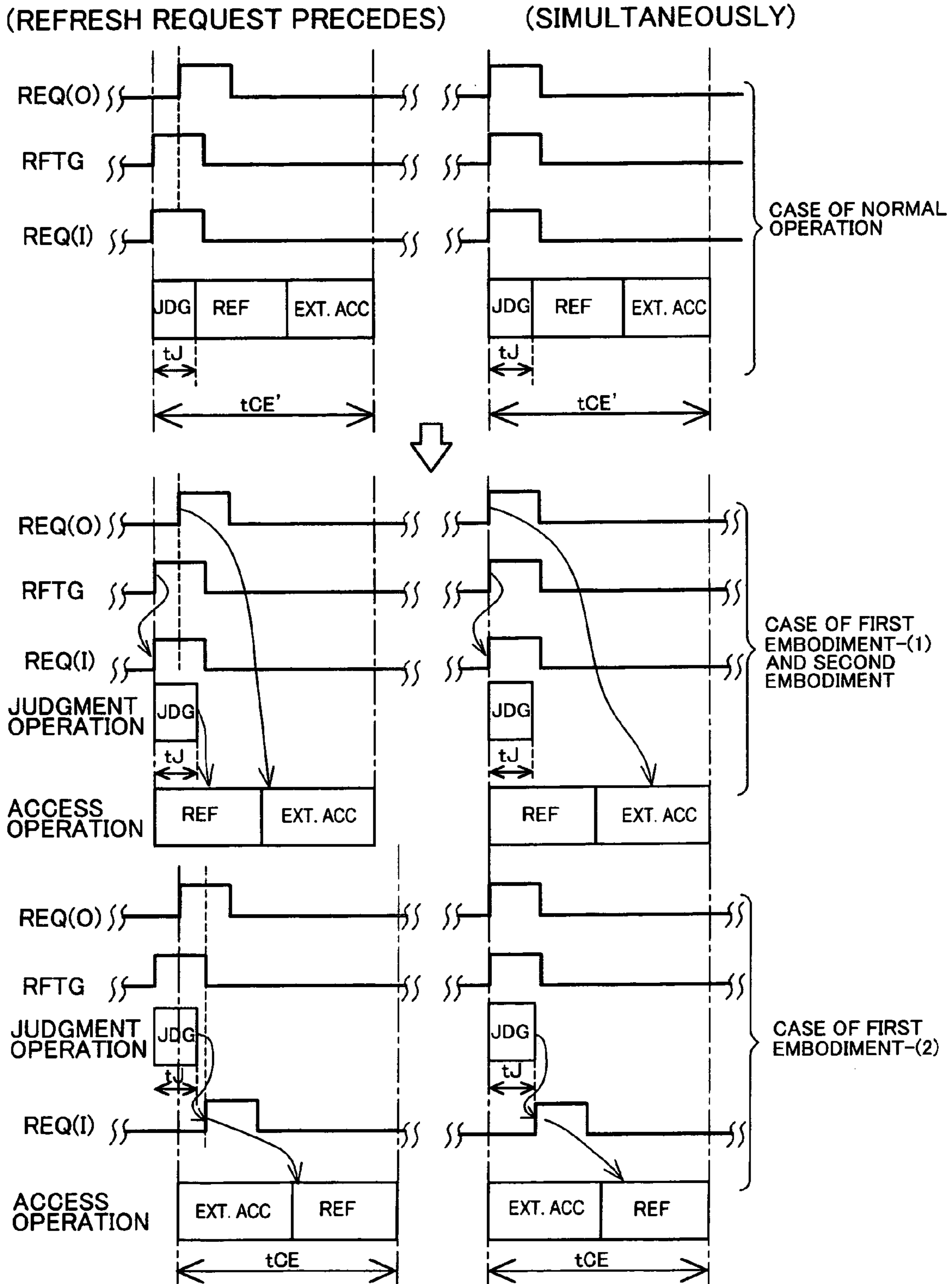
FIG. 7 OPERATIONAL WAVEFORMS SHOWING ACCESS COMPETITION IN PSEUDO SRAM
