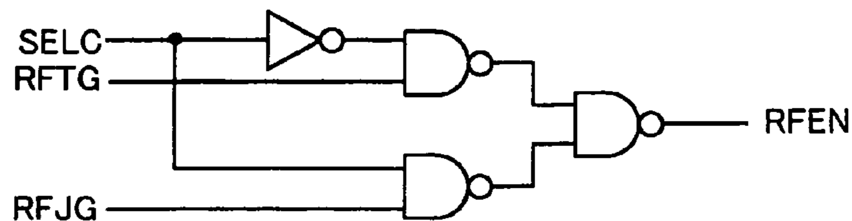
FIRST JUDGMENT SECTION EMPLOYED IN THIRD EMBODIMENT
