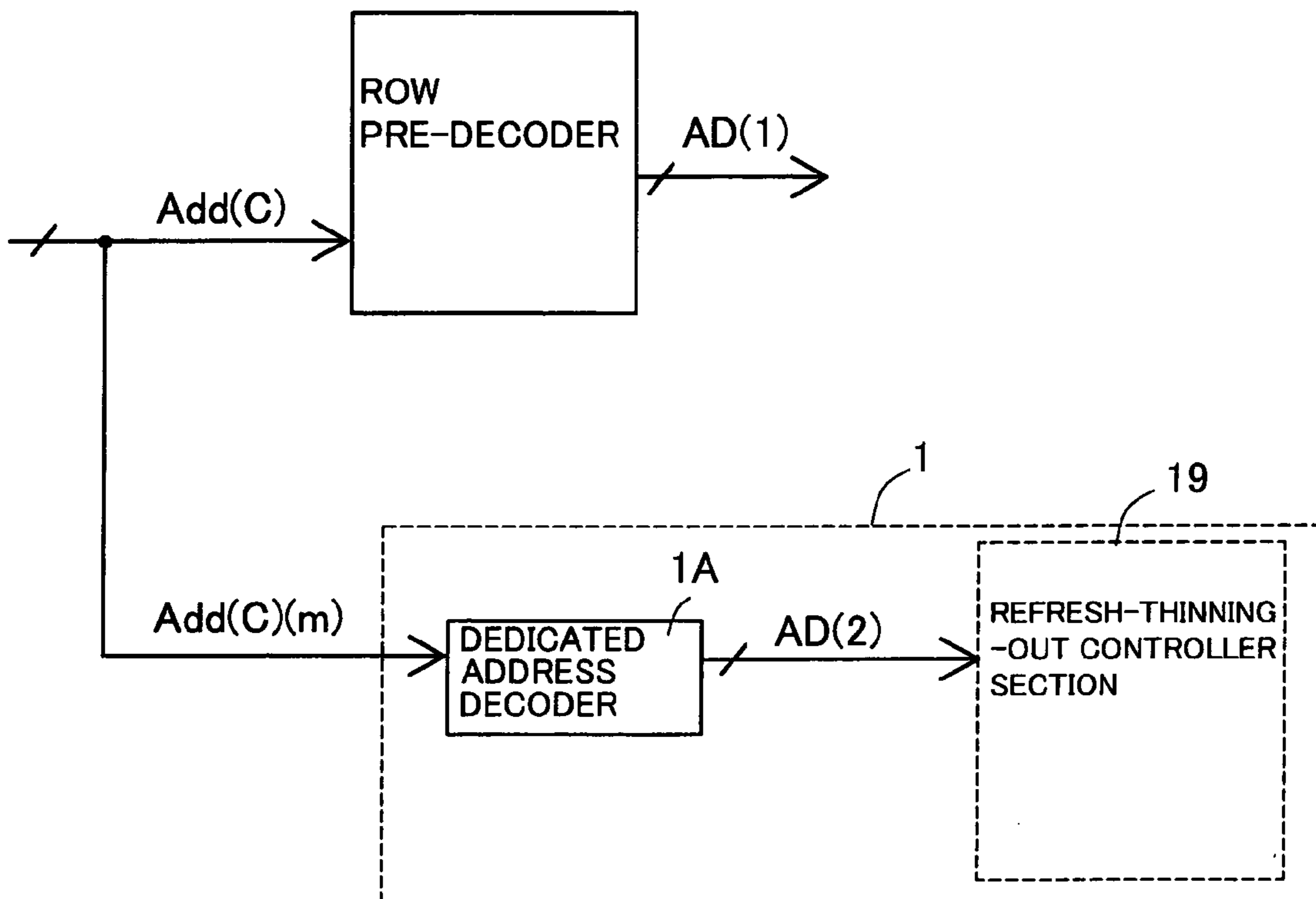
EXAMPLE OF INPUT OF ADDRESS TO REFRESH-THINNING-OUT CONTROL CIRCUIT EMPLOYED IN FIRST EMBODIMENT
