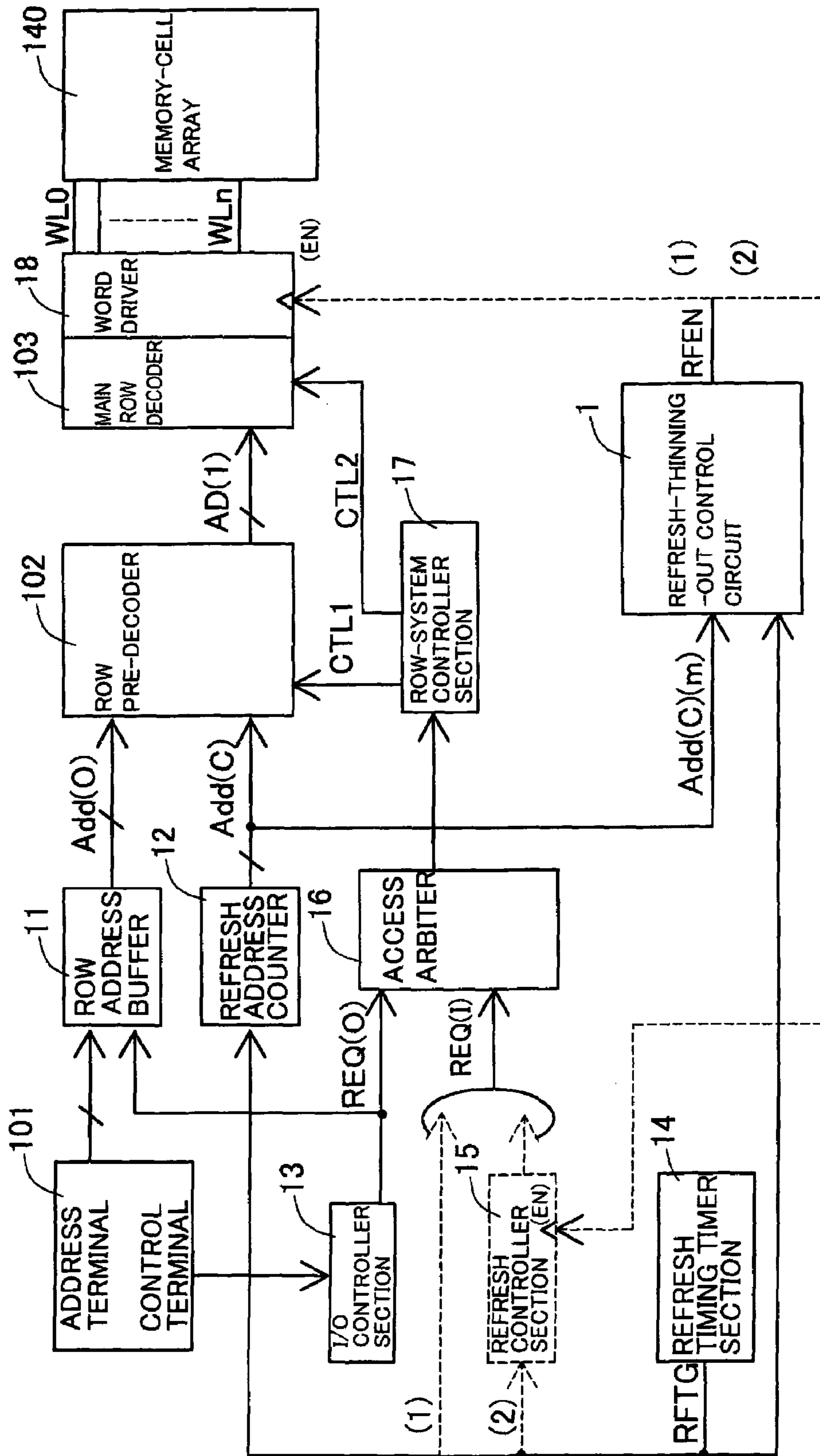
FIG. 1 CIRCUIT BLOCK DIAGRAM OF FIRST EMBODIMENT
