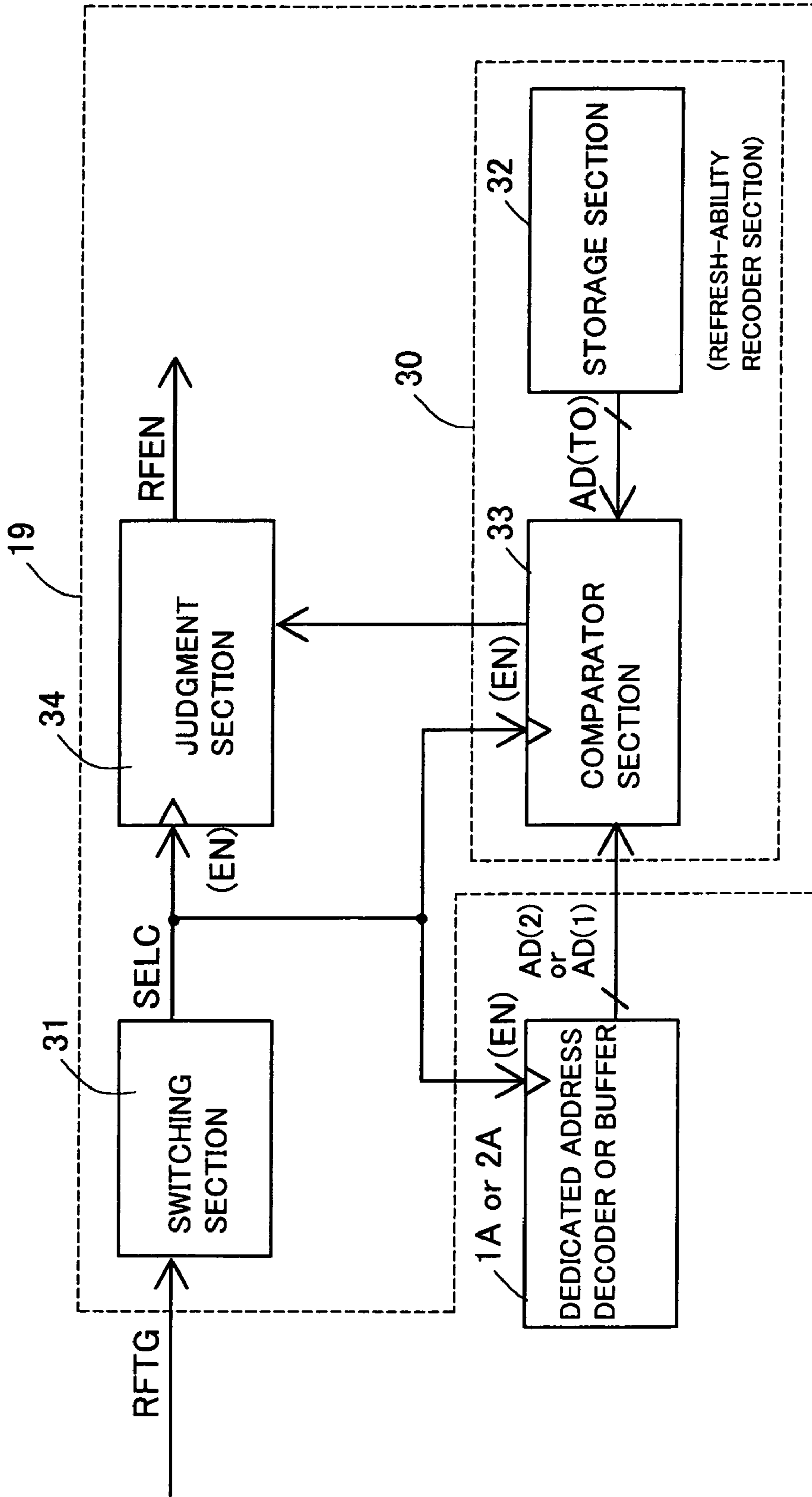
FIG. 12 REFRESH-THINNING-OUT CONTROL CIRCUIT (THIRD EMBODIMENT)
