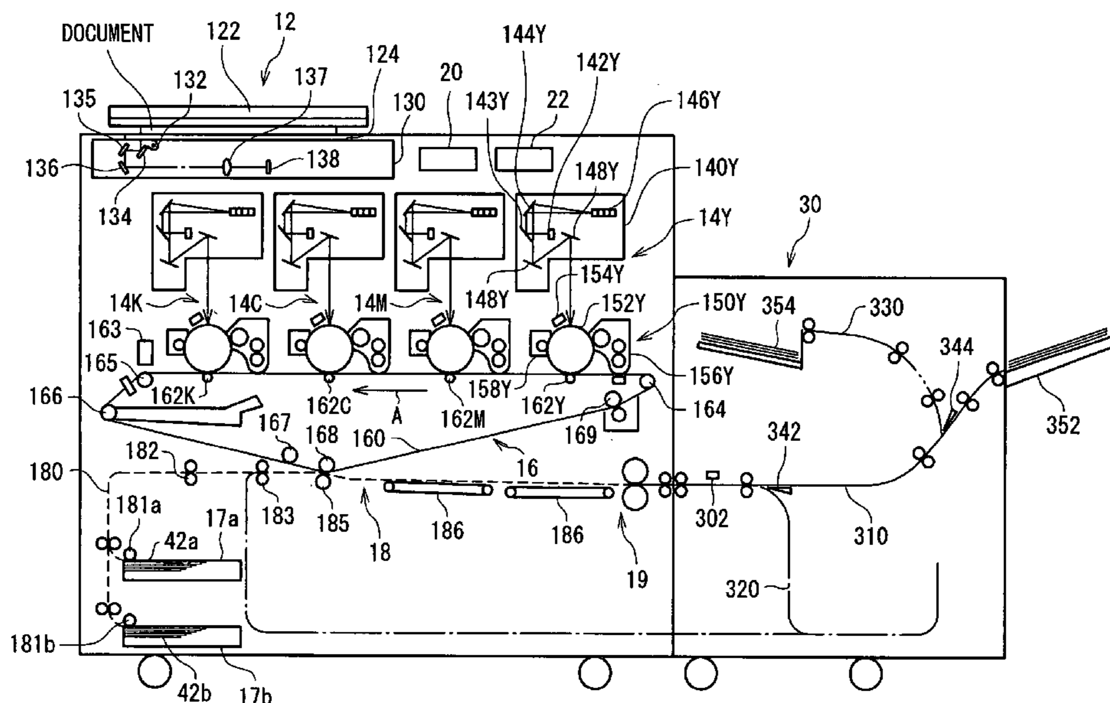
10 PRINTER DEVICE
