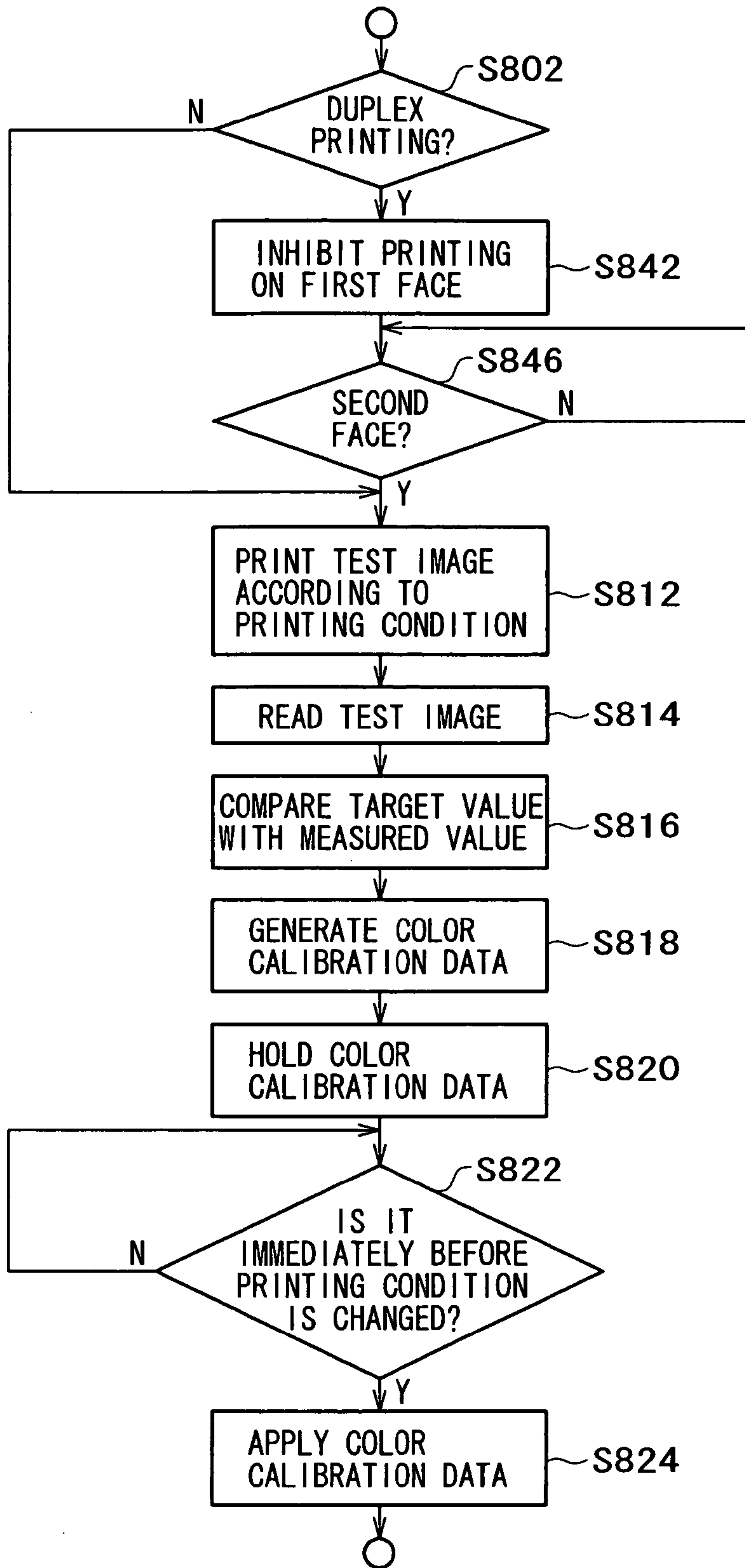
COLOR CALIBRATION PROCESS DURING PRINTING
