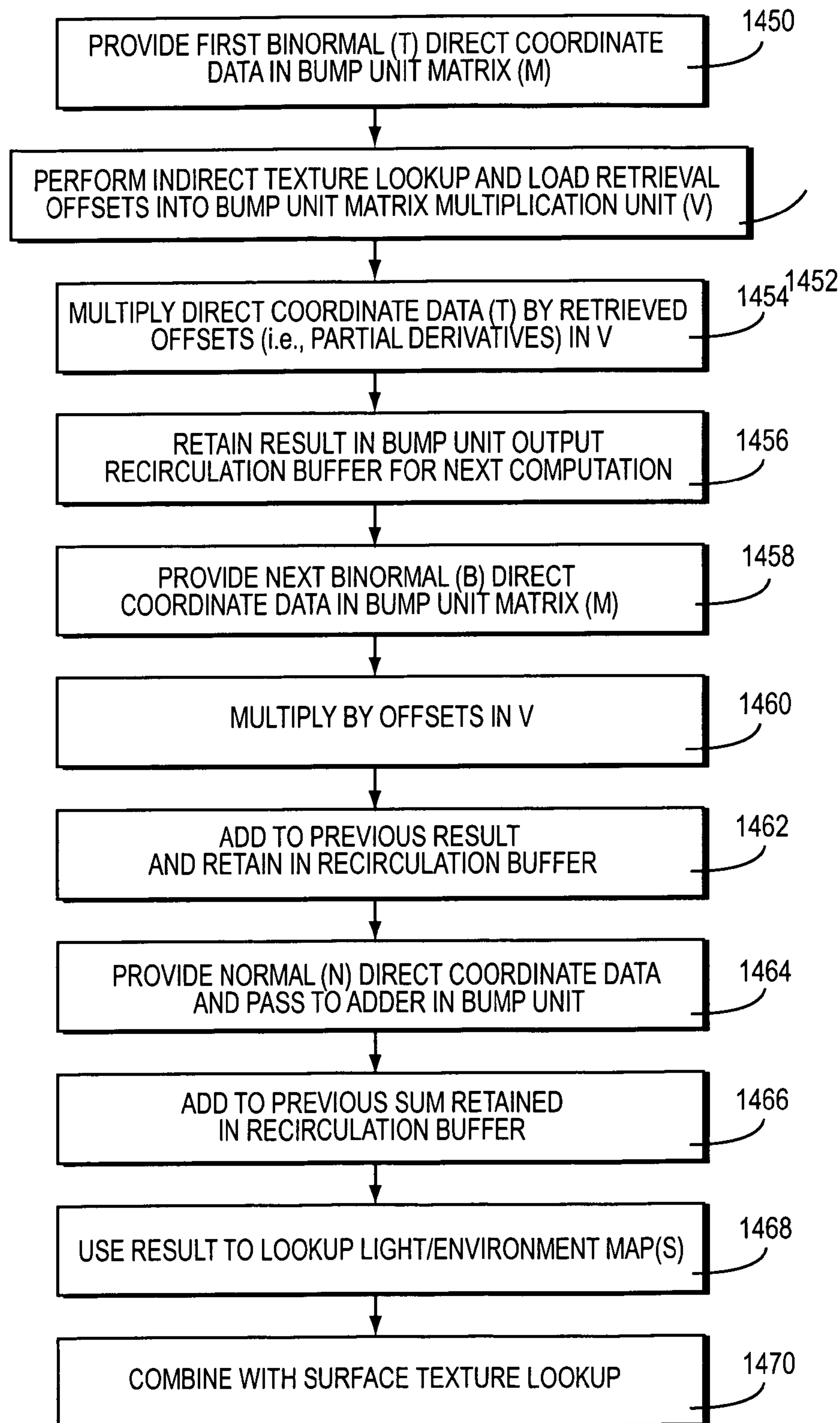
FIG. 27 DETAILED EXAMPLE EMBM (dSdT) PROCESS STEPS
