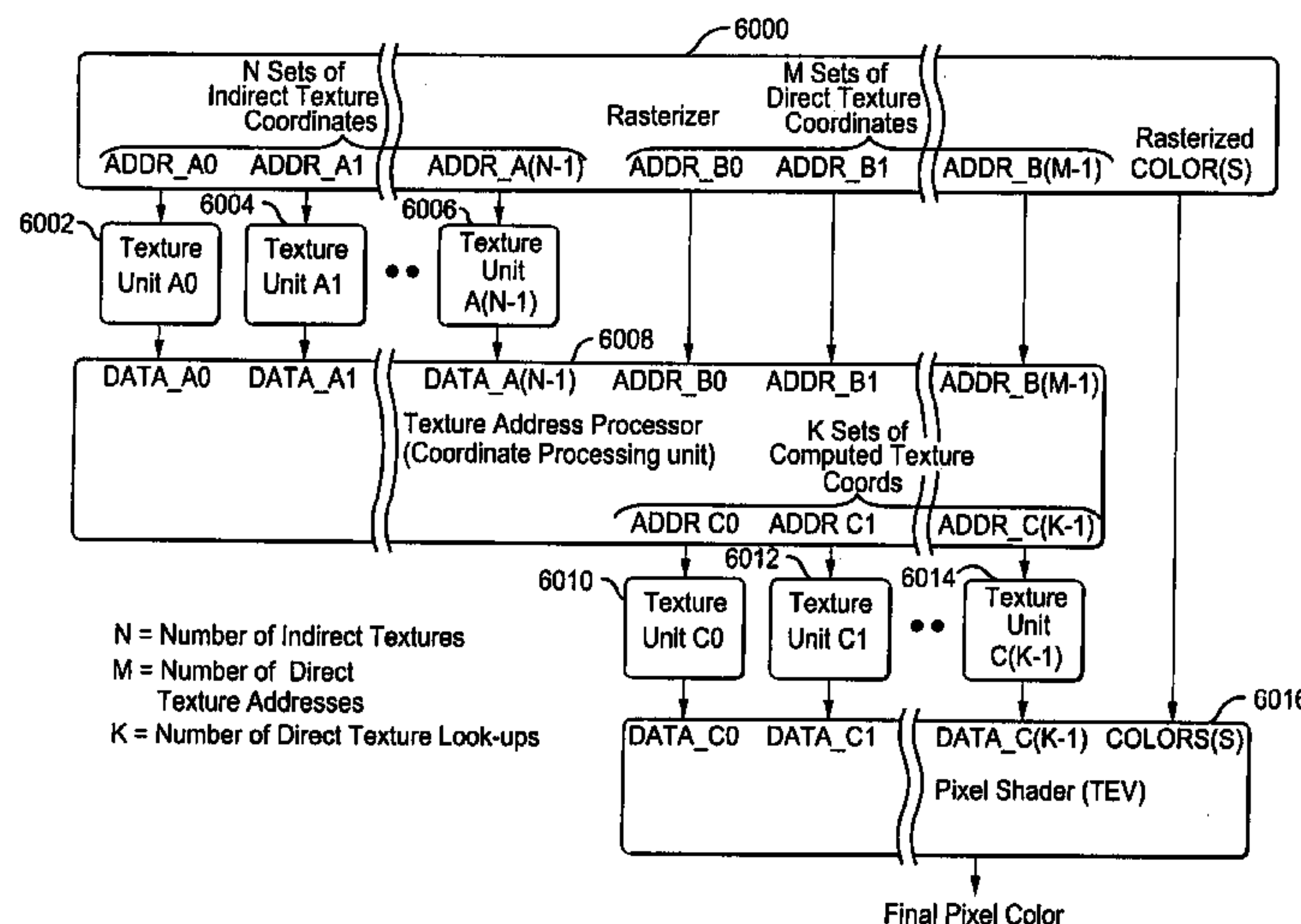
Logical Block Diagram of Indirect Texture Processing
