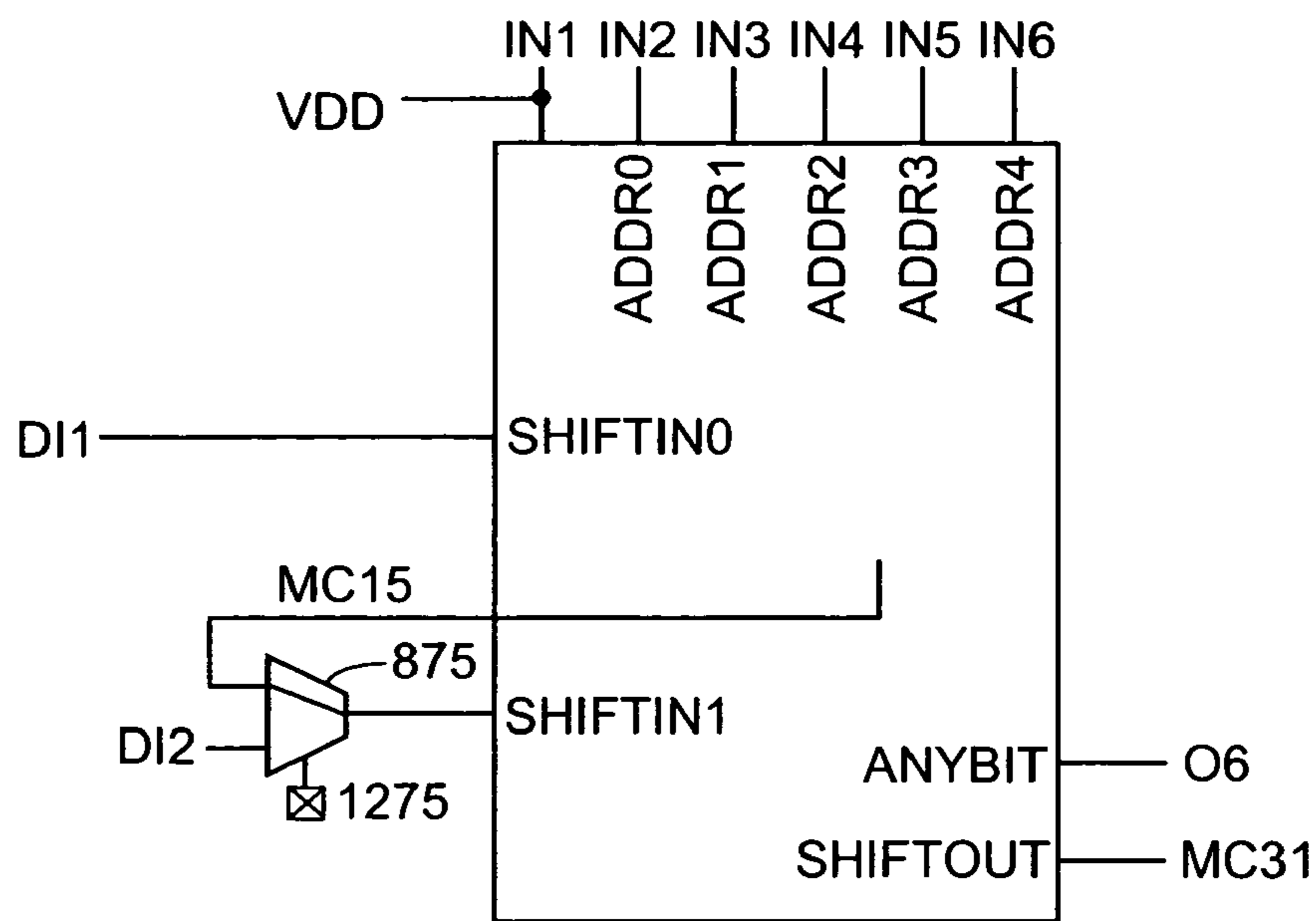
FIG. 12 (32x1 SRL)
