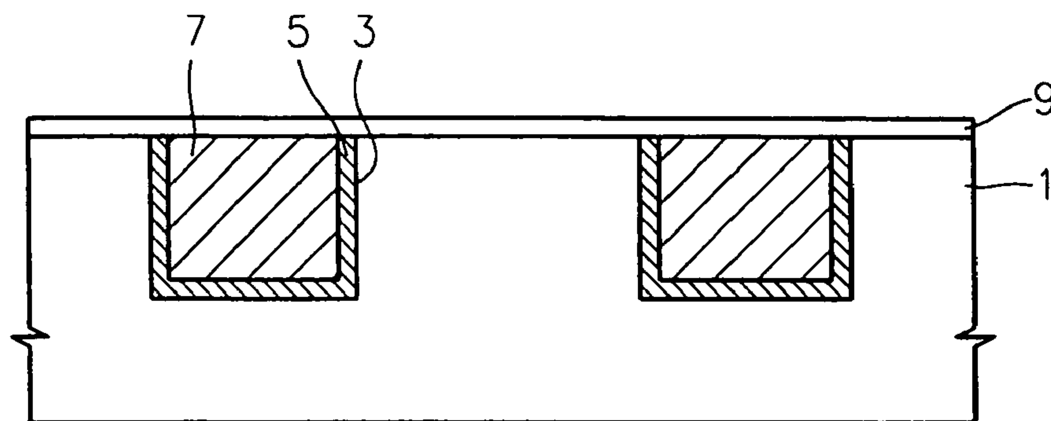
FIG. 1 (PRIOR ART)
