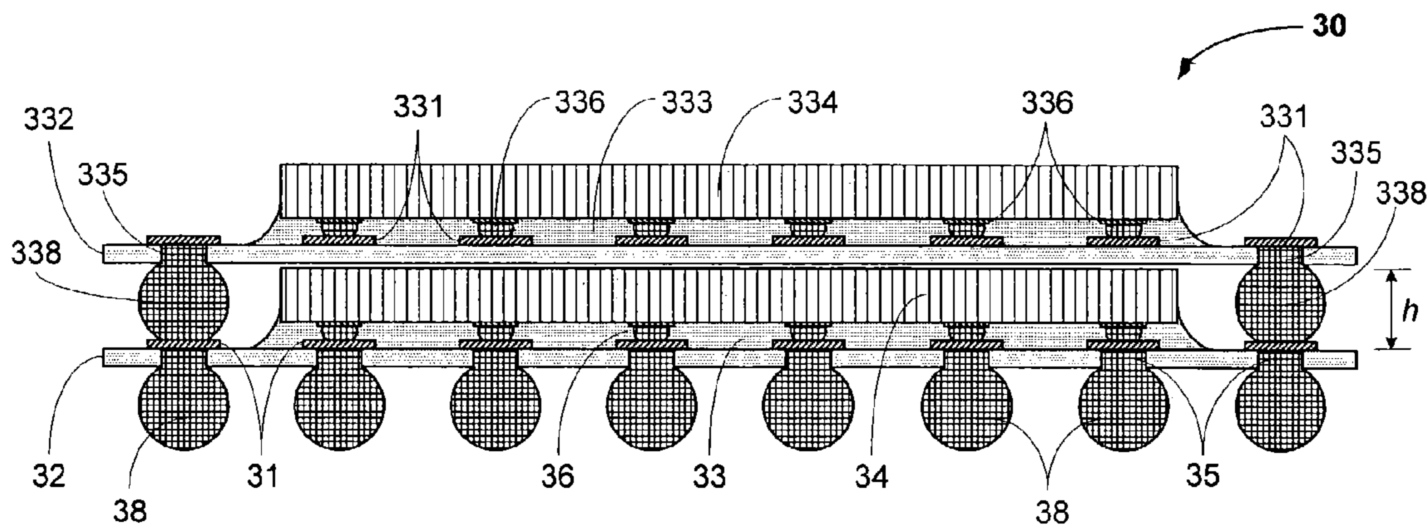
Fig. 3 PRIOR ART
