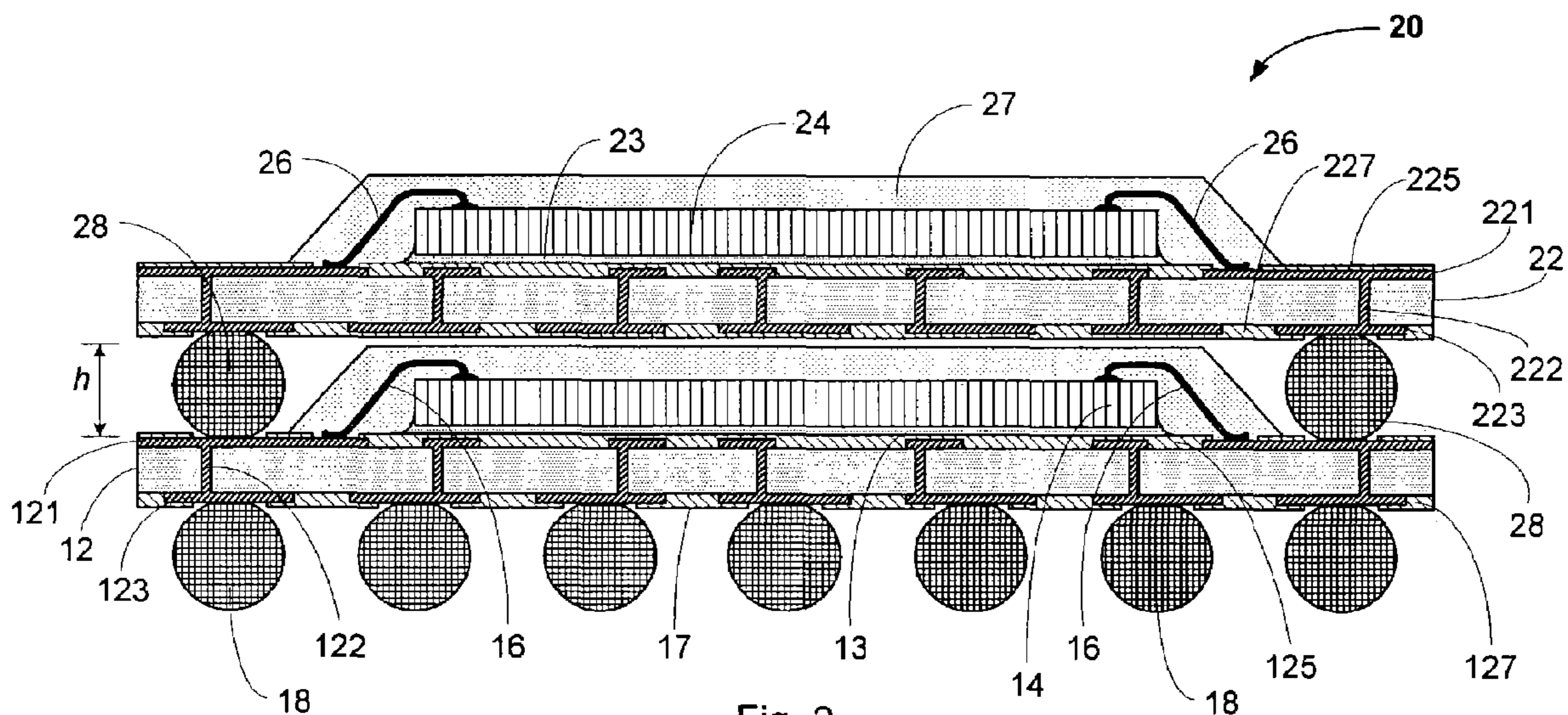
Fig. 2 PRIOR ART
