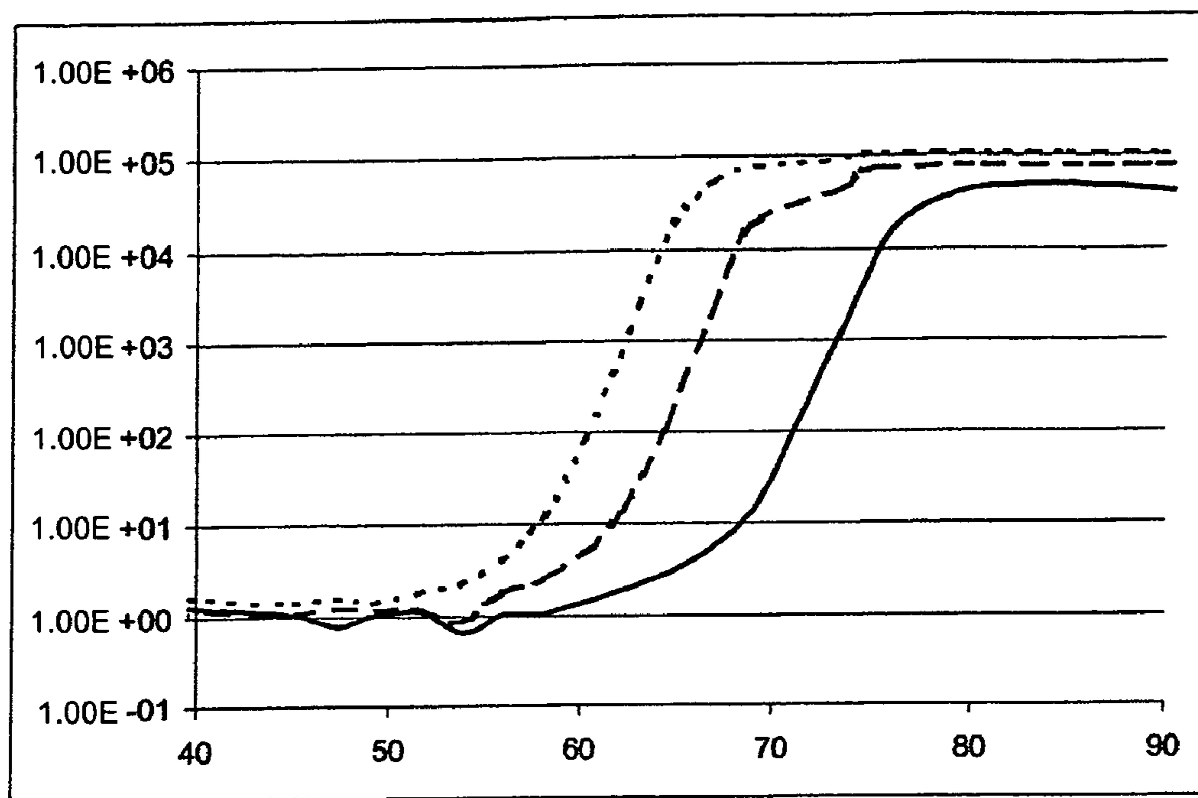
Fig 1: Gelling curves of plastisols 1-3
