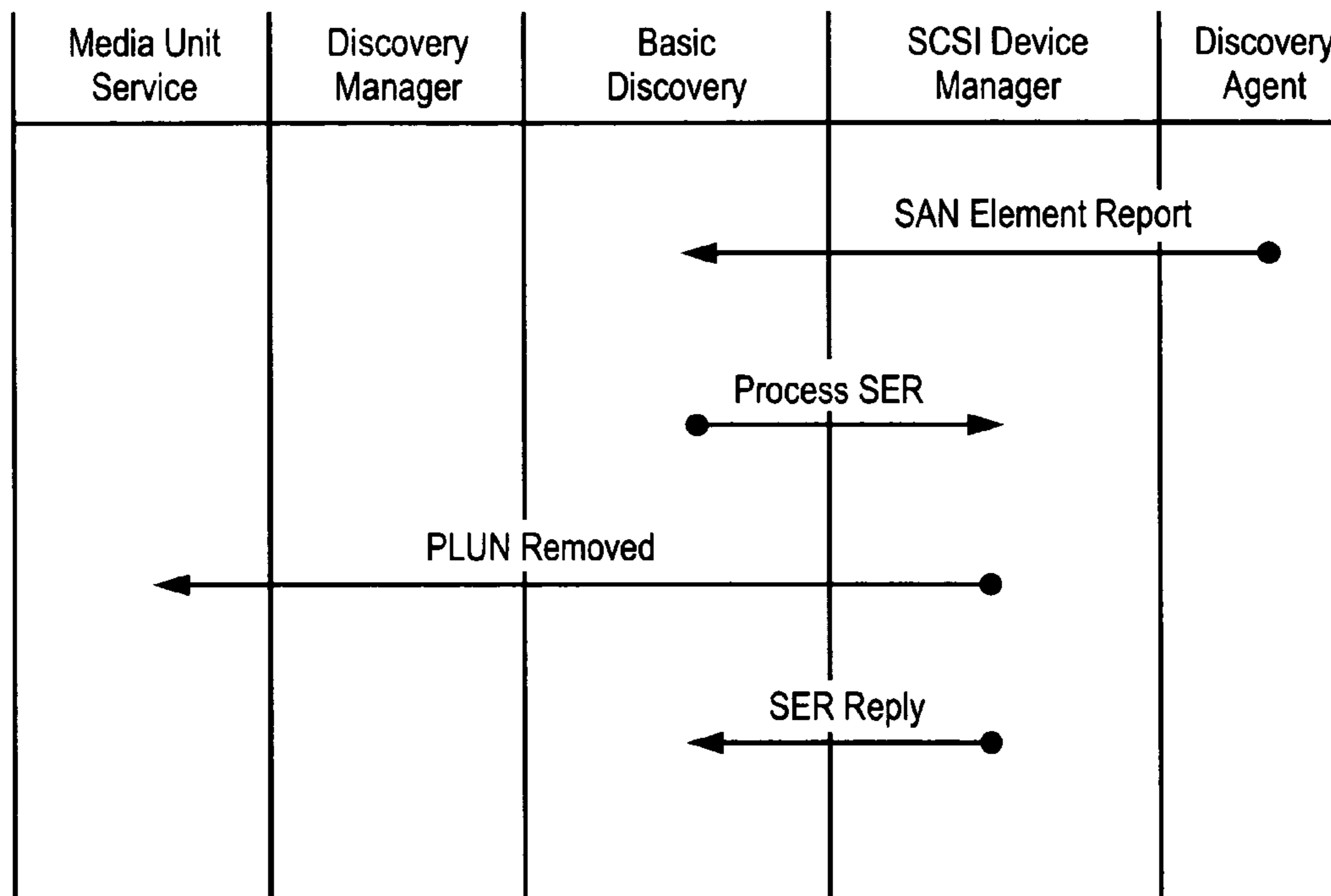
Device Removed Sequence Diagram
