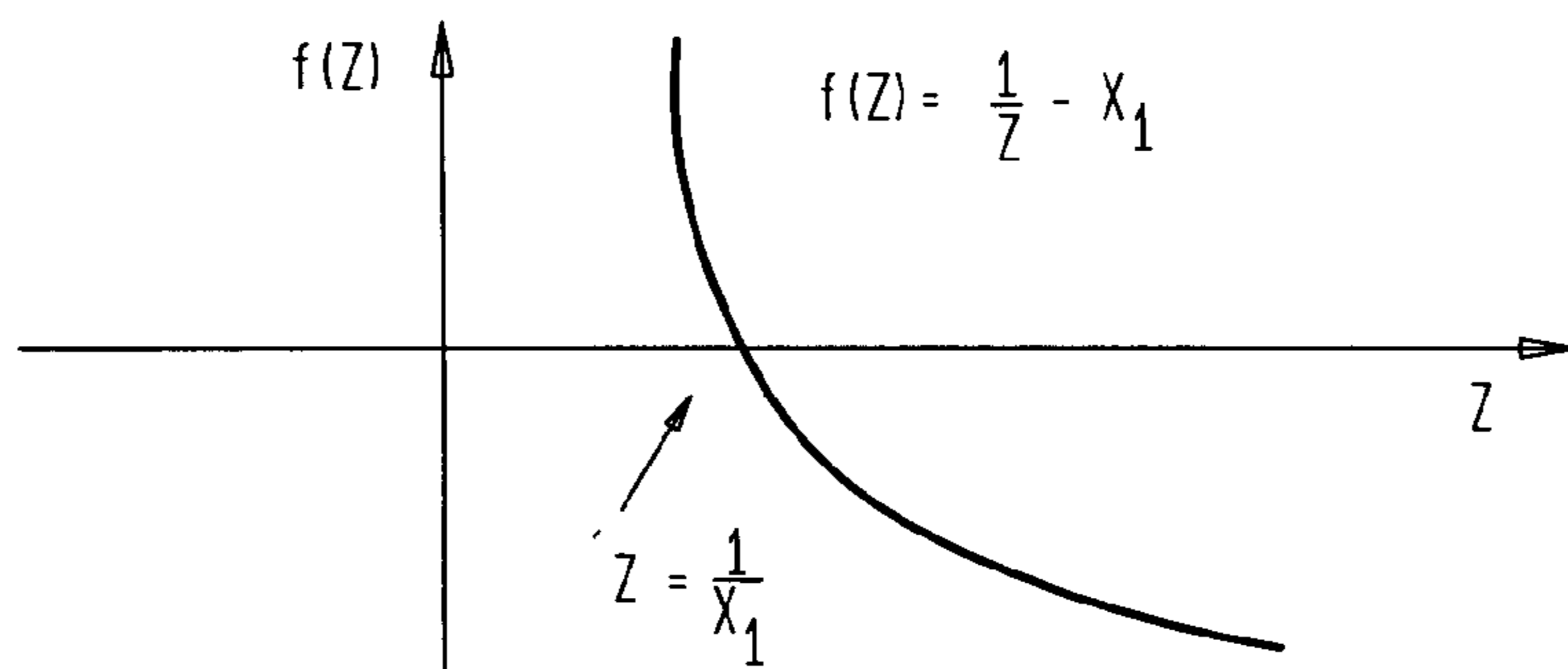
FIG. 70A USING NEWTON-RAPHSON ITERATION TO FIND 1/X_1
