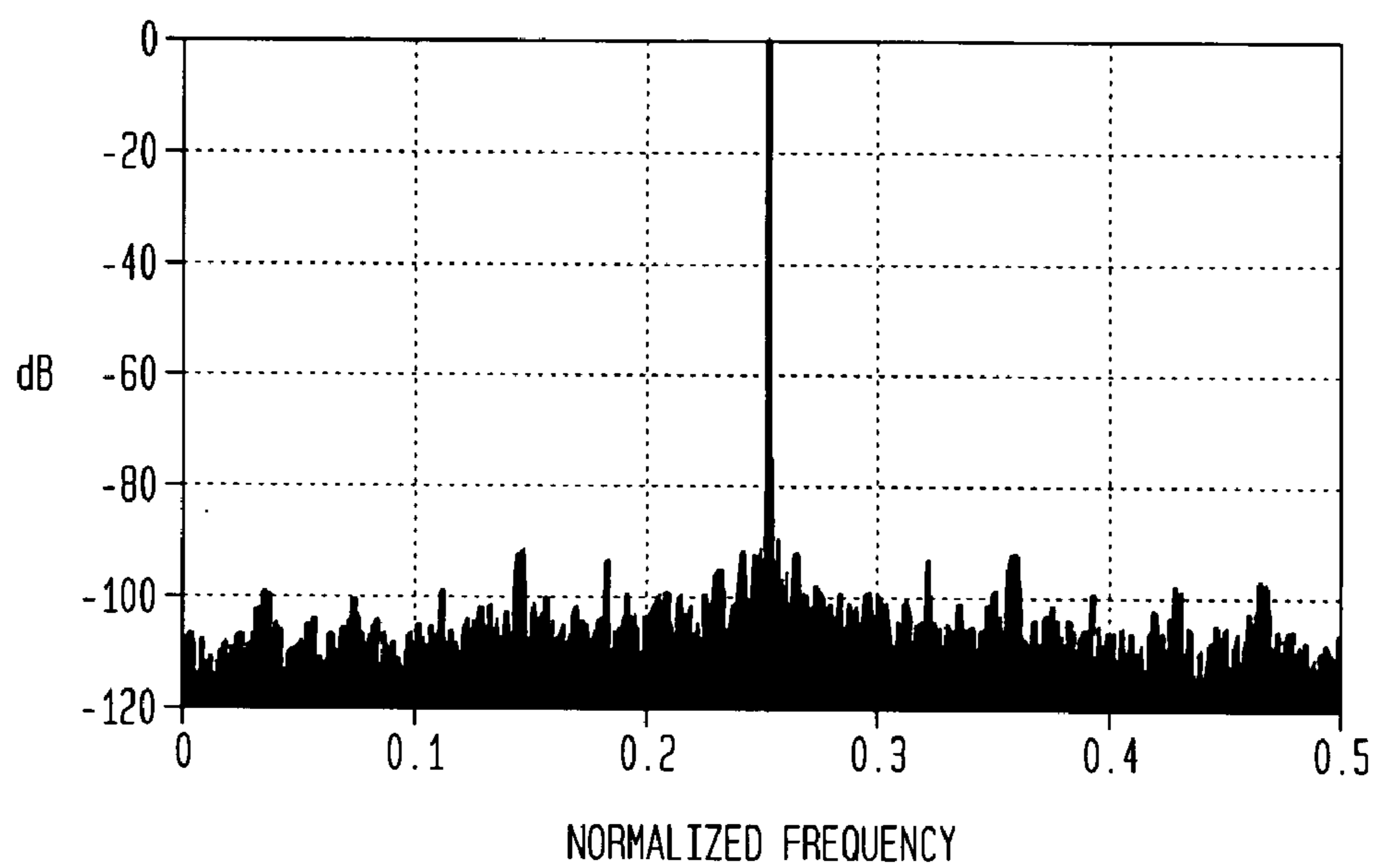
FIG. 43 OUTPUT SPECTRUM SHOWING 90.36 dB SFDR
