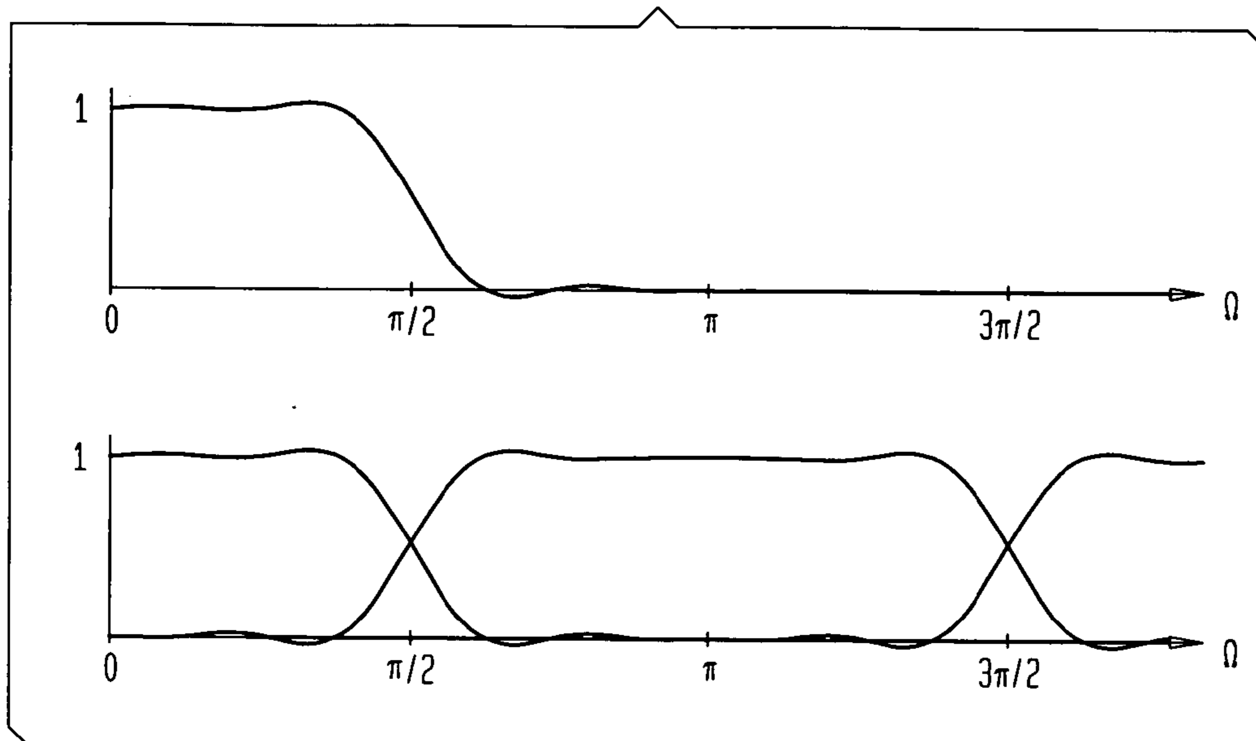
FIG. 27A FRACTIONAL-DELAY FILTER WITH \mu=0.12 , USING THE PRELIMINARY N=8 INTERPOLATOR
