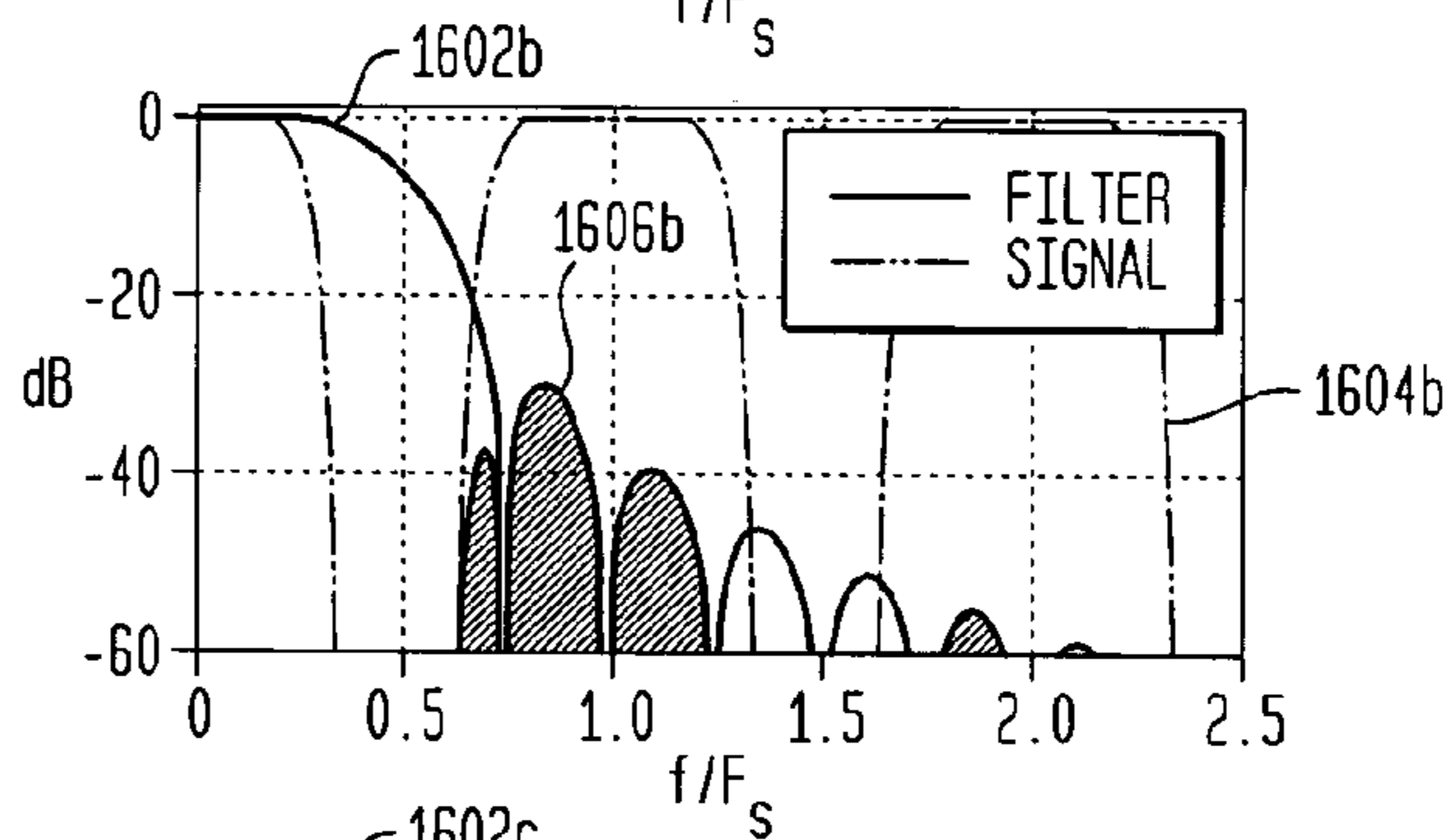
FIG. 16B TRIGONOMETRIC INTERPOLATOR 1000 (FIG. 10)
