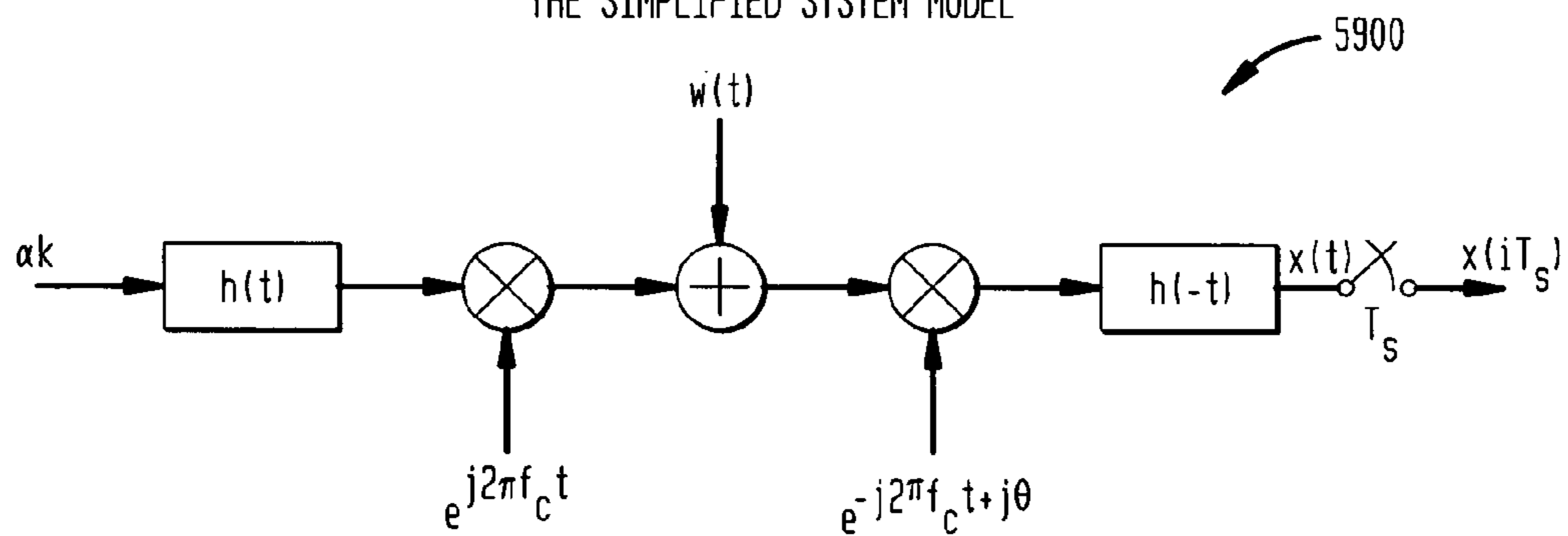
FIG. 59 THE SIMPLIFIED SYSTEM MODEL
