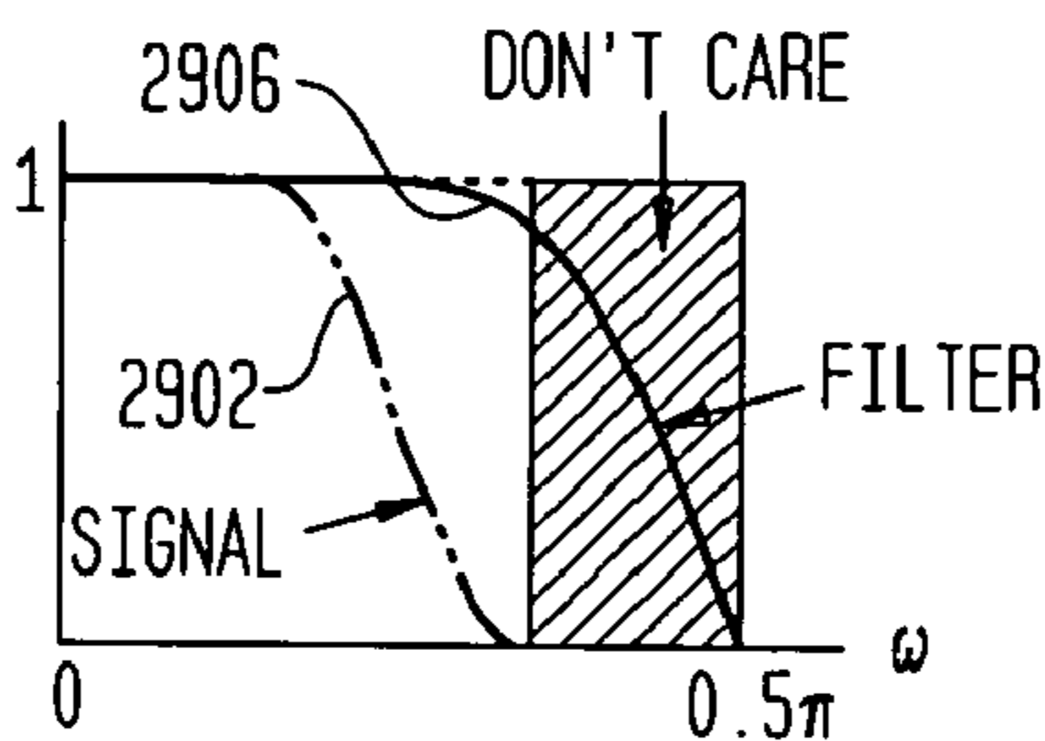
FIG. 29B F_{\mu}(\omega) , WITH \mu=0.5 , N=8 , AFTER OPTIMIZATION
