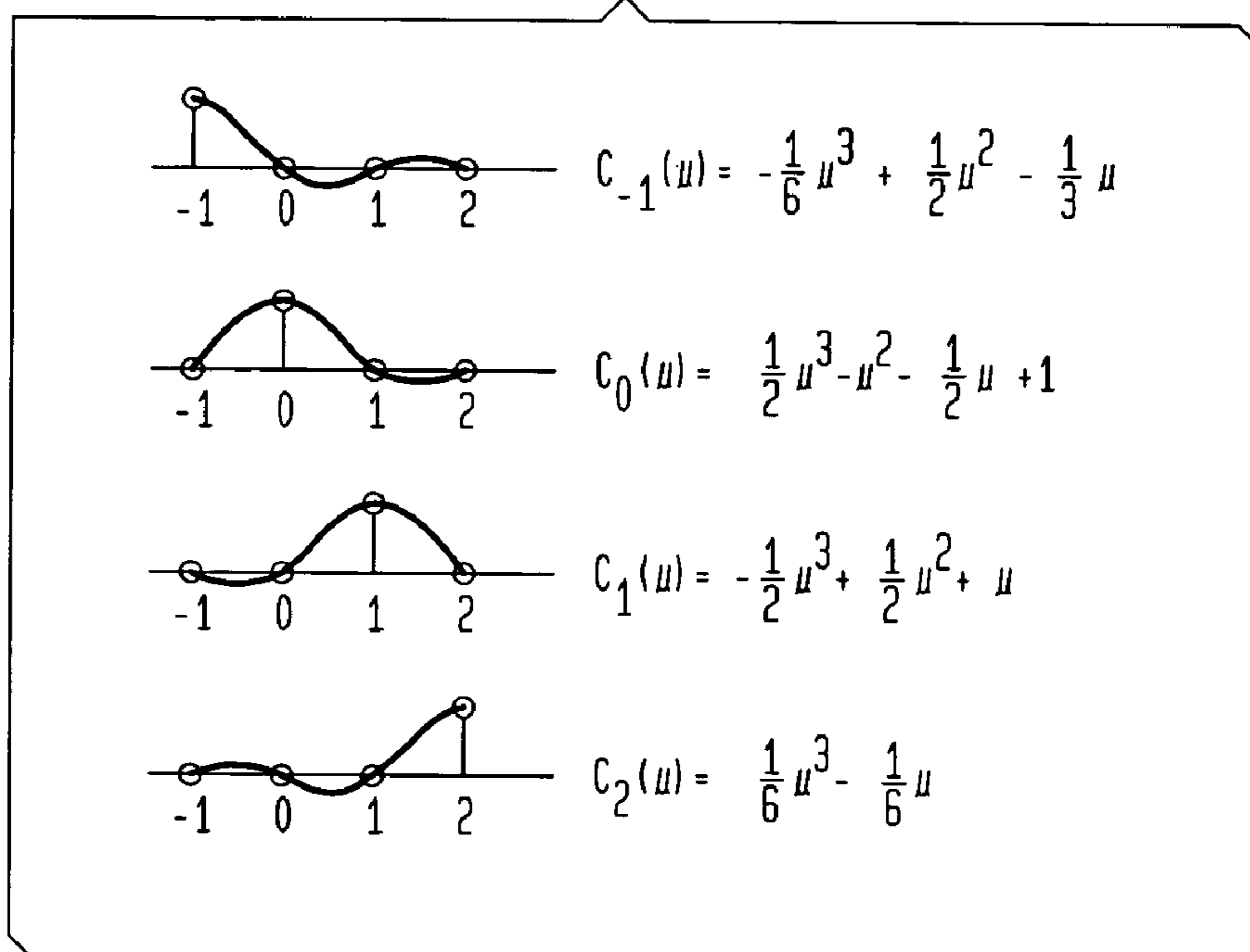
FIG. 3 THE LAGRANGE BASIS POLYNOMIALS
