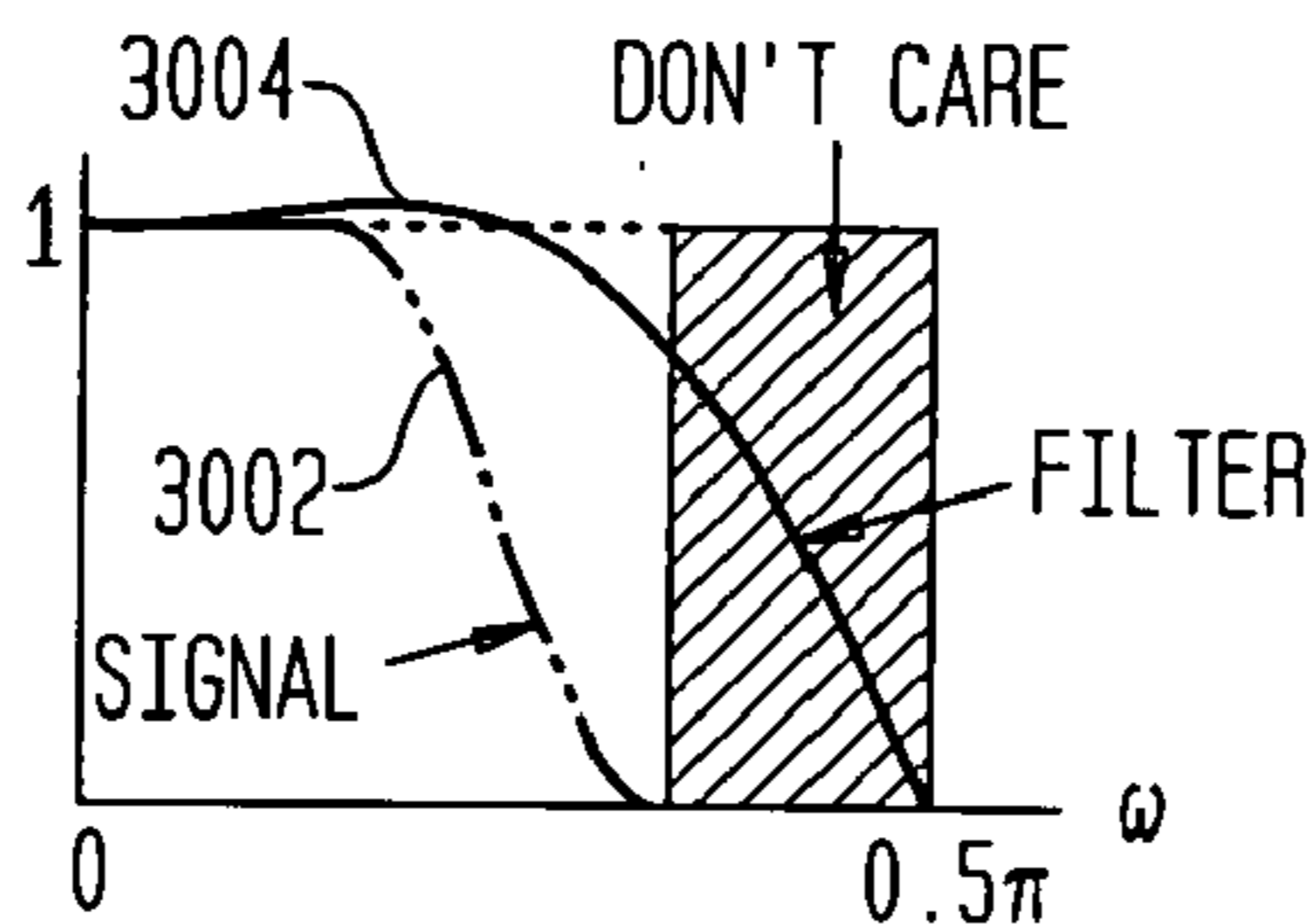
FIG. 30A F_{\mu}(\omega) , WITH \mu=0.5 , N=4 , BEFORE MODIFICATION
