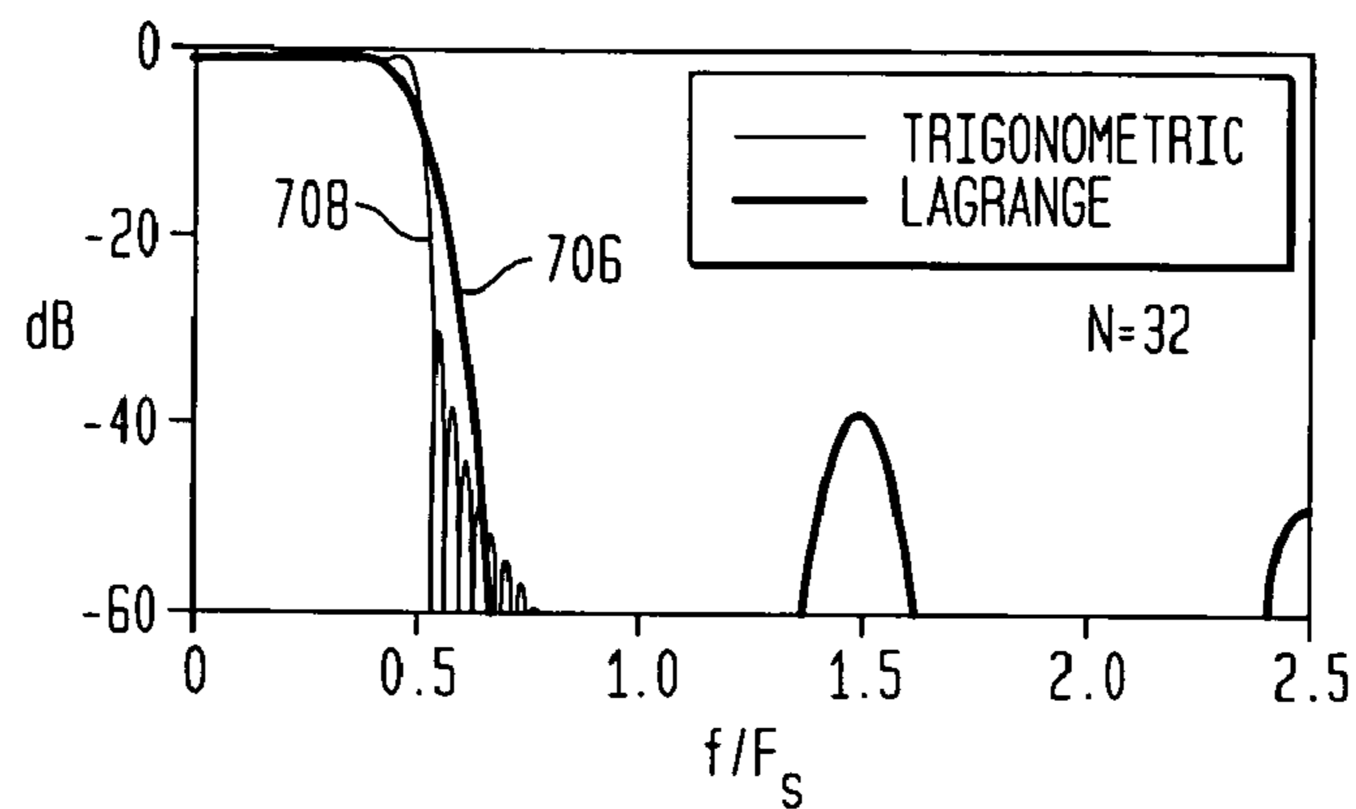
FIG. 7B FREQUENCY RESPONSES FOR N=32
