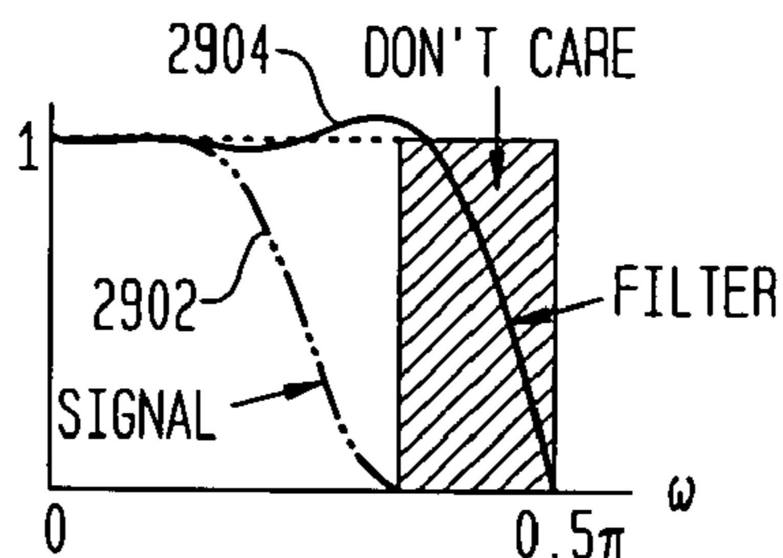
FIG. 29A F_{\mu}(\omega) , WITH \mu=0.5 , N=8 , BEFORE OPTIMIZATION
