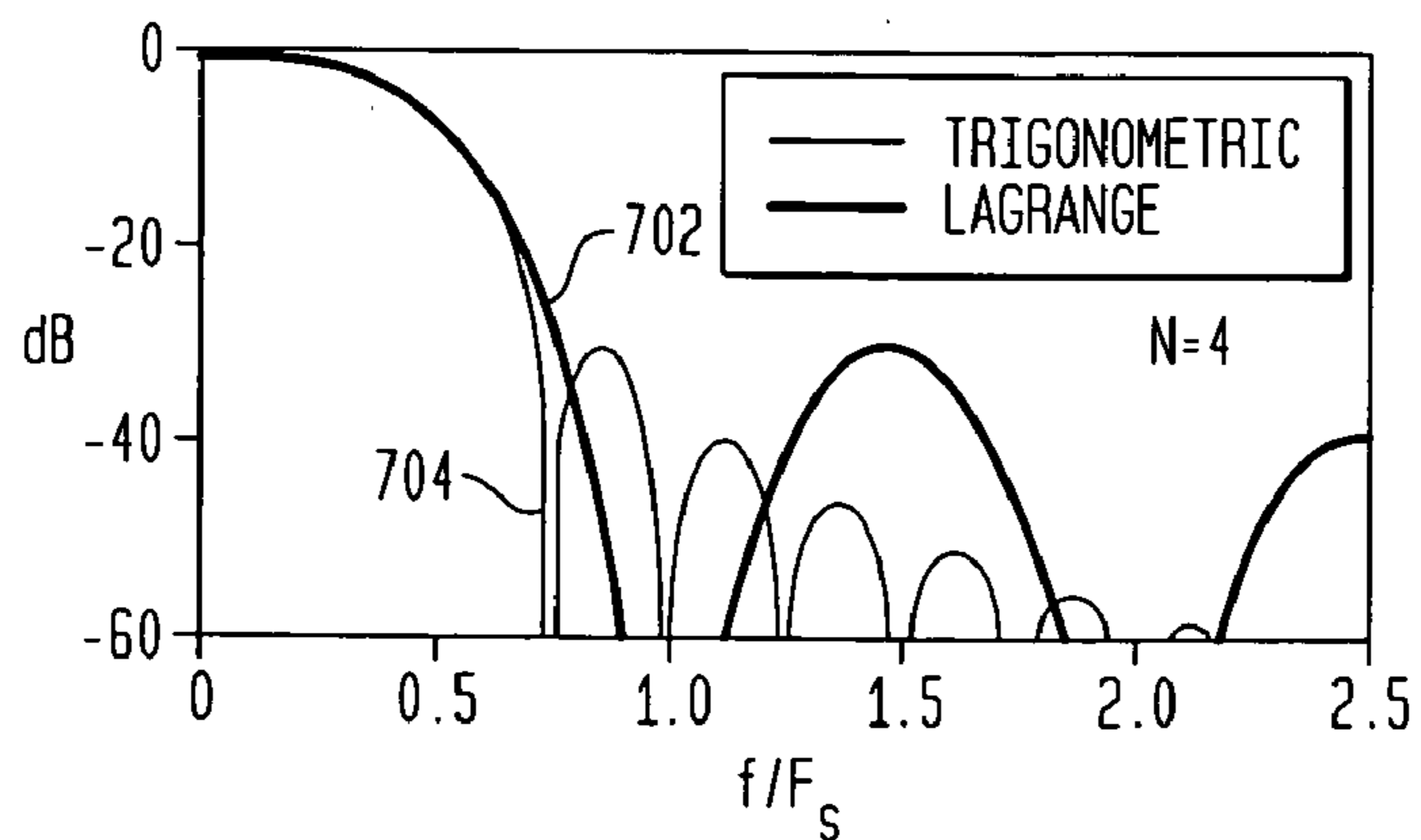
FIG. 7A FREQUENCY RESPONSES FOR N=4
