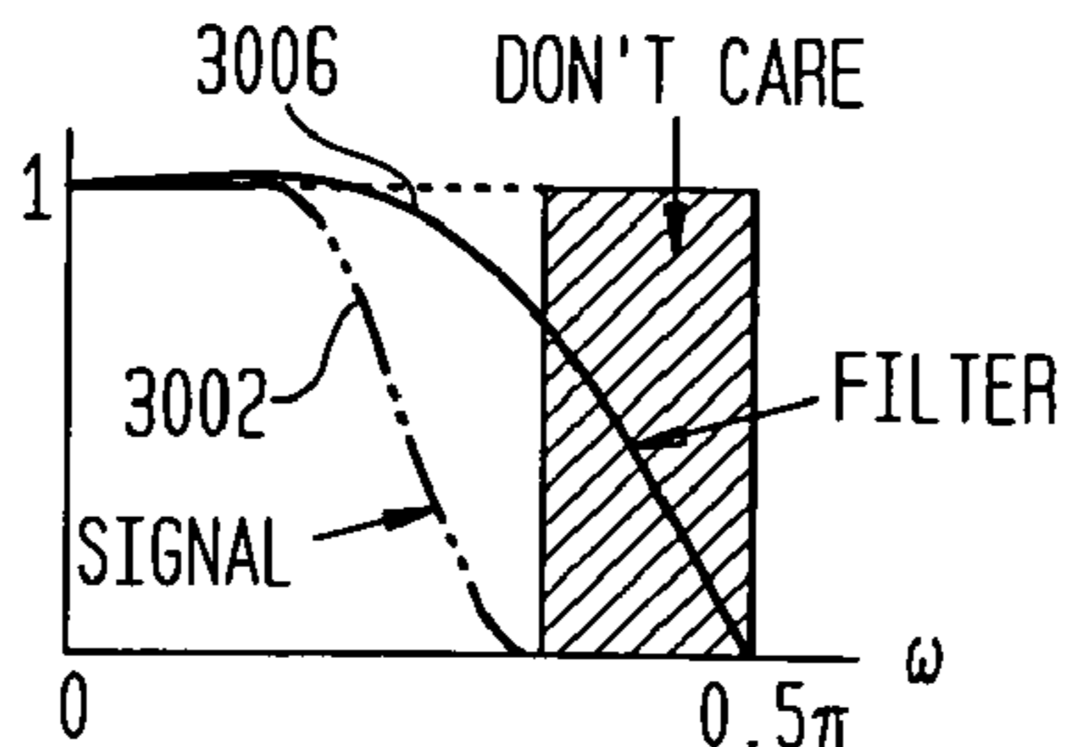
FIG. 30B F_{\mu}(\omega) , WITH \mu=0.5 , N=4 , AFTER MODIFICATION
