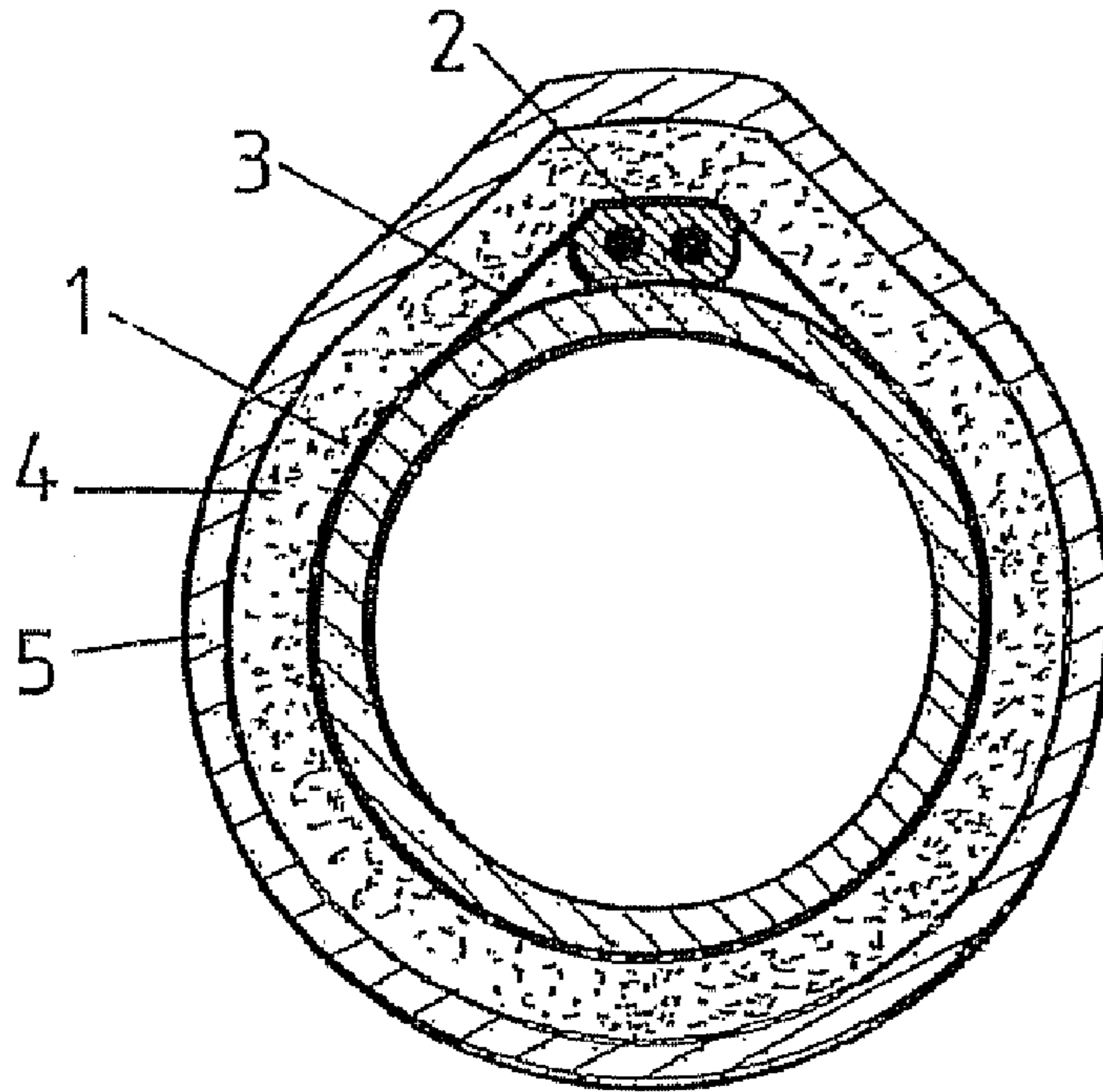
FIG. 1 (PRIOR ART)
