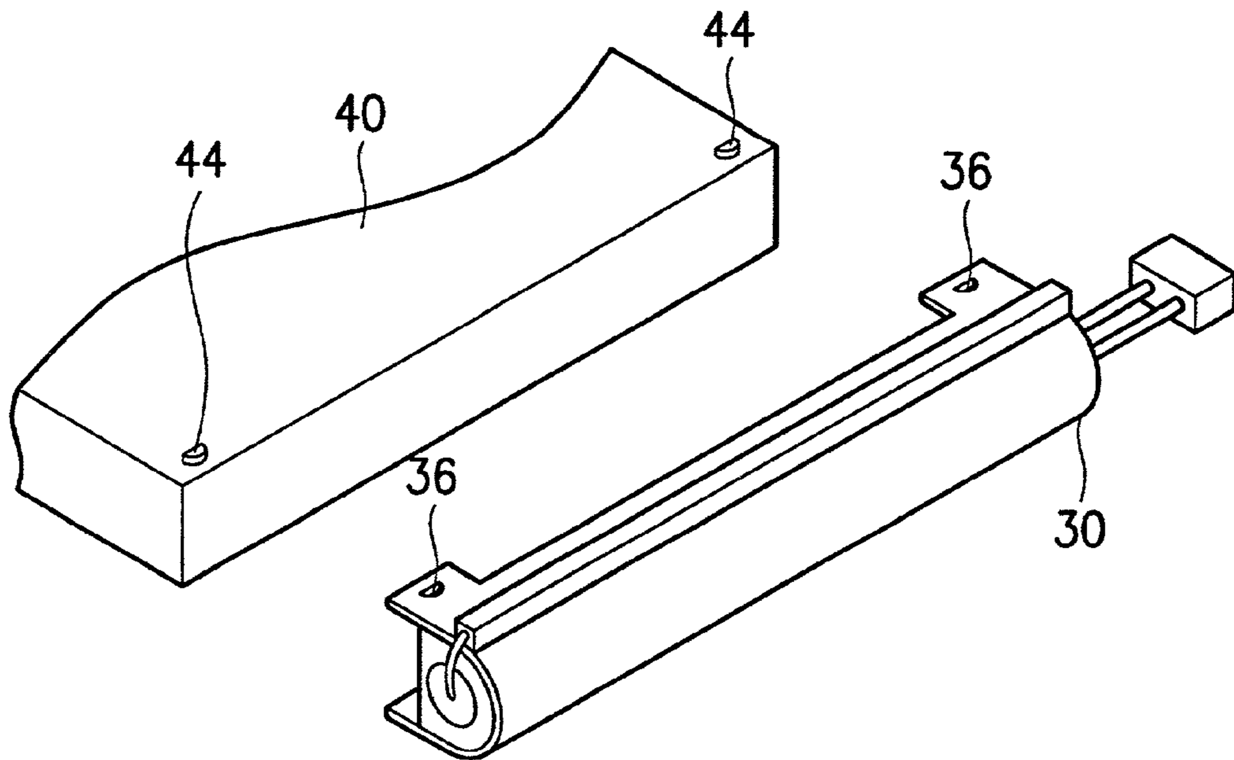
FIG. 2 ( PRIOR ART )
