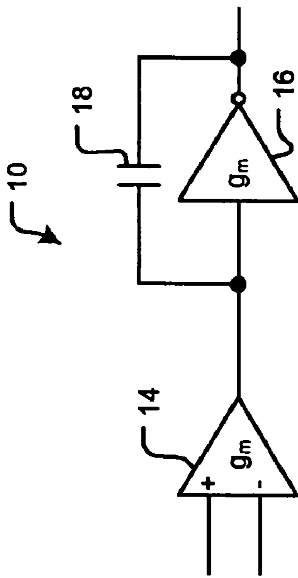
FIG. 1 Prior Art
