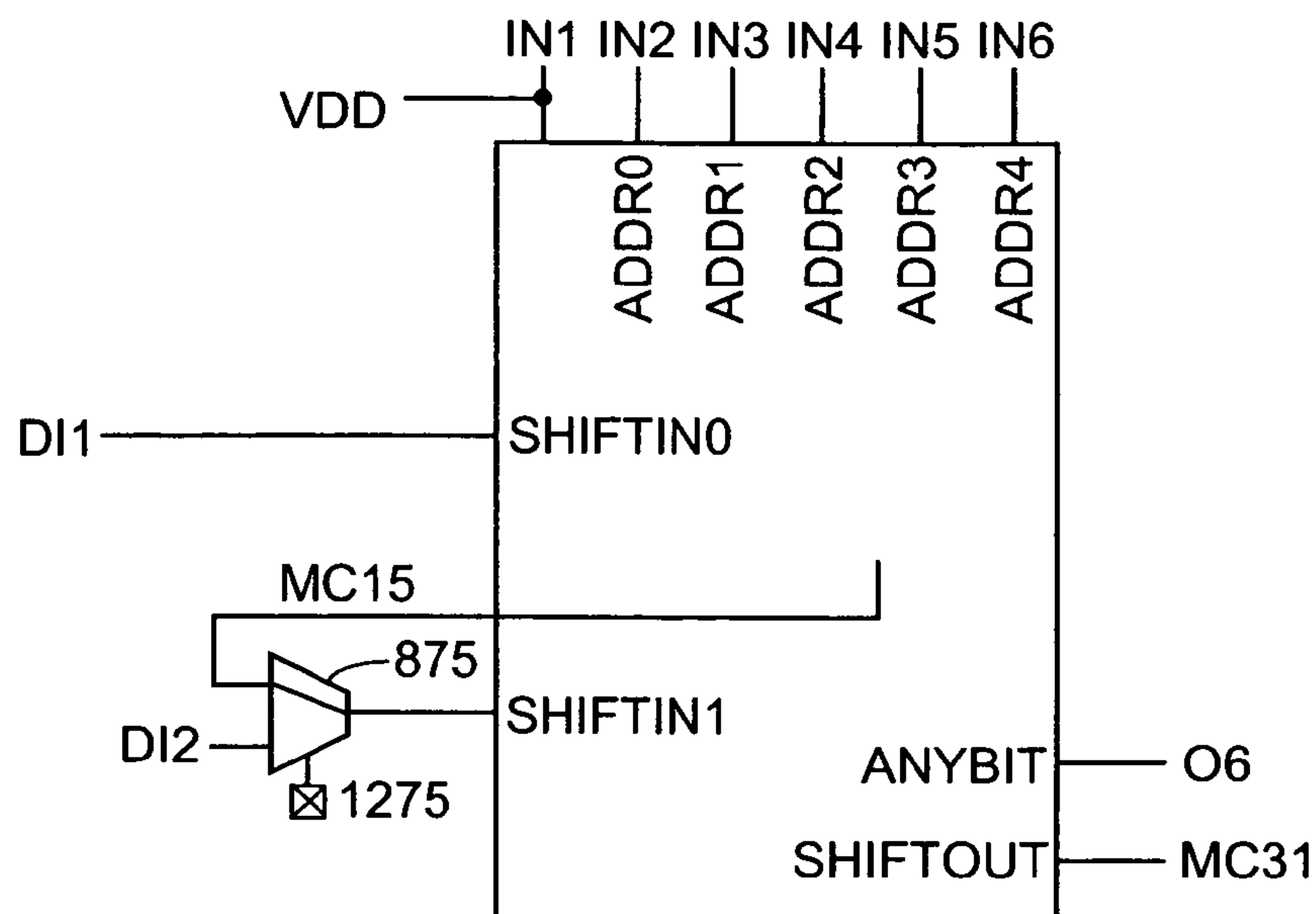
FIG. 12 (32x1 SRL)
