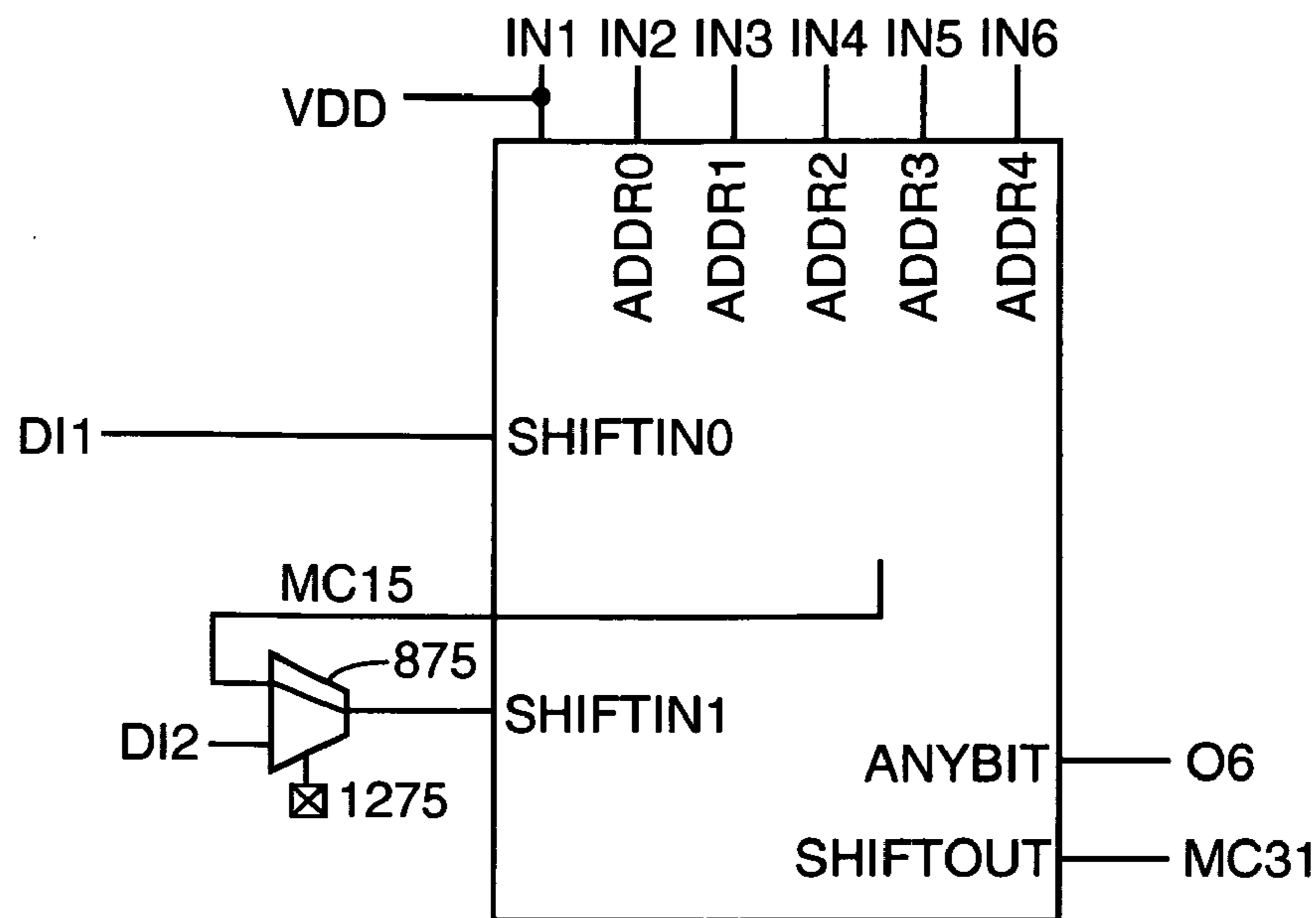
FIG. 12 (32x1 SRL)
