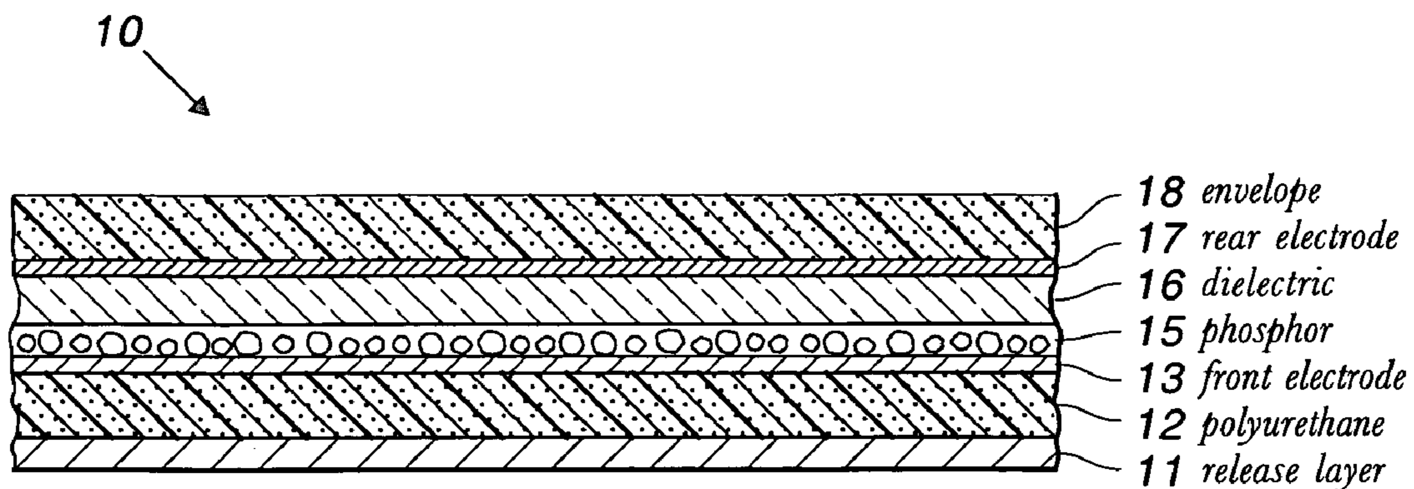
FIG. 1 (PRIOR ART)
