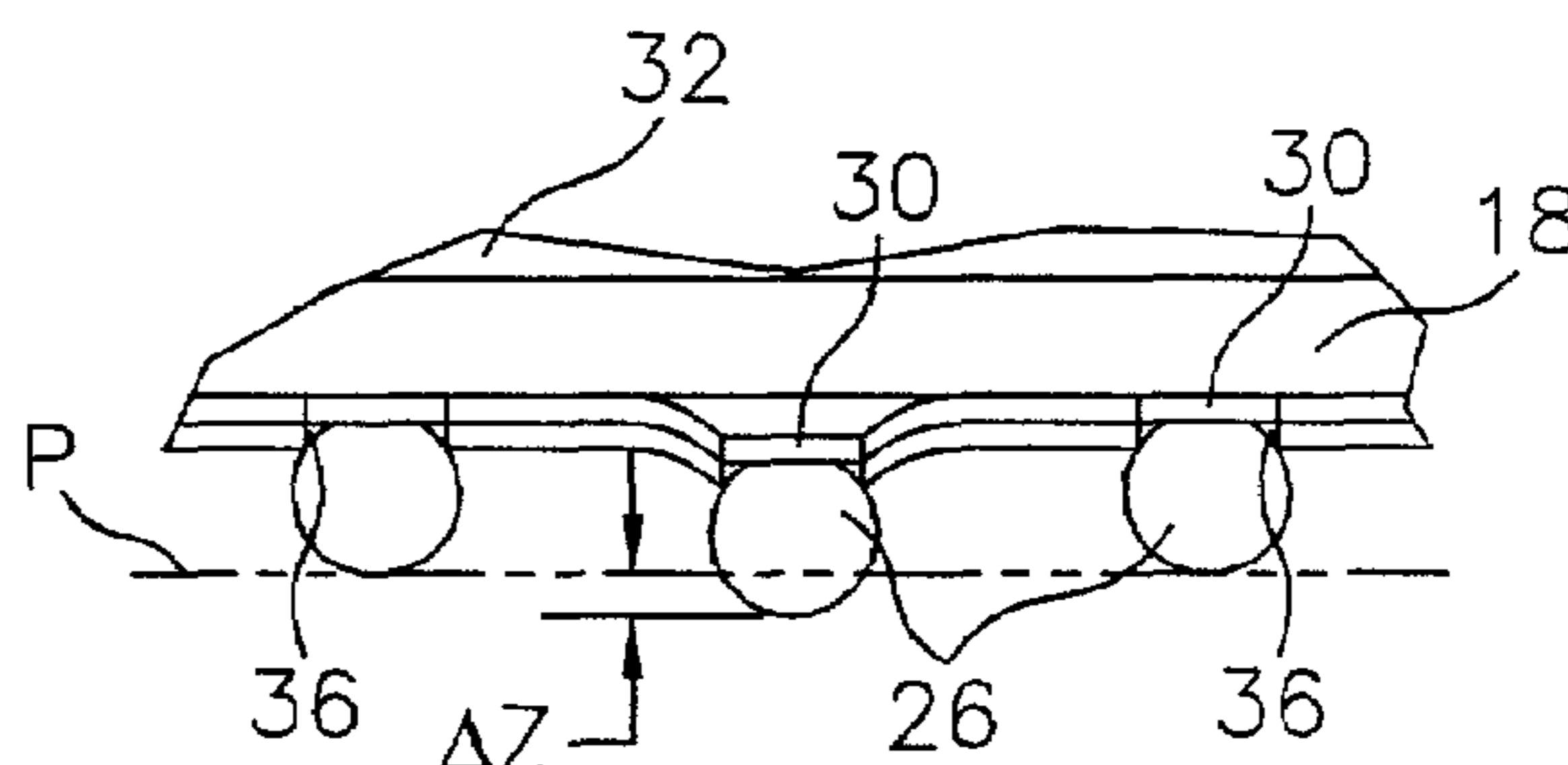
FIGURE 1C (PRIOR ART)
