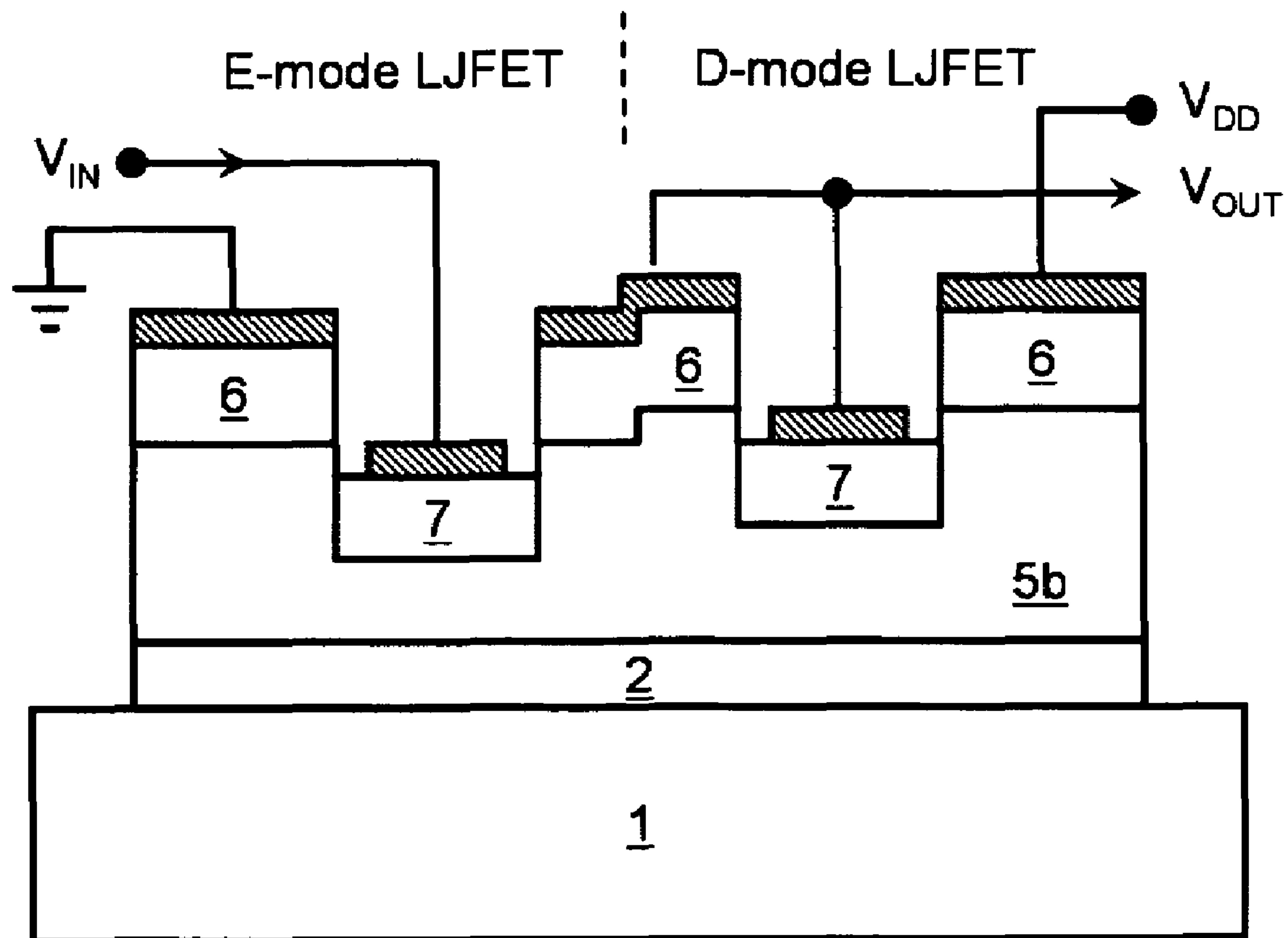
Lateral channel JFET IC chip
