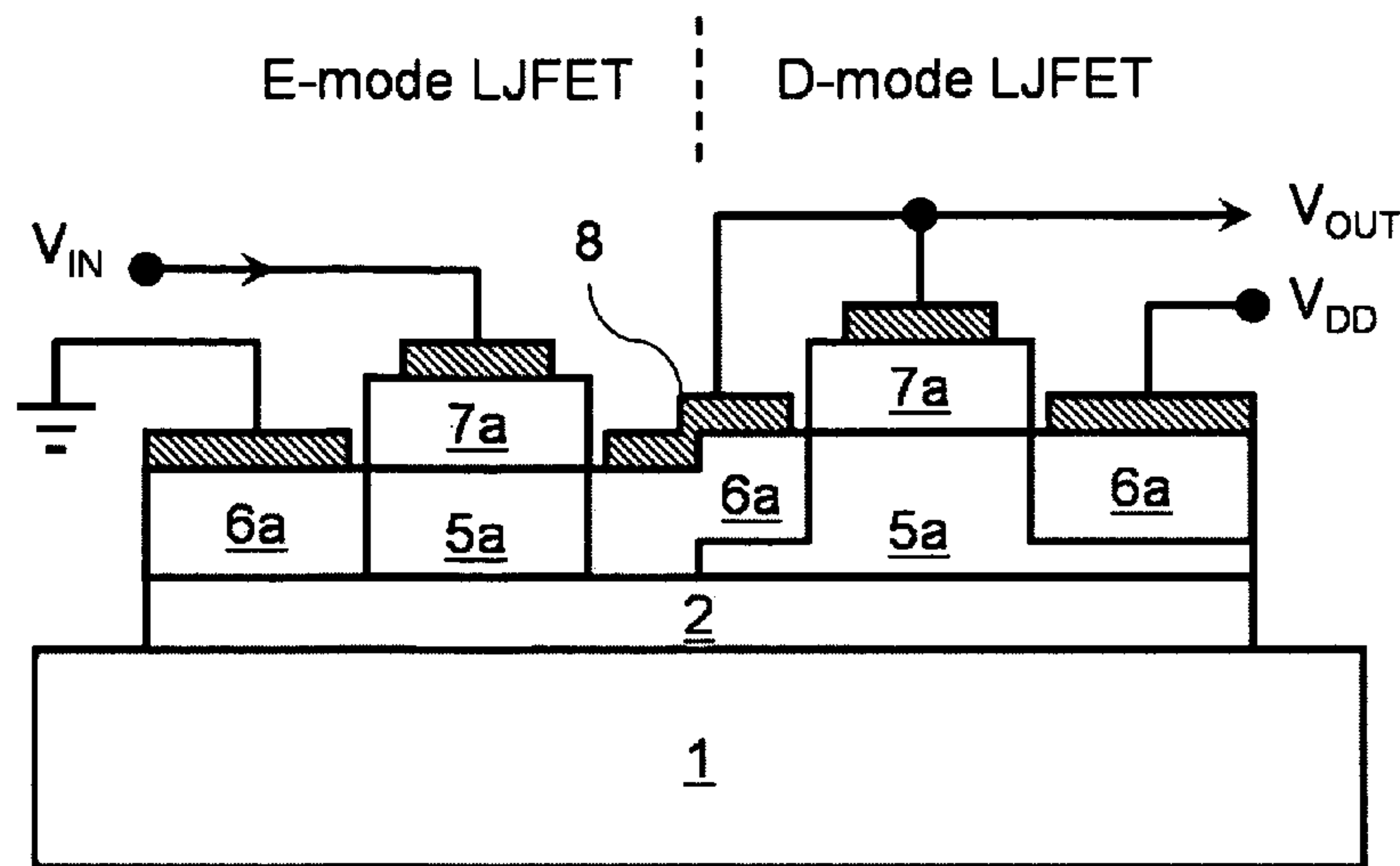
Lateral channel JFET IC chip
