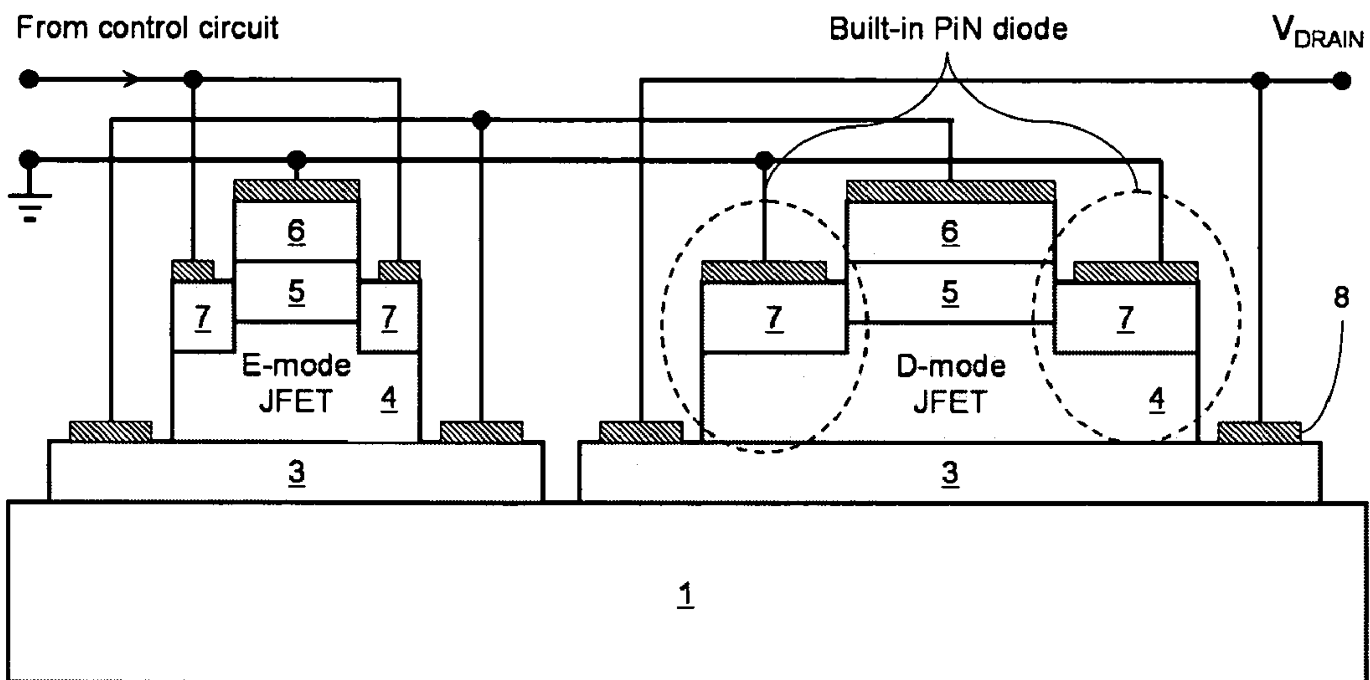
Vertical channel JFET IC chip
